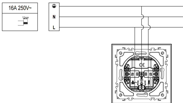
① Wiring diagram for grounding socket
