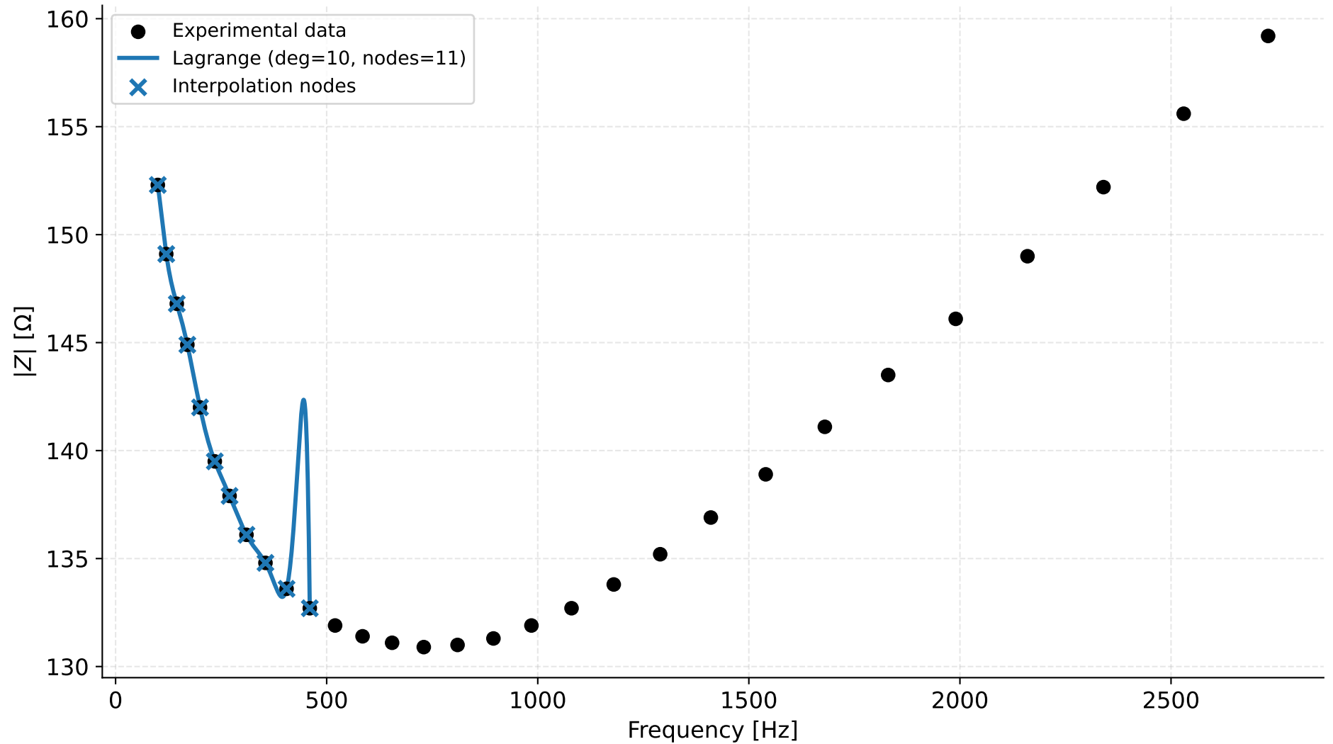
Global Lagrange Interpolation
