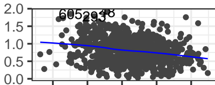
Scale-Location
