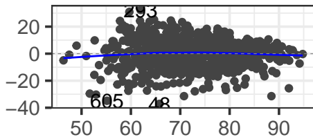
Residuals vs Fitted
