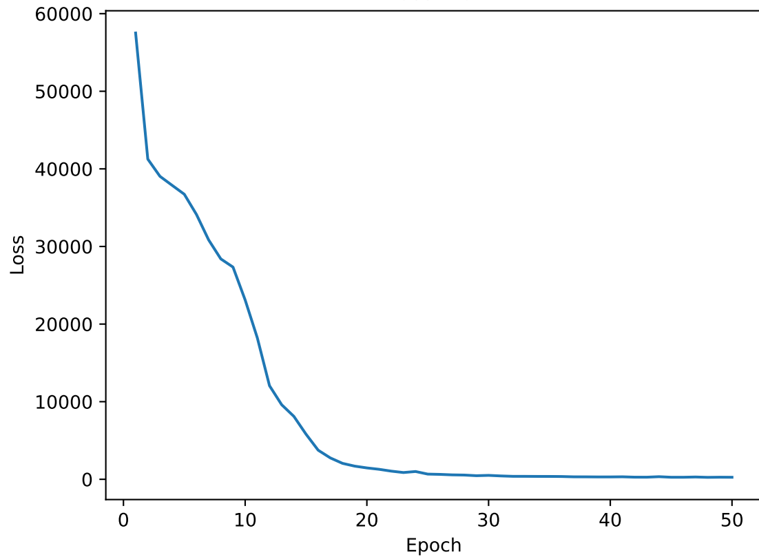
Loss Plot
