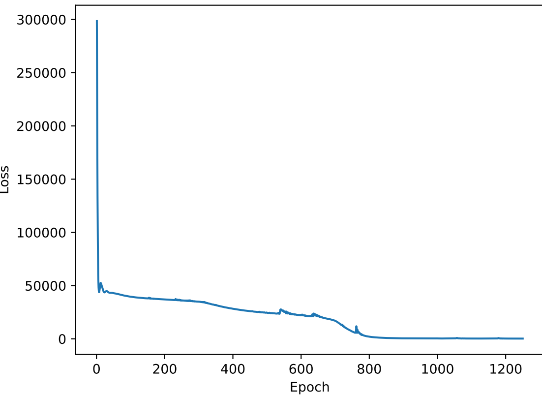
Loss Plot
