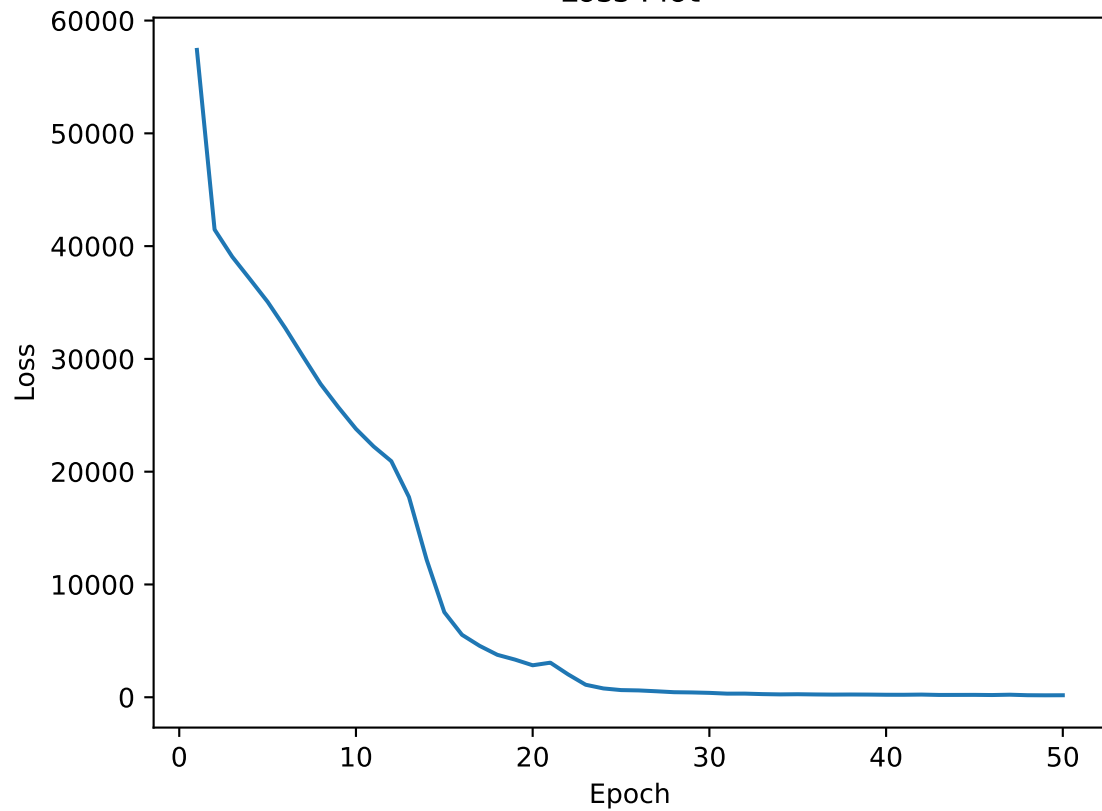
Loss Plot
