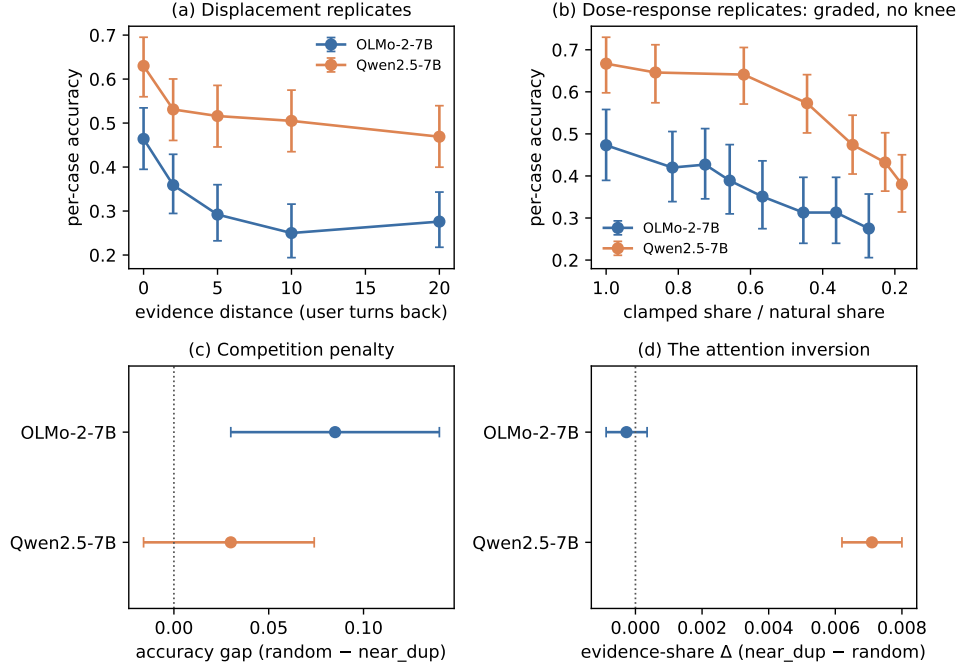
Figure 8: The causal program replicates on Qwen2.5-7B, except competition. (a) The distance ladder at matched fill ( n=192 /arm in both families). (b) The share \rightarrow accuracy dose-response, x as a fraction of each family’s natural share (OLMo layer-24-indexed with common subset n=131 , Qwen all-layer with n=181-192 ): graded with no knee in both. (c) The competition contrast is significant on OLMo, not detected on Qwen. (d) The evidence’s attention under near-duplicate context: flat on OLMo, rising on Qwen, with disjoint intervals—the family divergence. Whiskers in (a, b) are per-point Wilson 95% intervals. Panels (c, d) show the paired bootstrap CIs quoted in the text.
