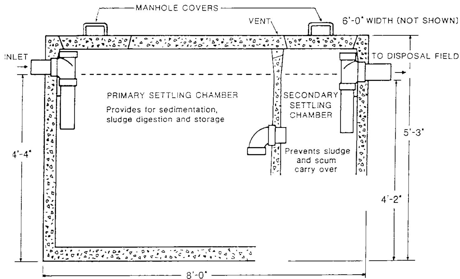
TYPICAL CONCRETE 1000 GALLON SEPTIC TANK (3 BEDROOM DWELLING)
