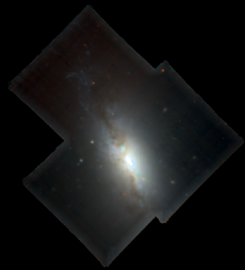
NGC4383
