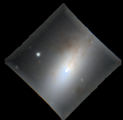
NGC4694
