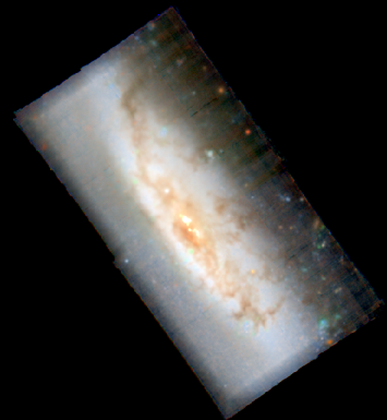
NGC4522
