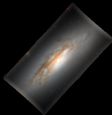
NGC4419
