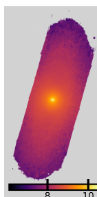
NGC4698: \log \Sigma_*
