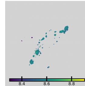
[O/H] (O3N2-M13, HII)
