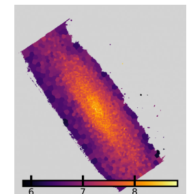
NGC4694: \log \Sigma_*
