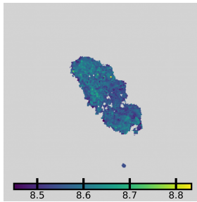
[O/H] (O3N2-M13, HII)
