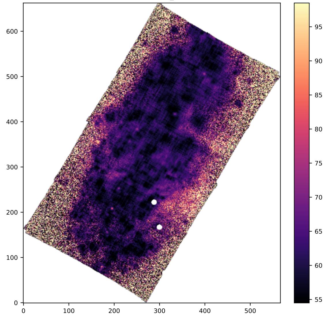
SPAXELS HA6562_SIGMA
