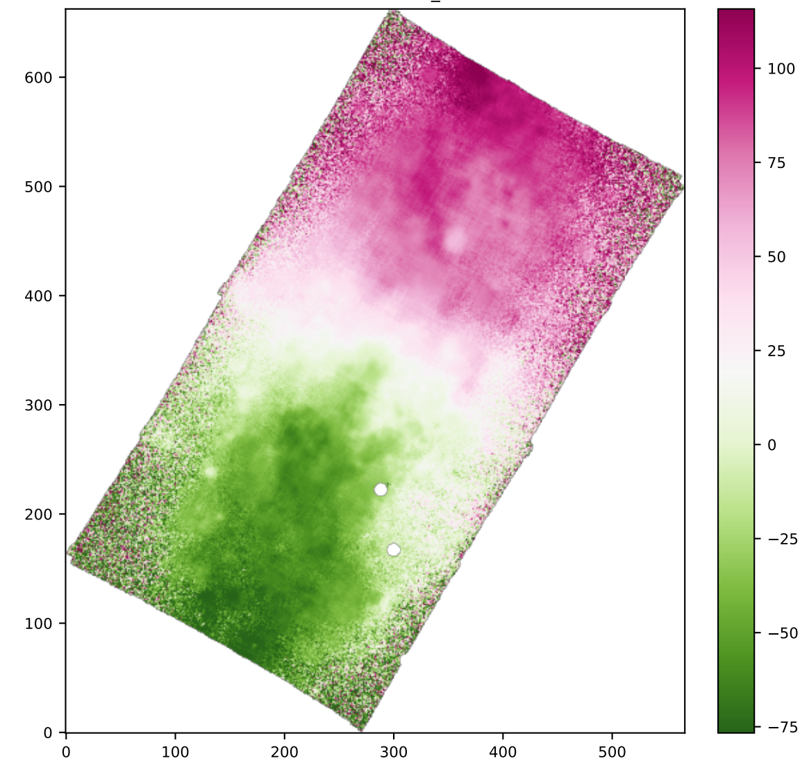
SPAXELS HA6562_VEL
