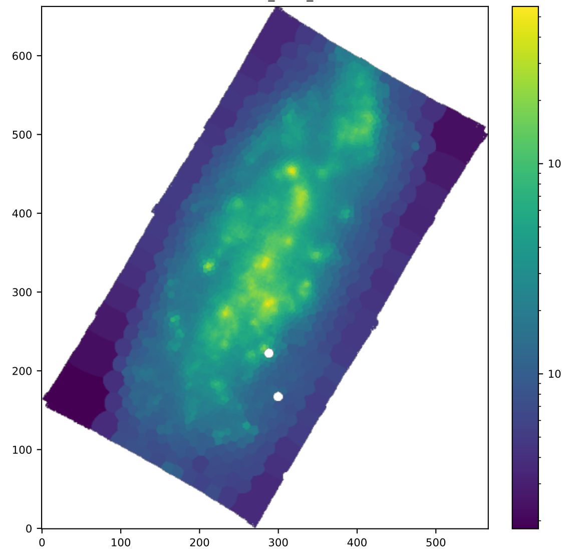
BIN HB4861_SIGMA_ERR
