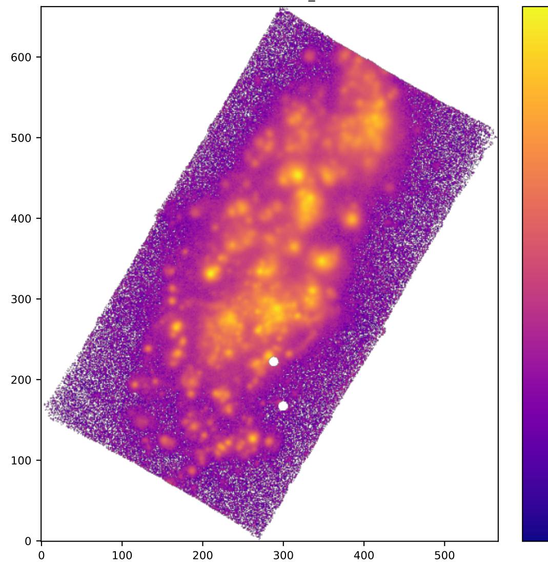
SPAXELS OIII5006_SIGMA
