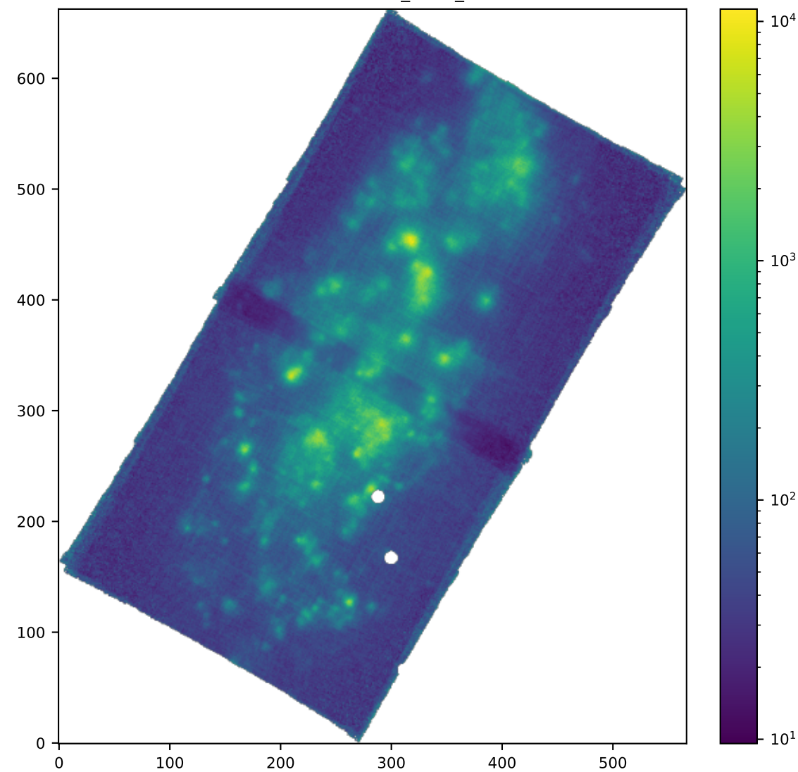
SPAXELS HA6562_SIGMA_ERR
