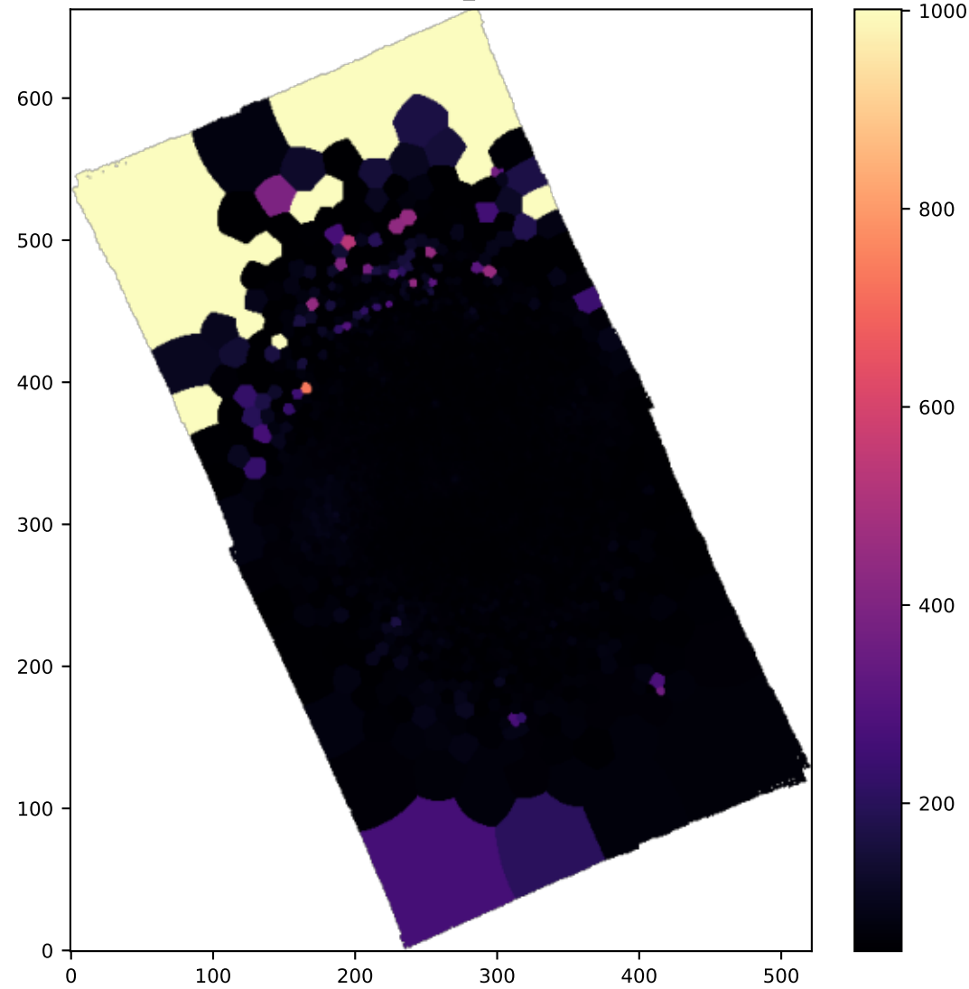
BIN OI6300_SIGMA
