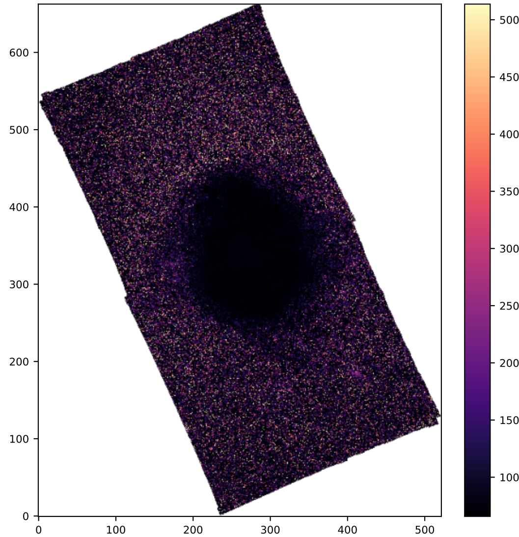
SPAXELS HB4861_SIGMA
