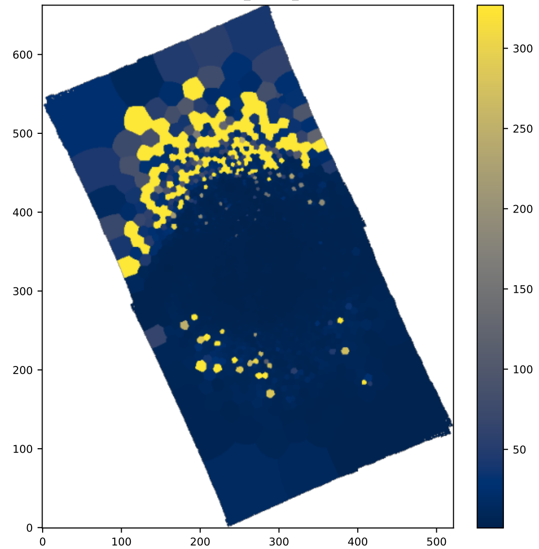
BIN OI6363_SIGMA_ERR
