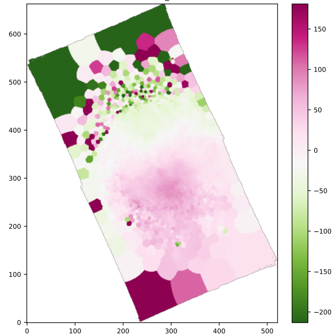
BIN OI6300_VEL
