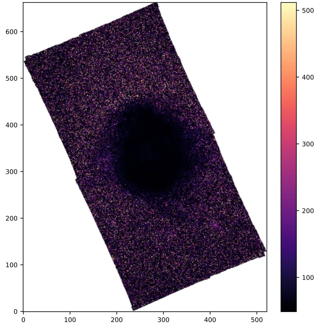
SPAXELS HA6562_SIGMA
