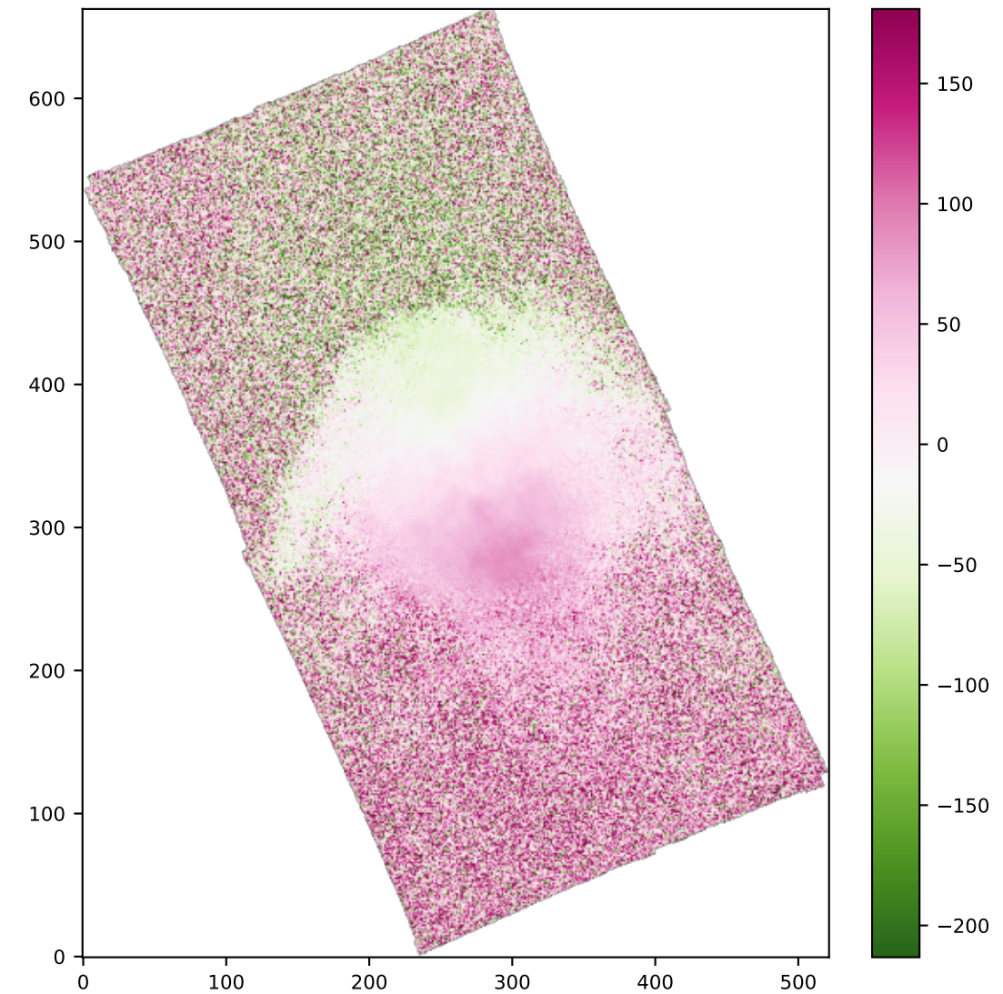
SPAXELS OI6300_VEL
