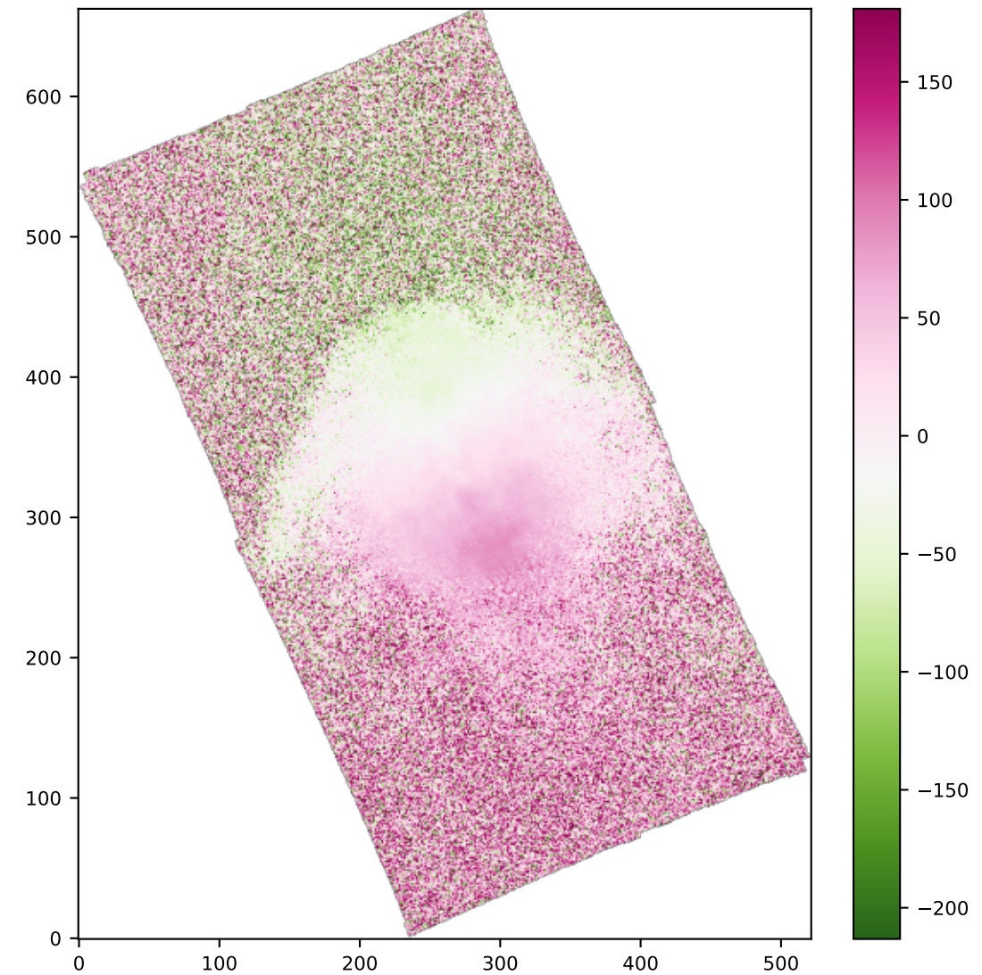
SPAXELS NII6583_VEL
