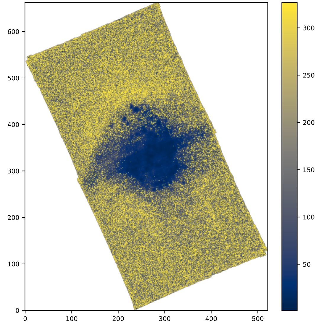
SPAXELS OI6300_SIGMA_ERR
