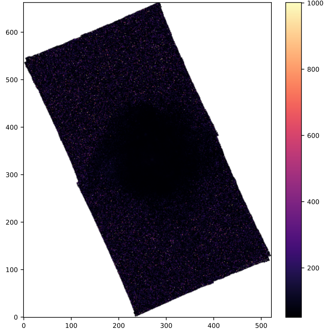
SPAXELS OI6300_SIGMA
