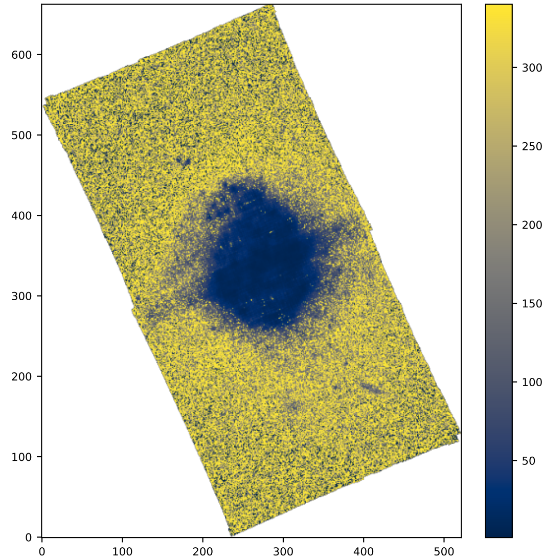
SPAXELS HB4861_SIGMA_ERR
