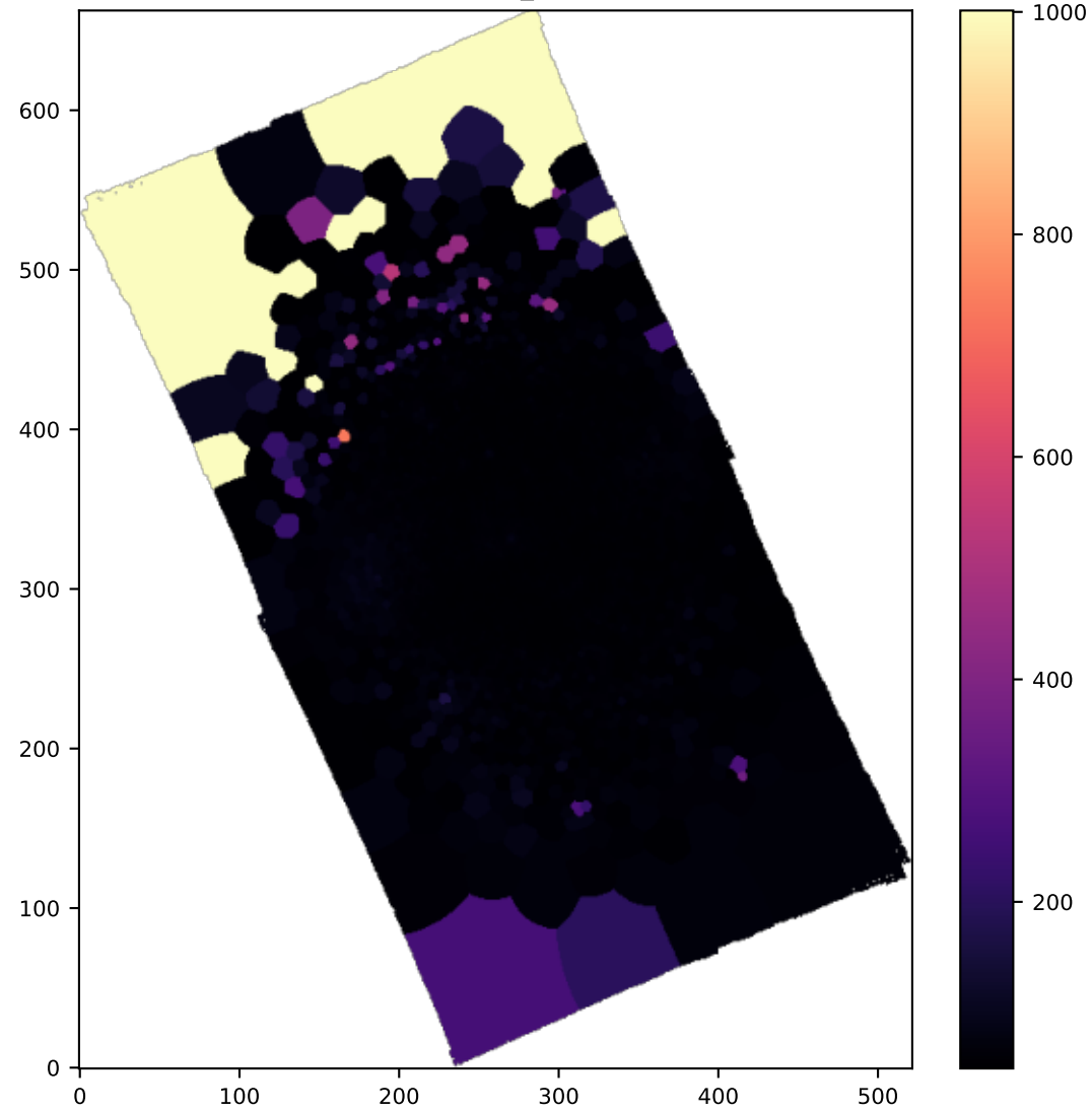
BIN OI6363_SIGMA
