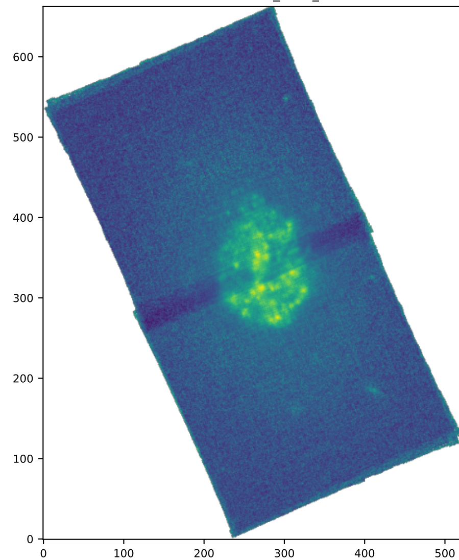
SPAXELS HA6562_SIGMA_ERR
