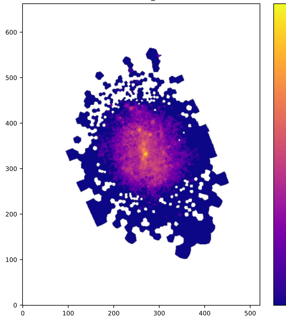
BIN OI6363_SIGMA
