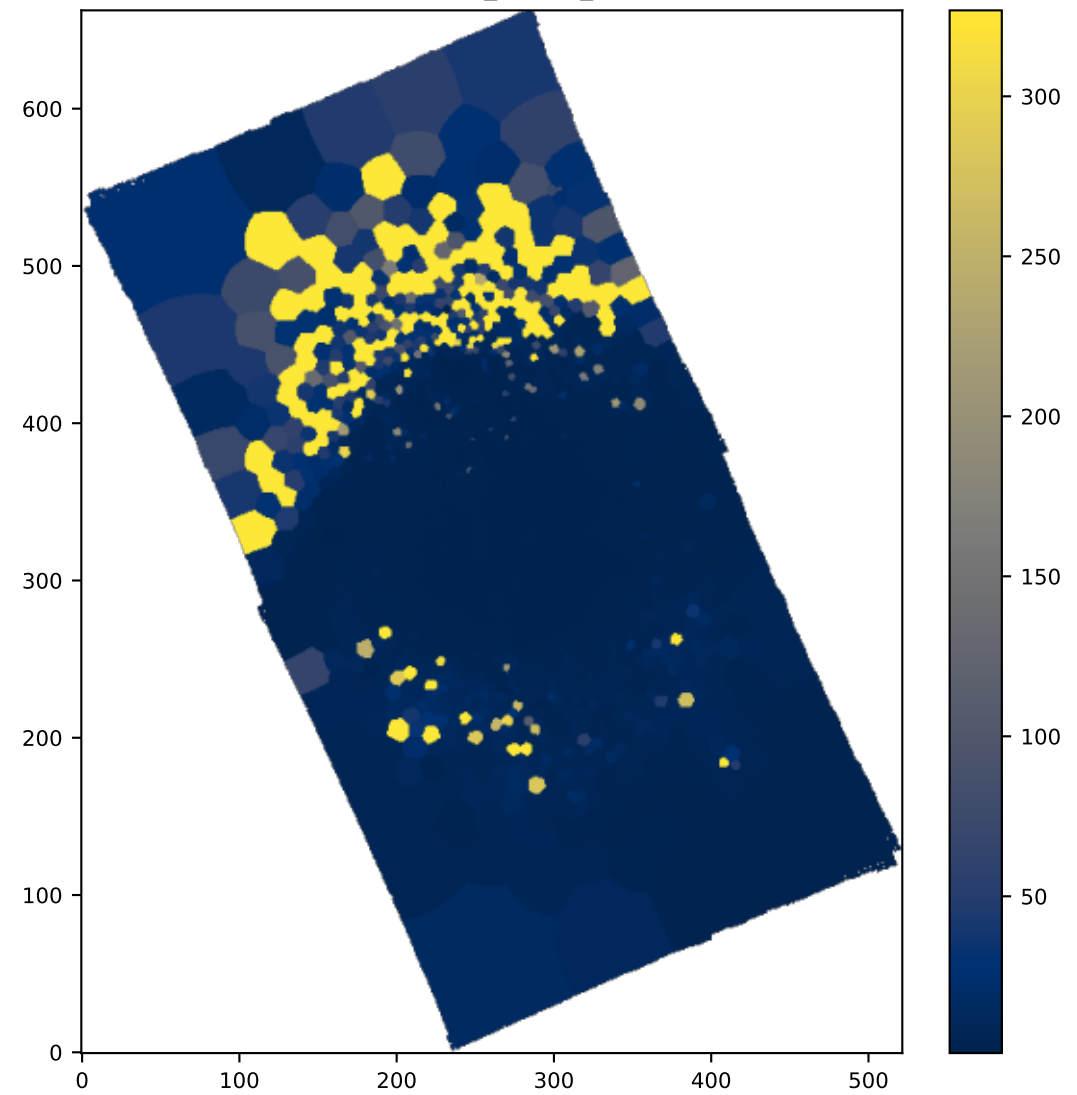
BIN OI6300_SIGMA_ERR
