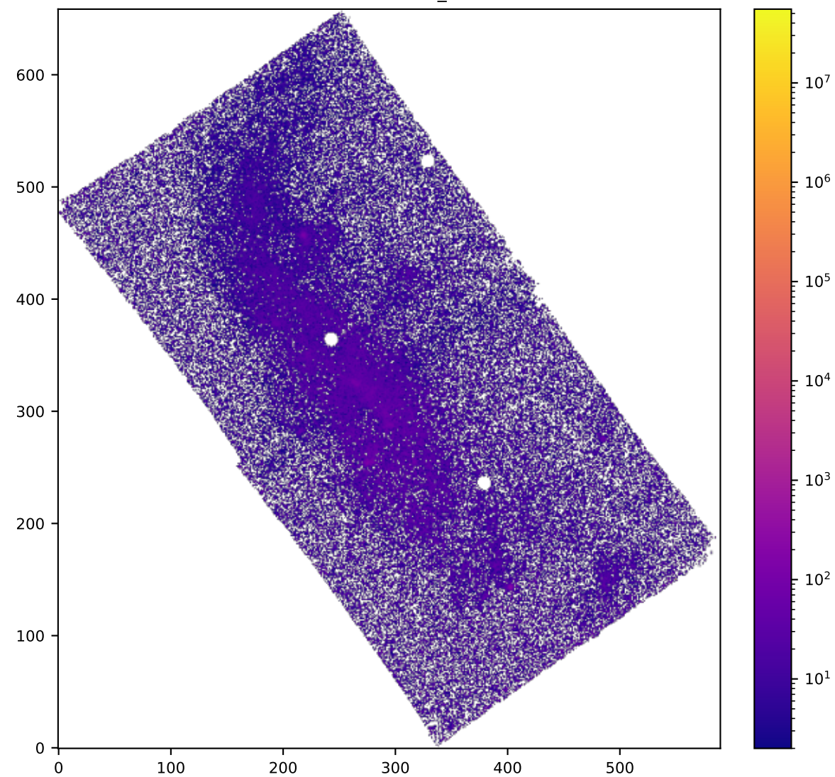
SPAXELS OI6363_SIGMA
