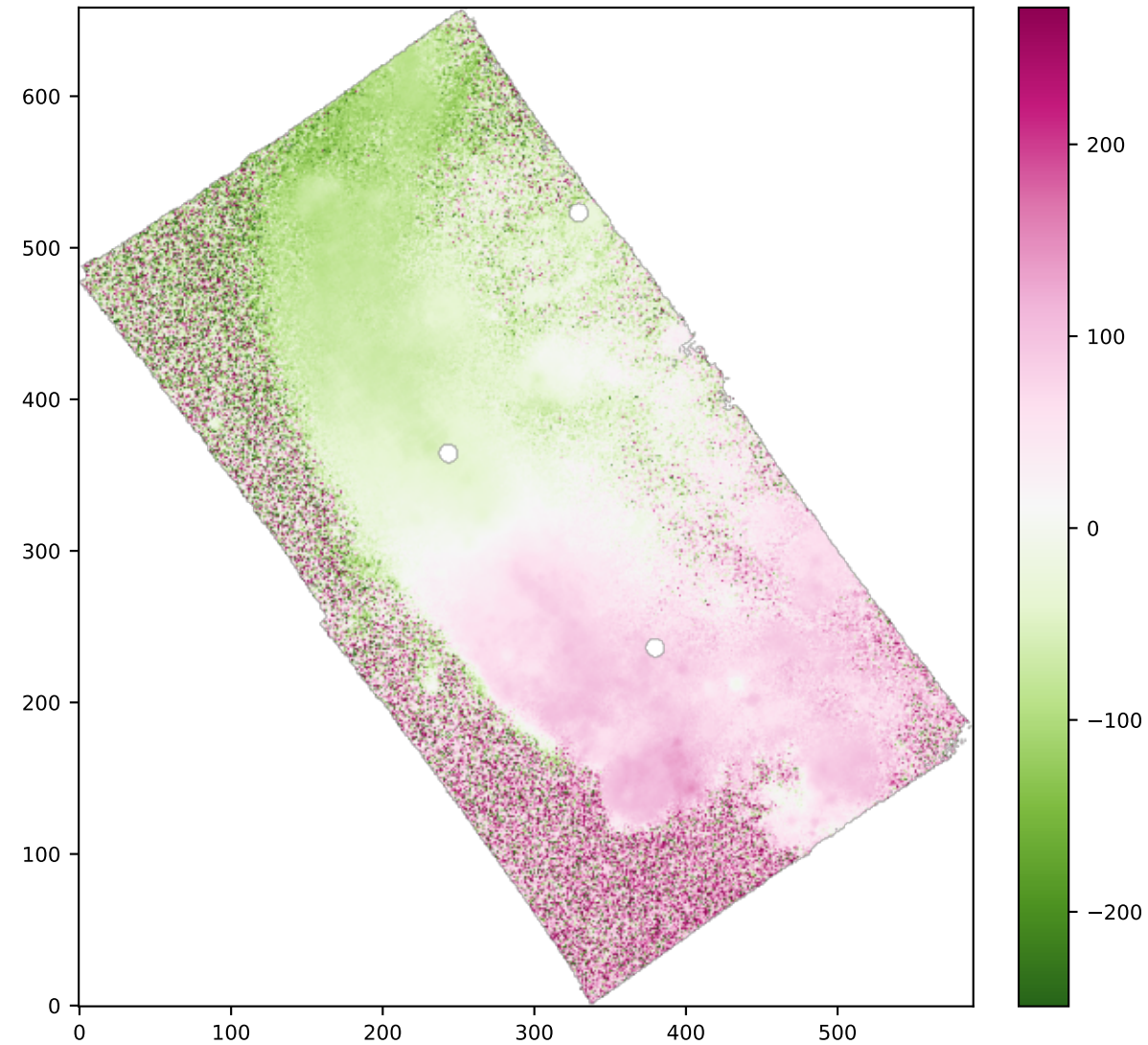
SPAXELS HB4861_VEL
