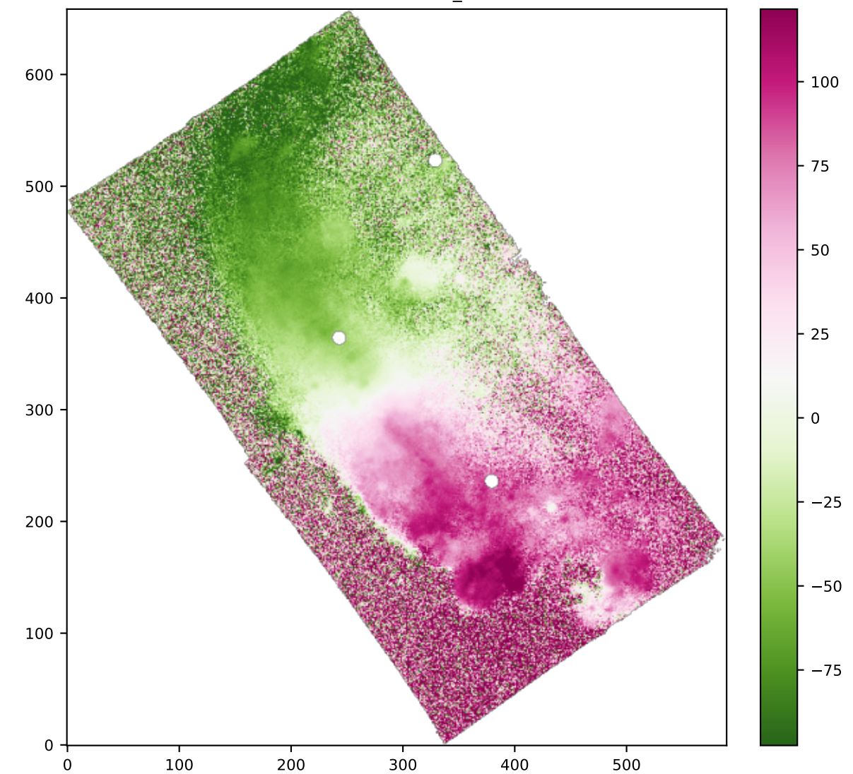
SPAXELS NII6583_VEL
