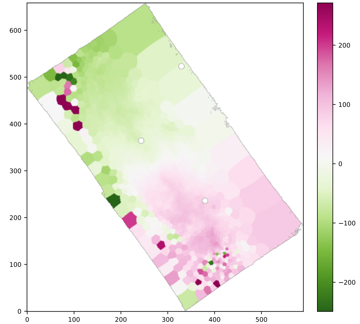
BIN HA6562_VEL
