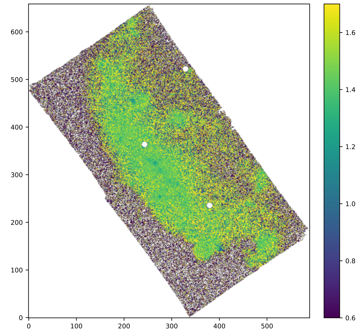
SPAXELS SII6716/SII6730
