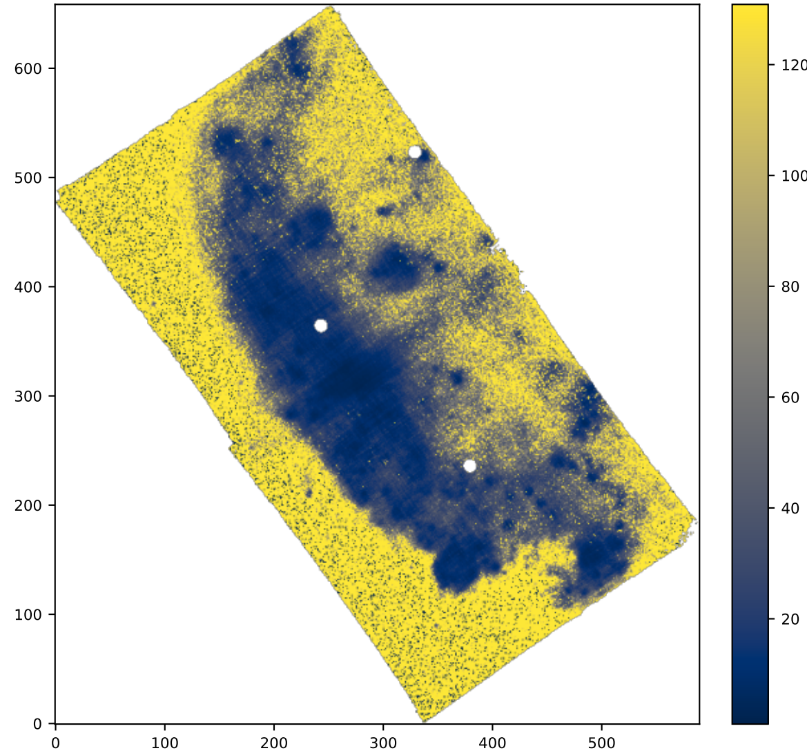
SPAXELS HA6562_SIGMA_ERR
