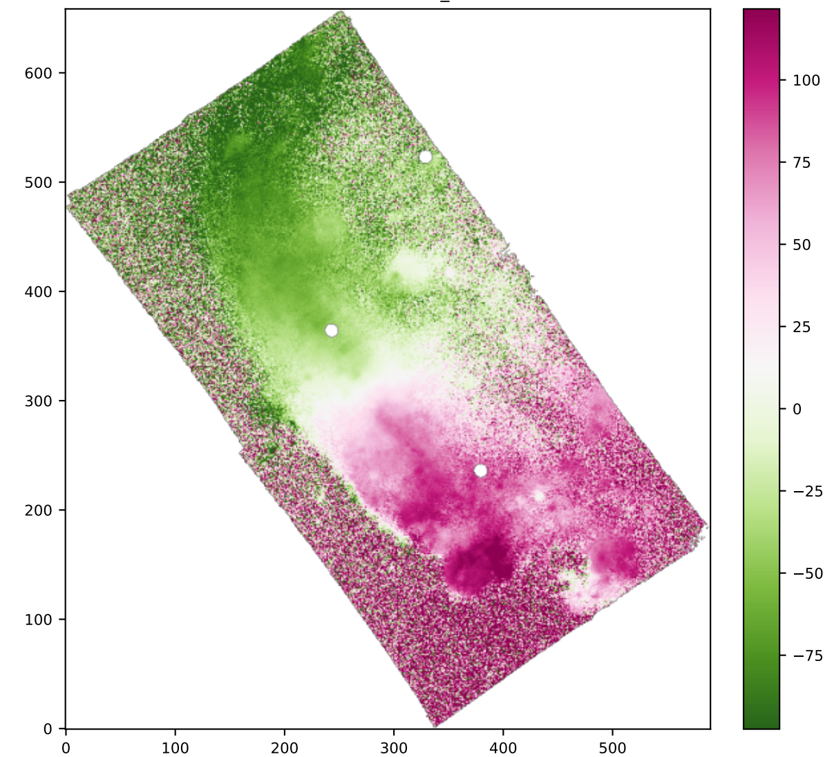
SPAXELS OI6363_VEL
