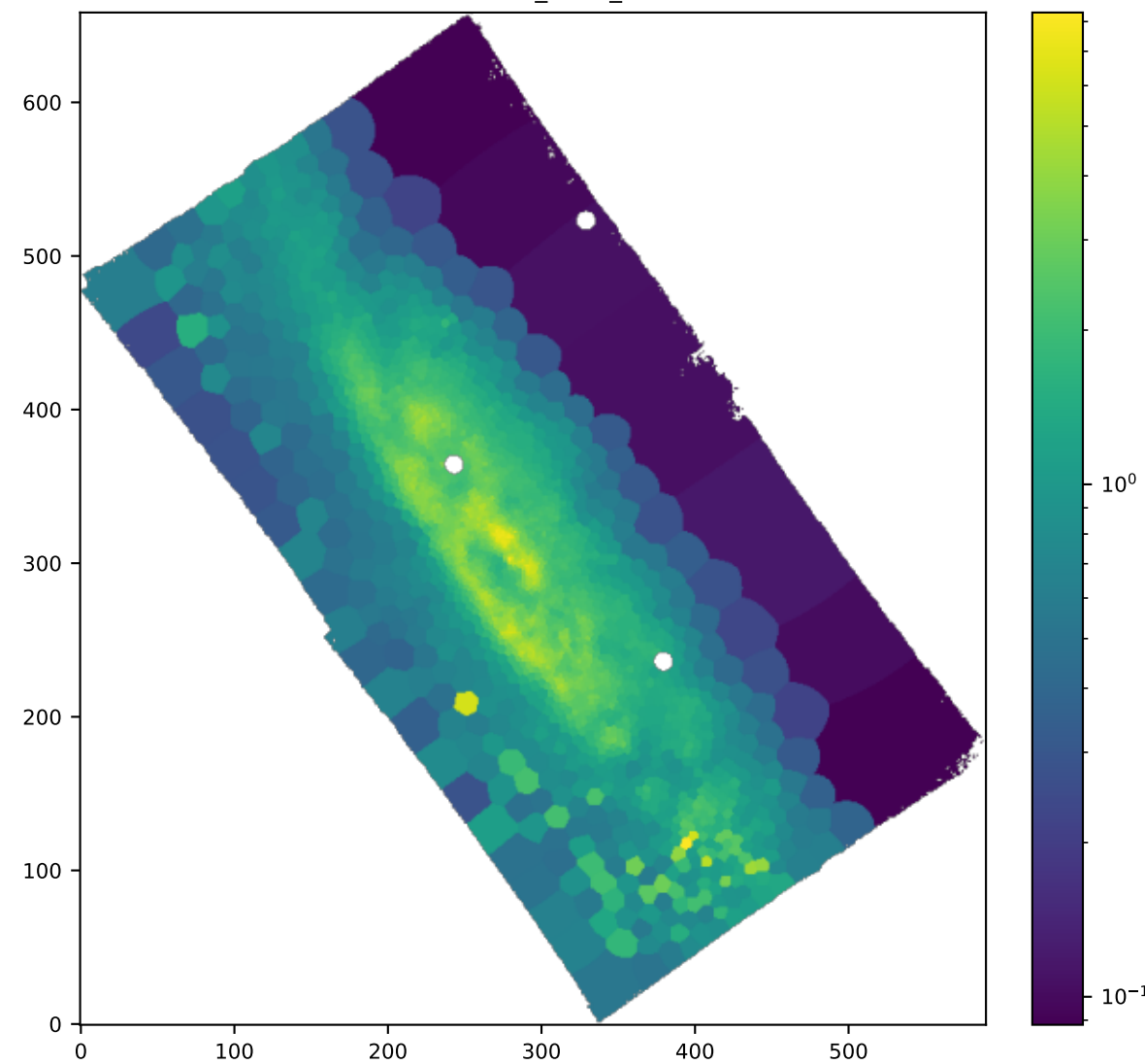
BIN OI6300_SIGMA_ERR
