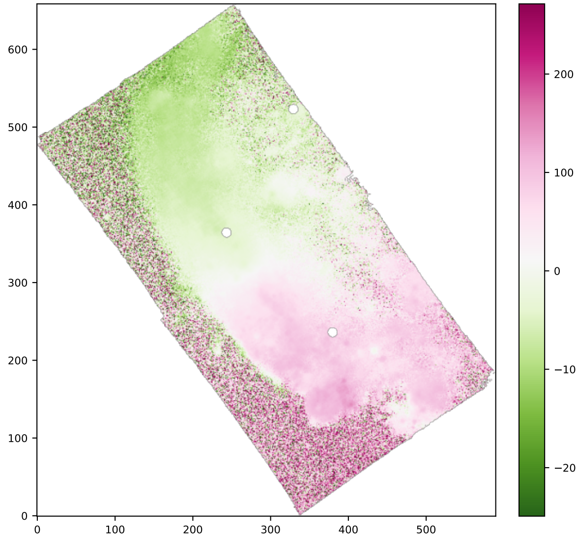
SPAXELS HA6562_VEL
