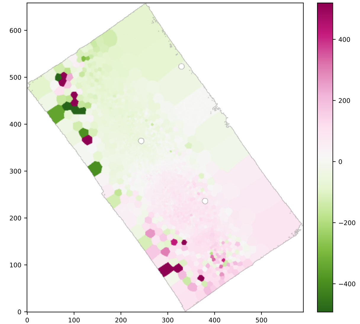
BIN OIII5006_VEL
