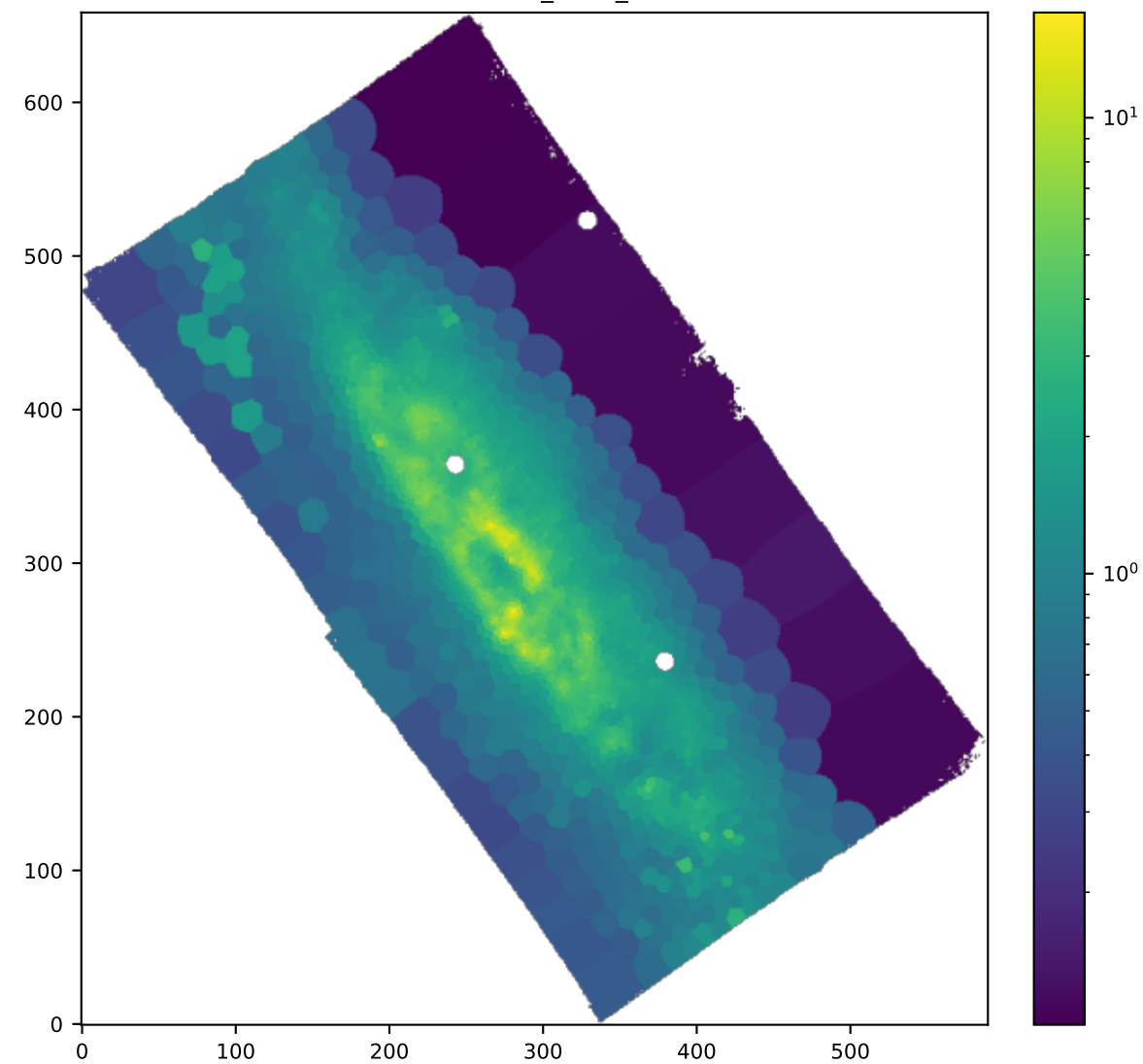
BIN HB4861_SIGMA_ERR
