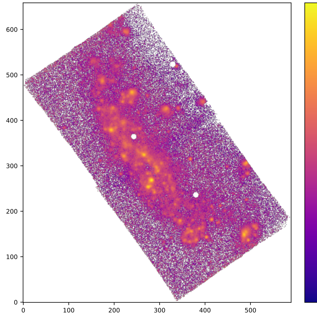
SPAXELS OIII5006_SIGMA
