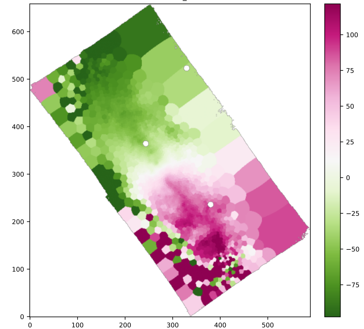
BIN OI6363_VEL
