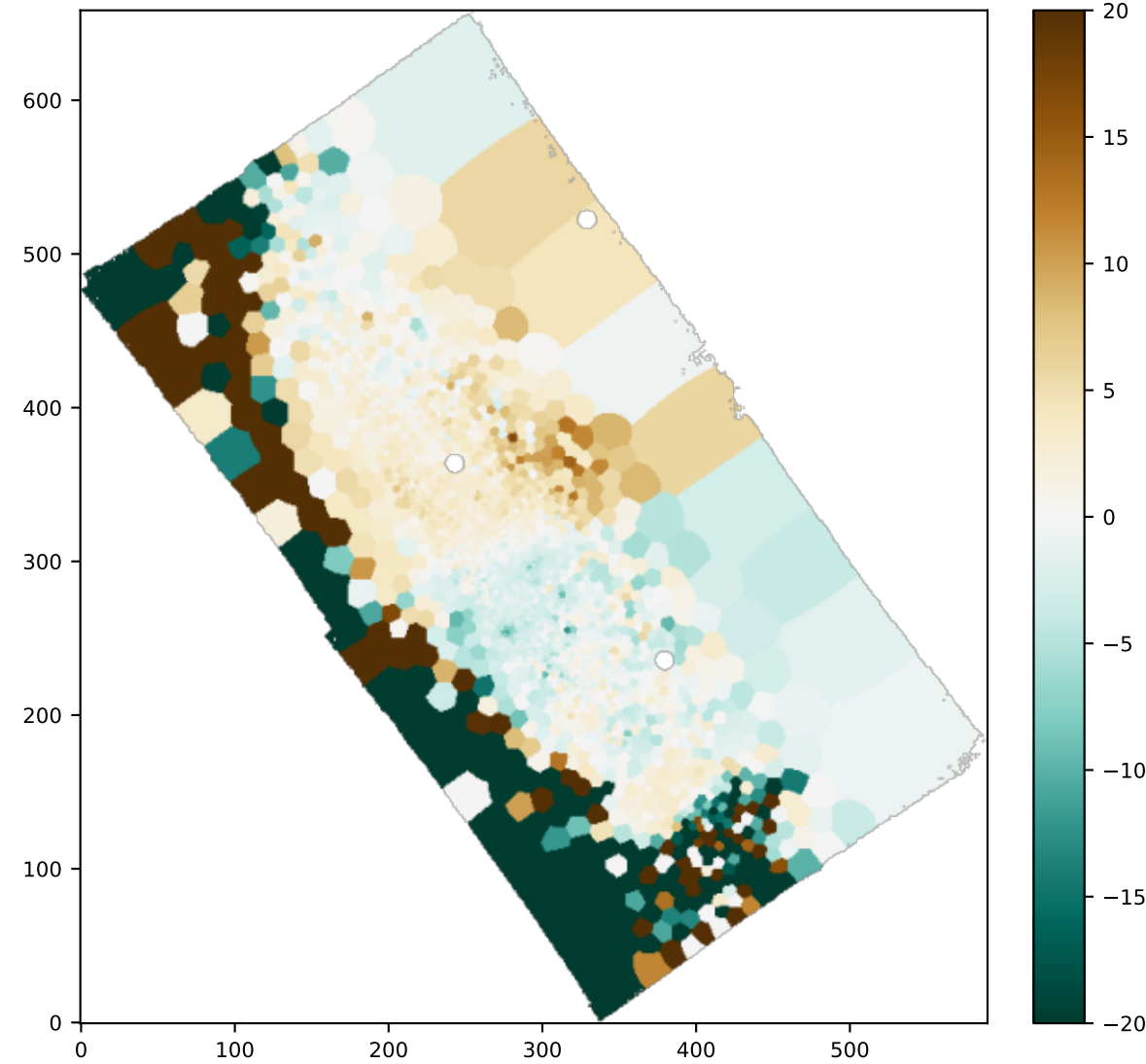
BIN SHa-SNII
