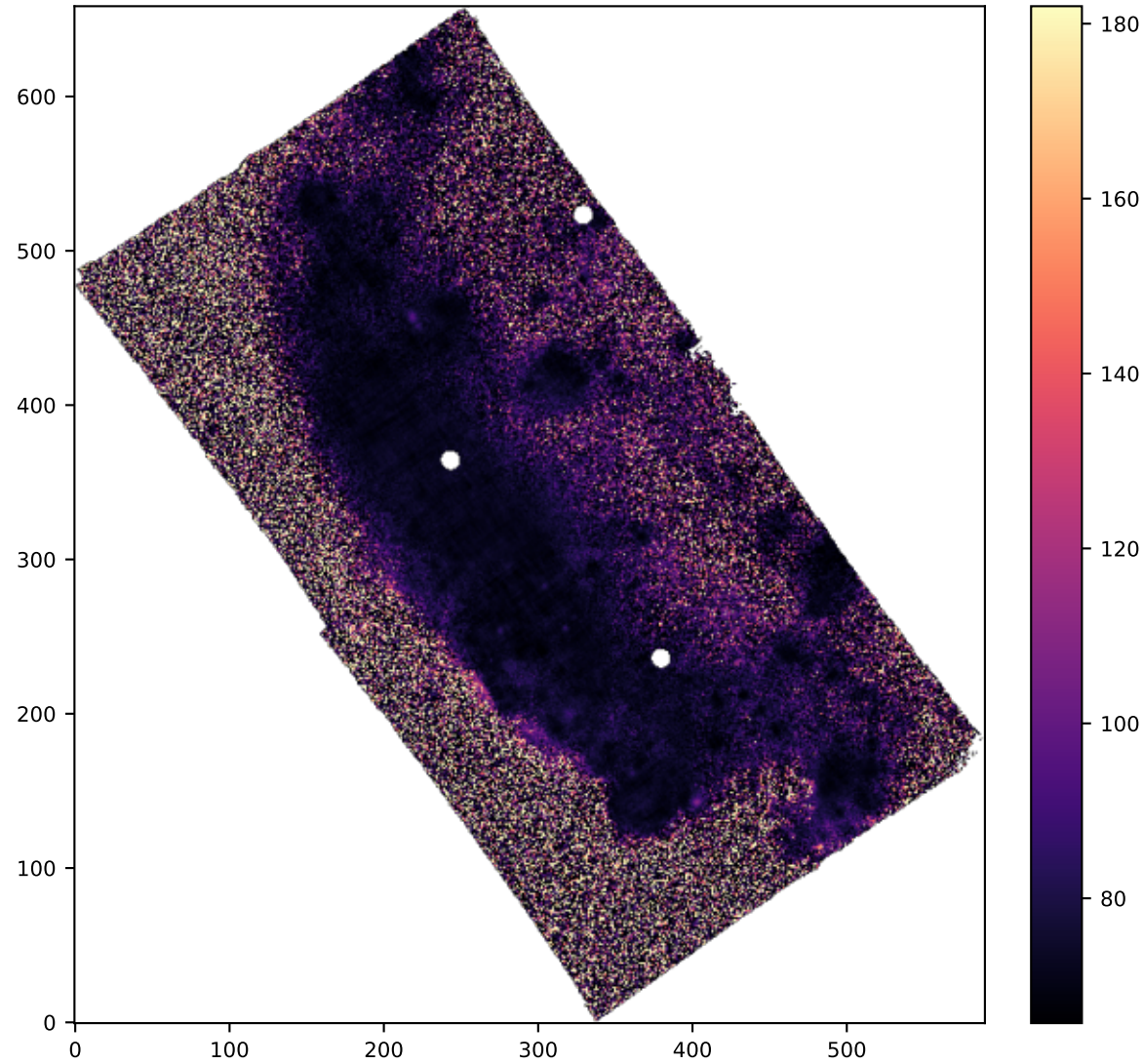
SPAXELS HB4861_SIGMA
