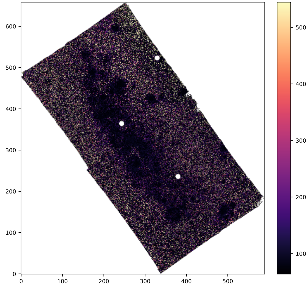
SPAXELS OIII5006_SIGMA
