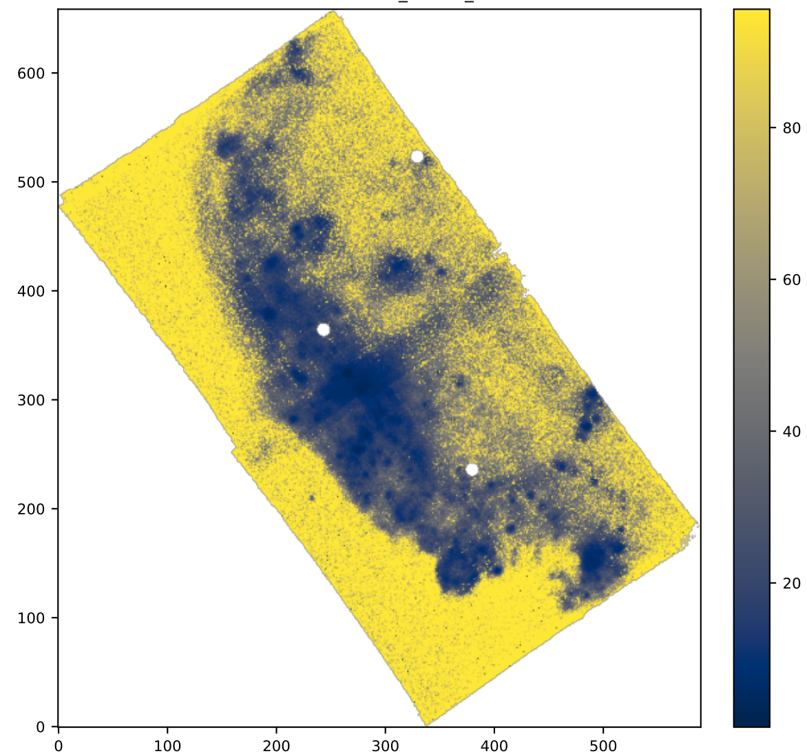
SPAXELS SII6716_SIGMA_ERR
