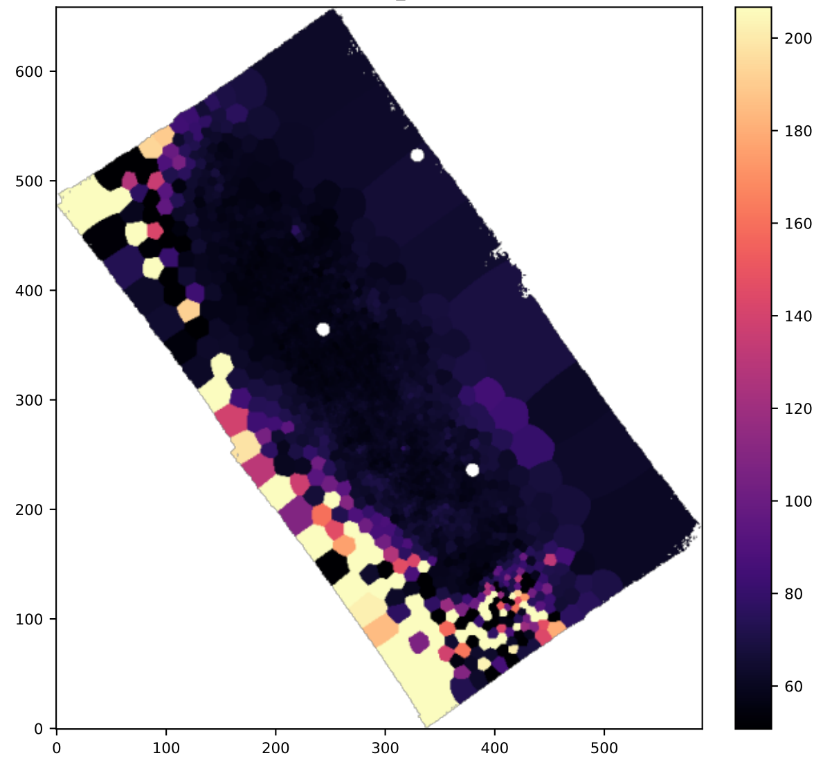
BIN OI6300_SIGMA
