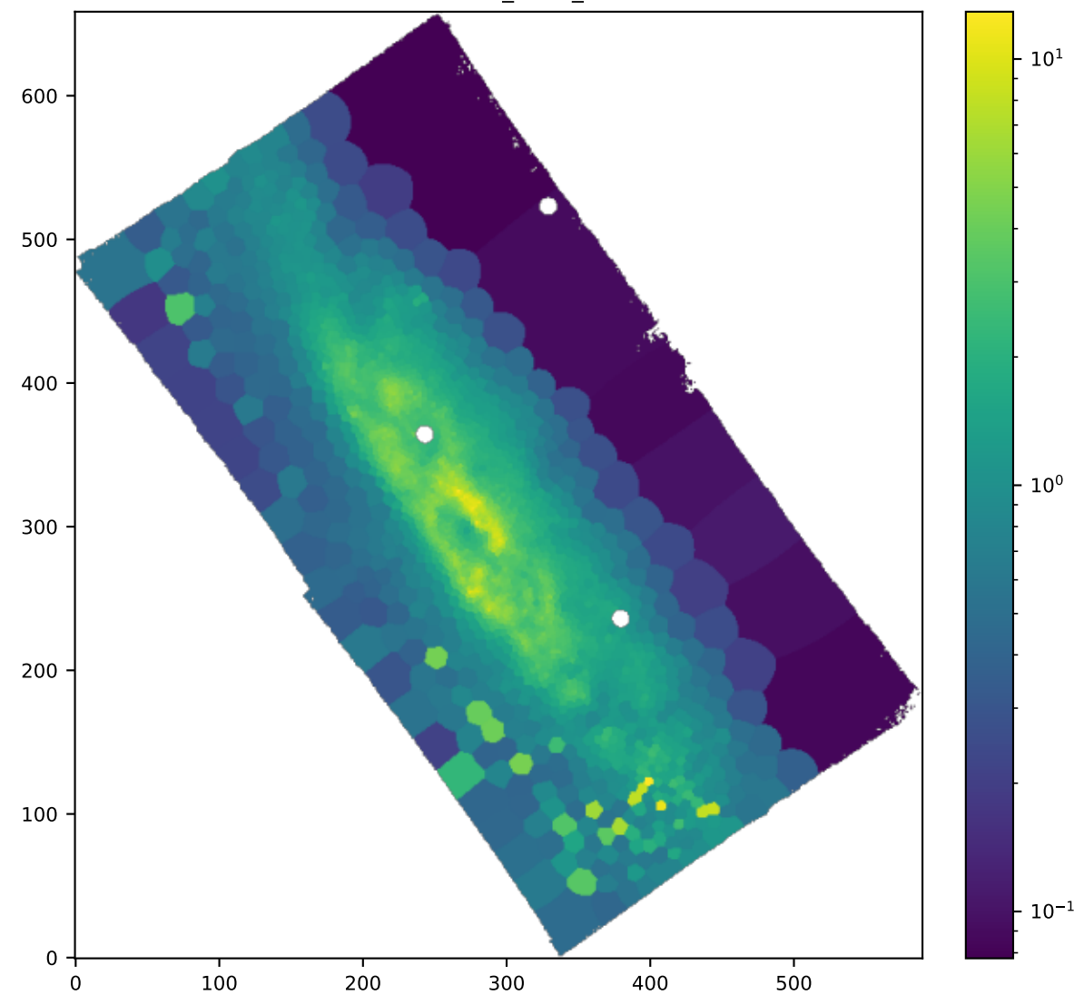
BIN SII6716_SIGMA_ERR
