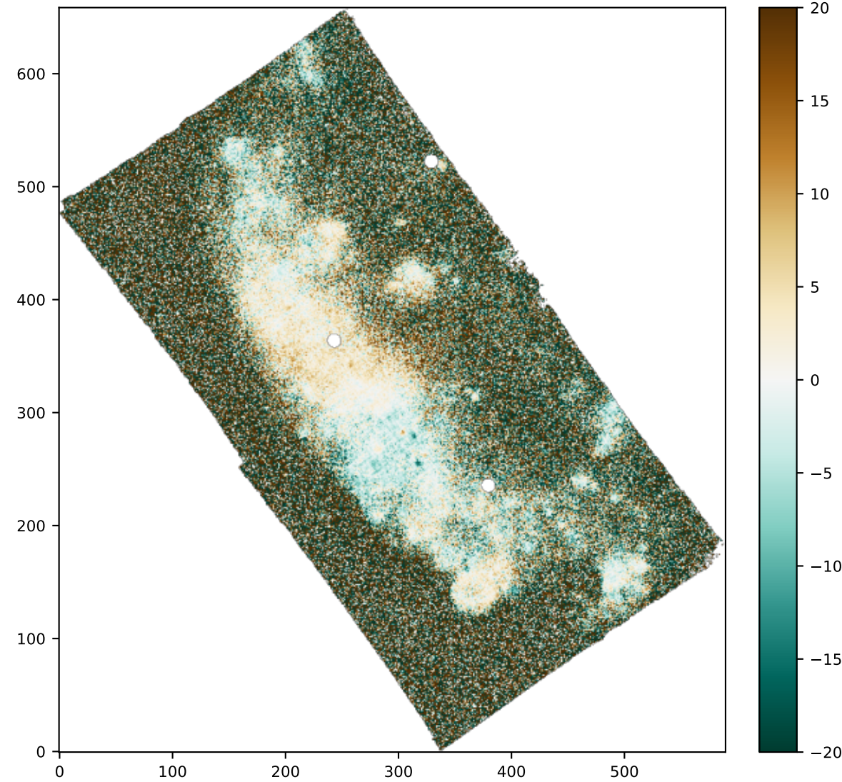
SPAXELS SHa-SNII
