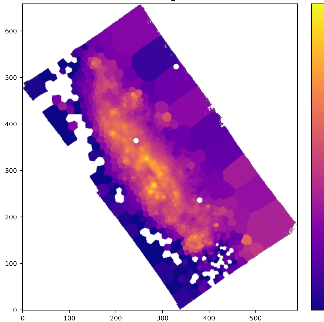
BIN HB4861_SIGMA
