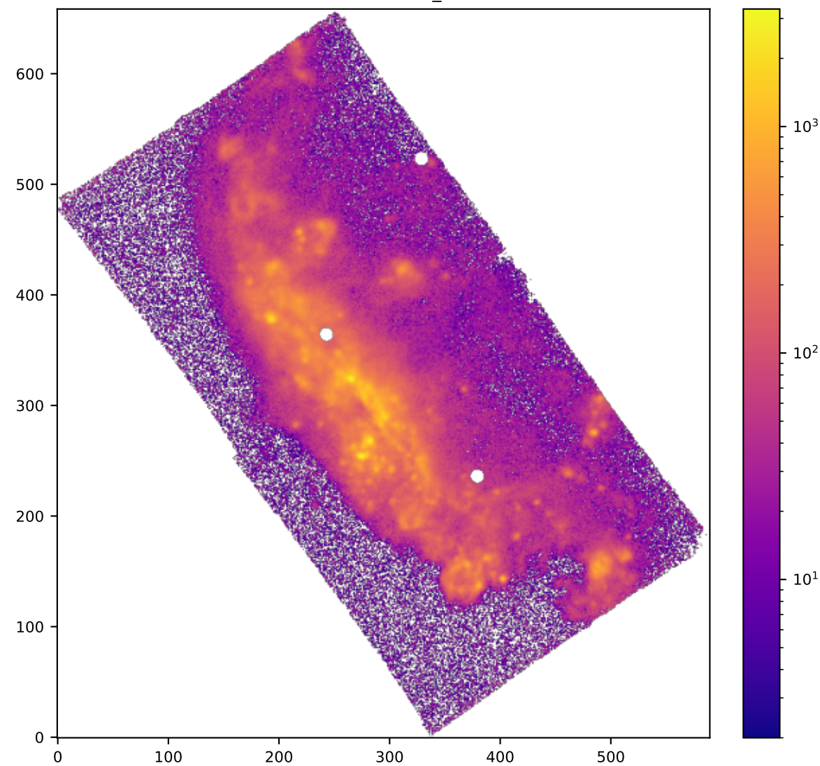
SPAXELS SII6716_SIGMA
