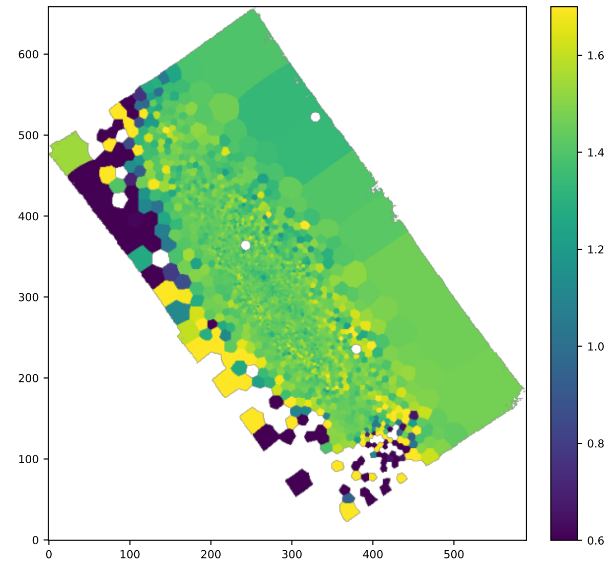
BIN SII6716/SII6730
