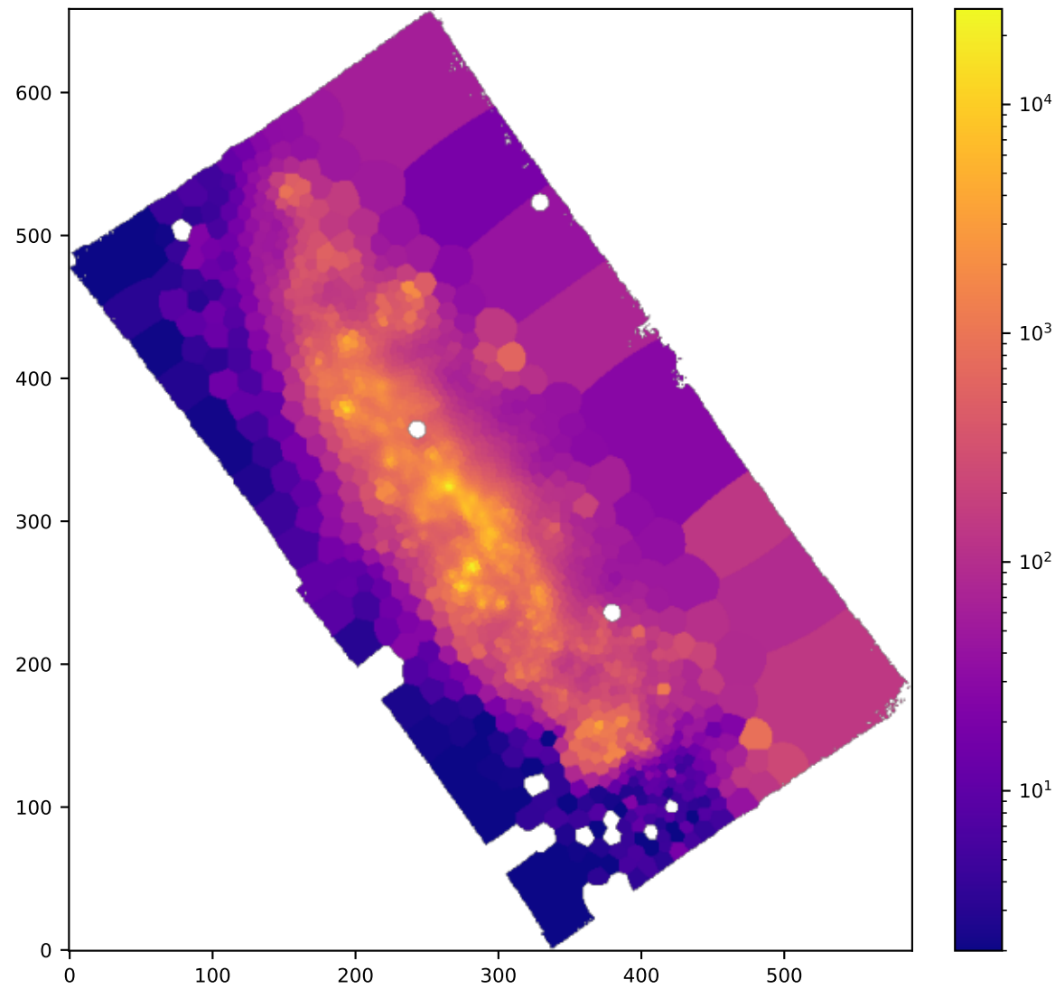
BIN HA6562_SIGMA
