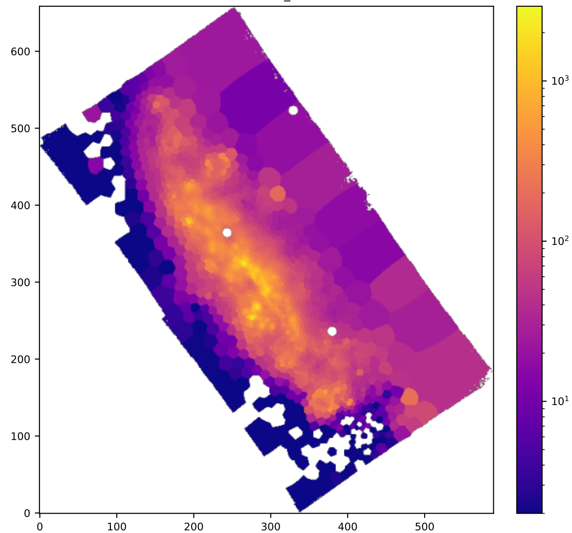
BIN SII6716_SIGMA
