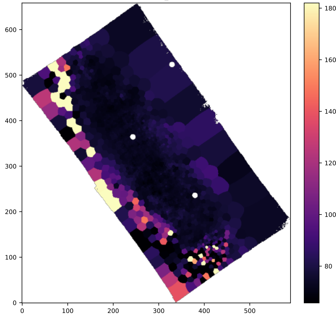
BIN HB4861_SIGMA
