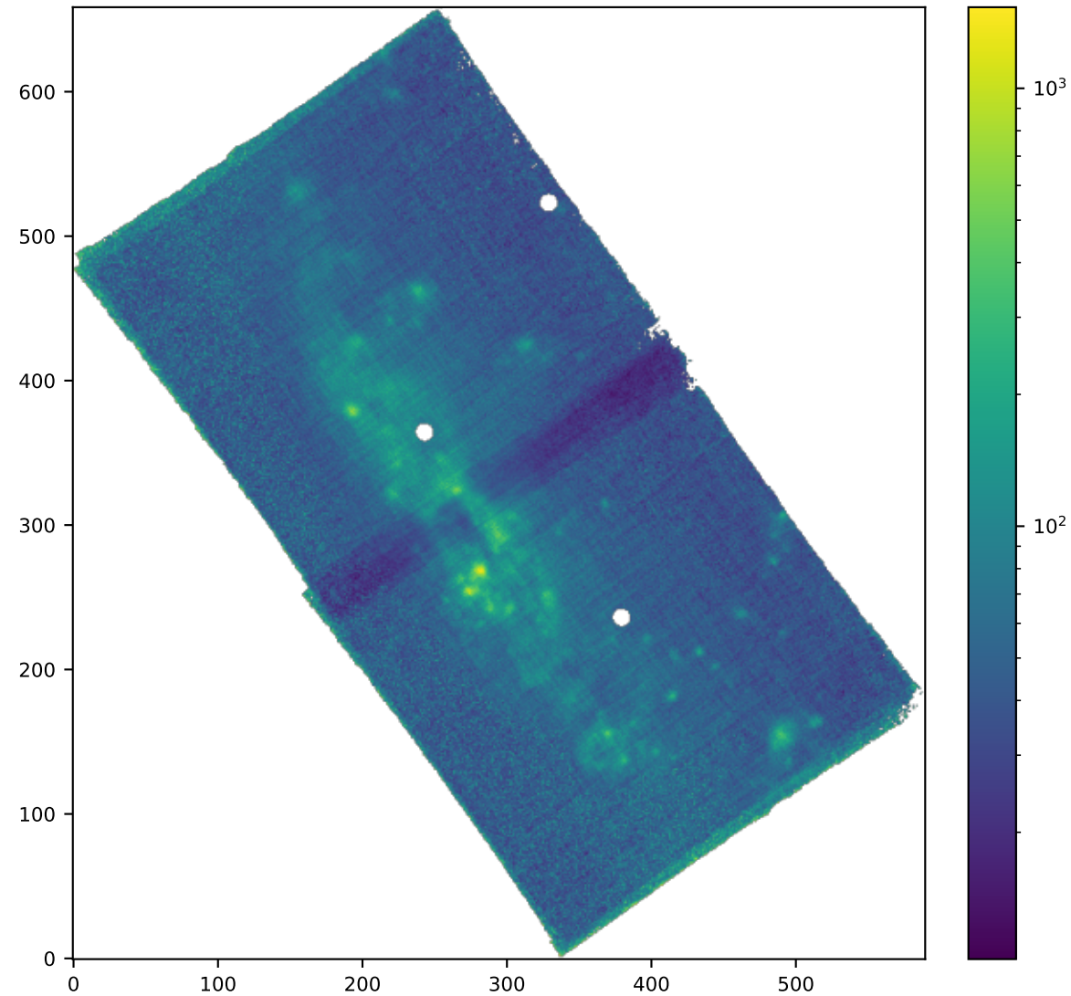
SPAXELS HB4861_SIGMA_ERR
