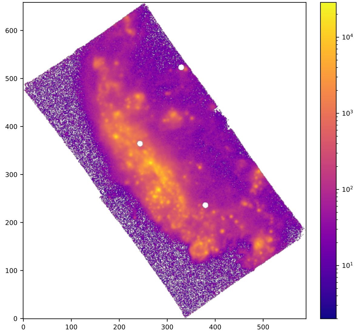
SPAXELS HA6562_SIGMA
