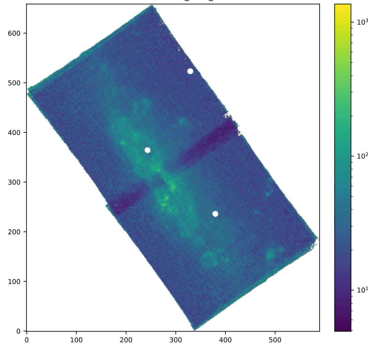
SPAXELS SII6716_SIGMA_ERR
