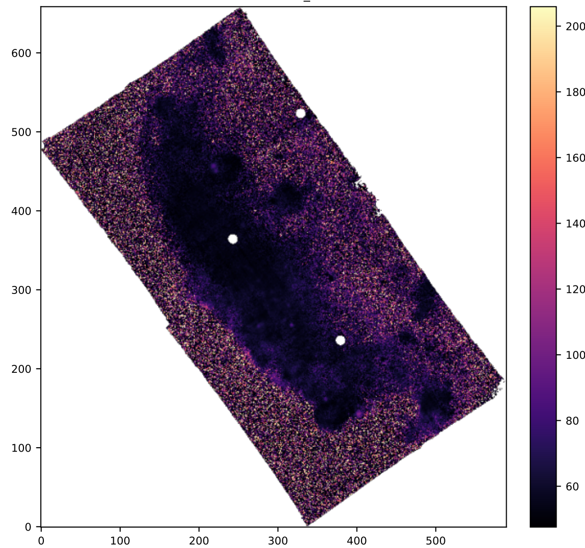
SPAXELS SII6716_SIGMA
