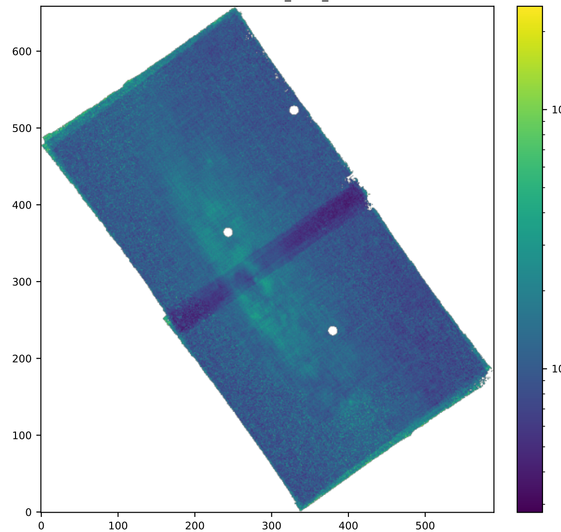
SPAXELS OI6363_SIGMA_ERR
