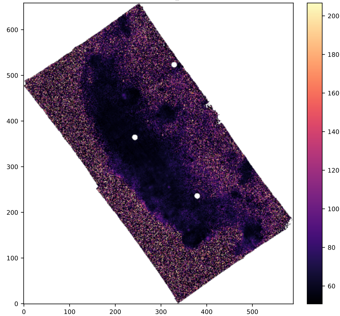
SPAXELS OI6300_SIGMA
