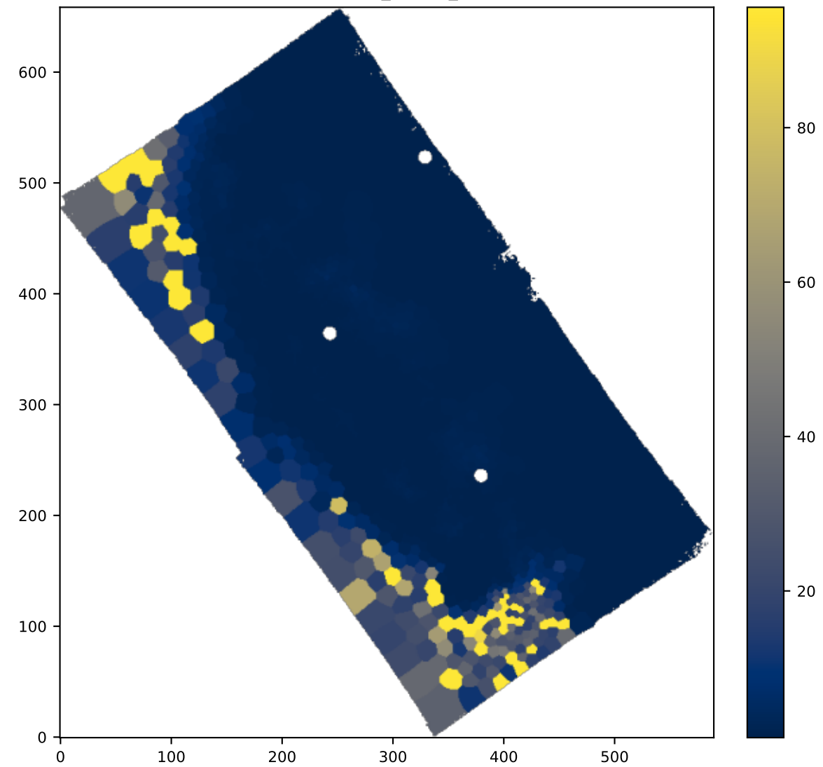
BIN OI6363_SIGMA_ERR
