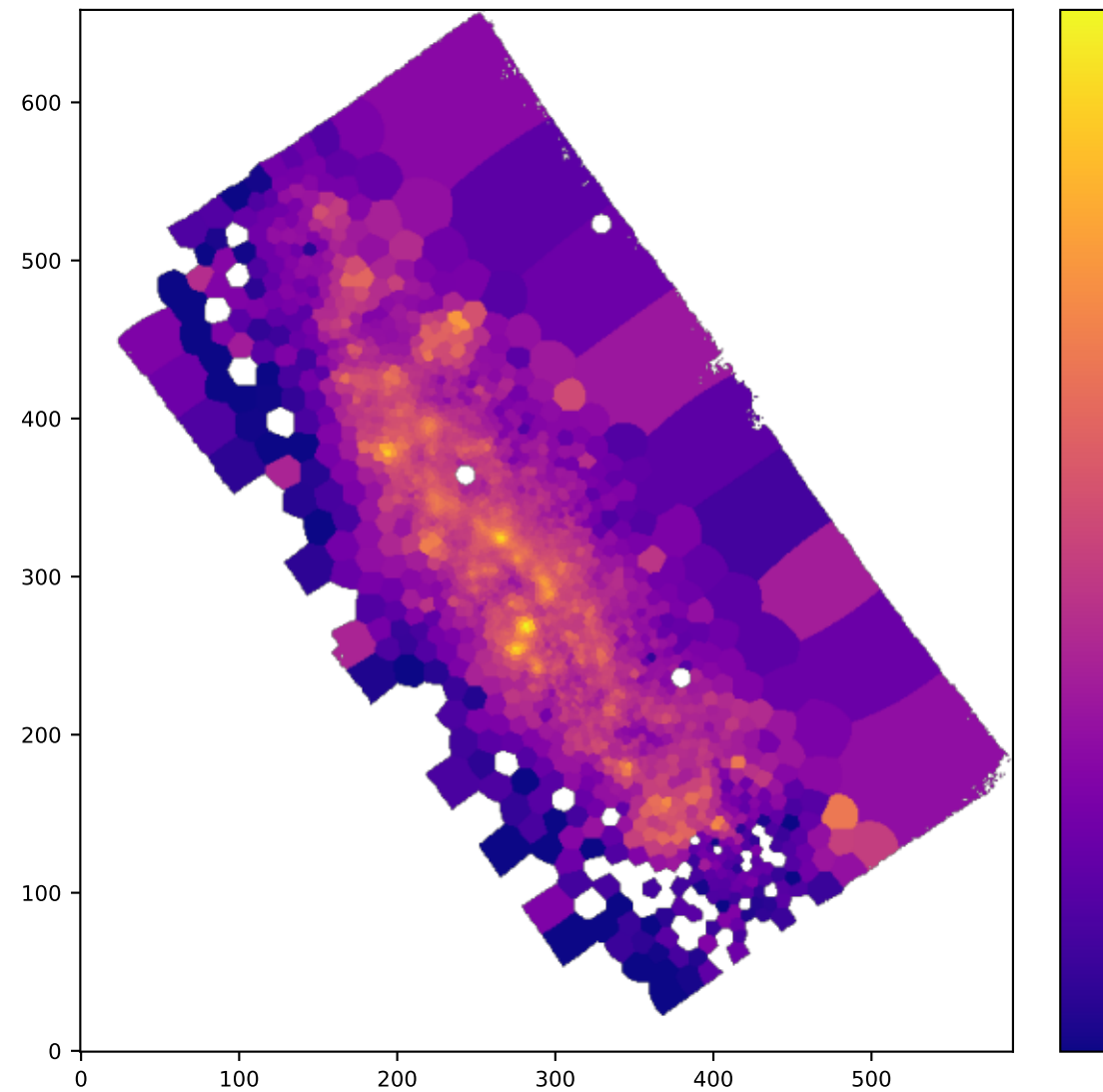
BIN OIII5006_SIGMA
