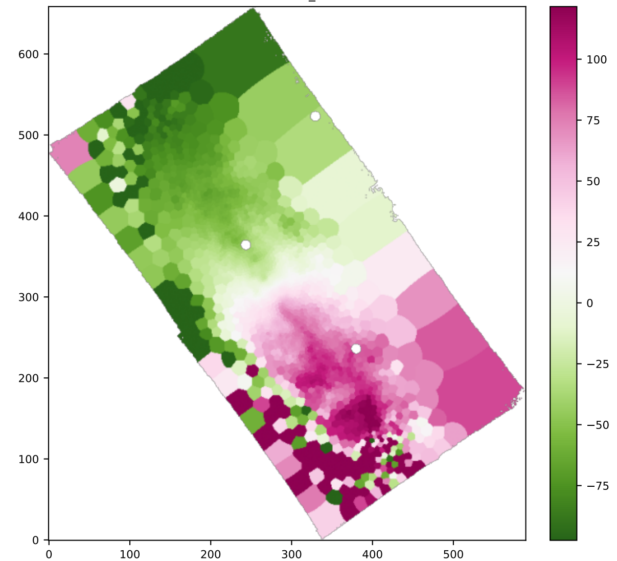
BIN OI6300_VEL
