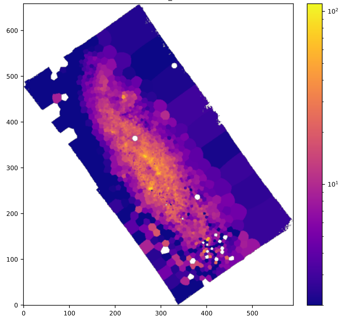
BIN OI6363_SIGMA
