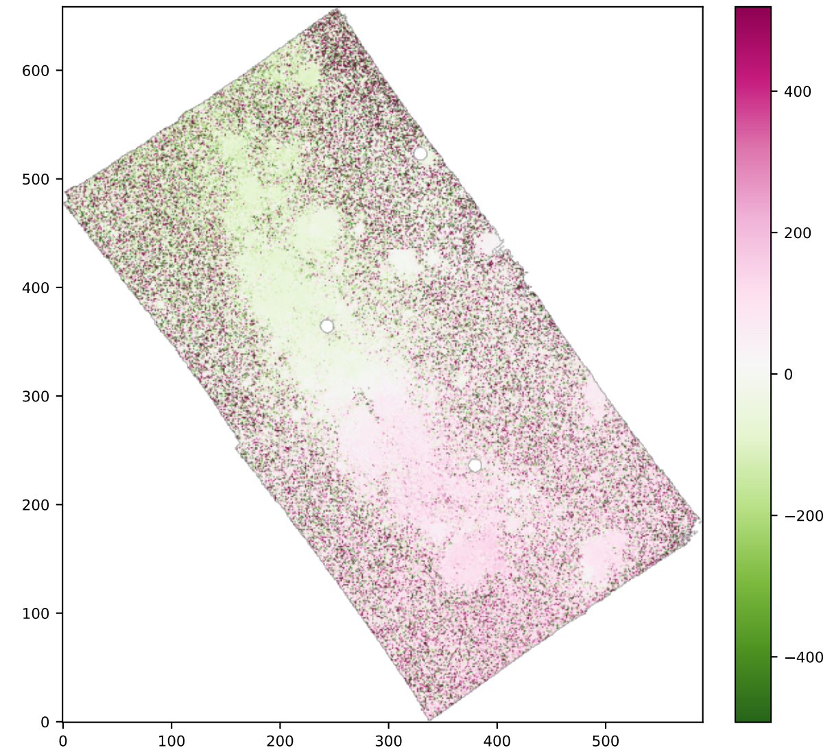
SPAXELS OIII5006_VEL
