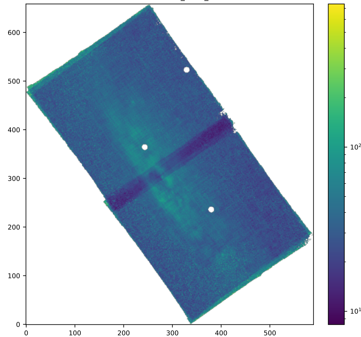
SPAXELS OI6300_SIGMA_ERR
