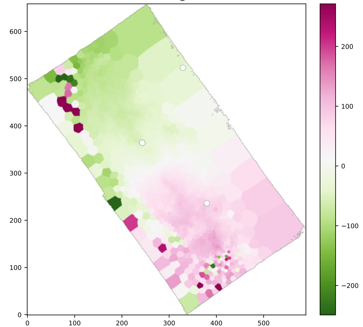
BIN HB4861_VEL
