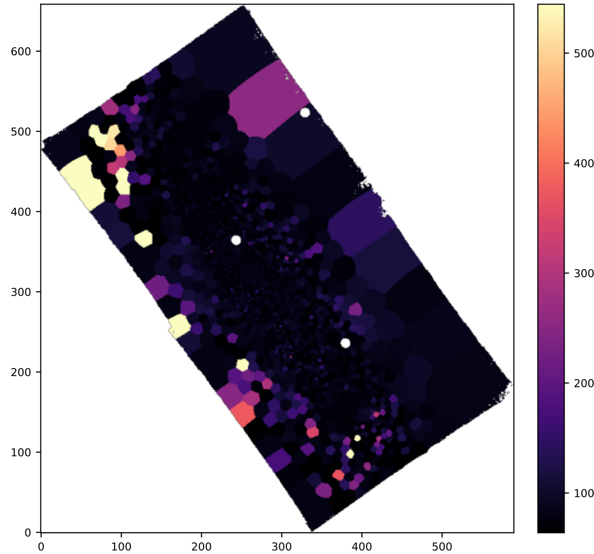
BIN OIII5006_SIGMA
