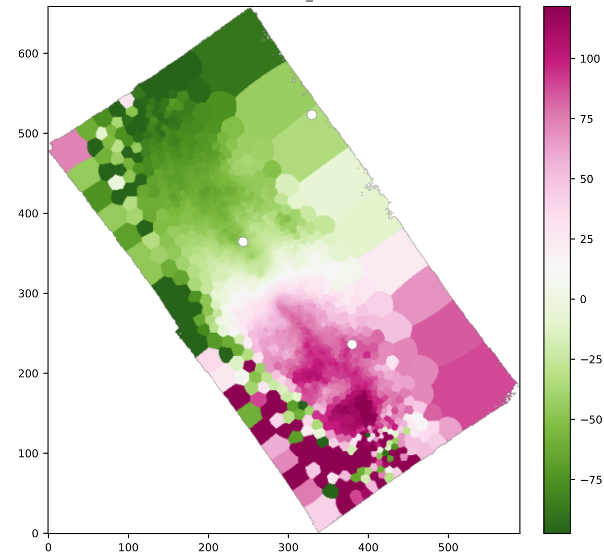
BIN SII6716_VEL
