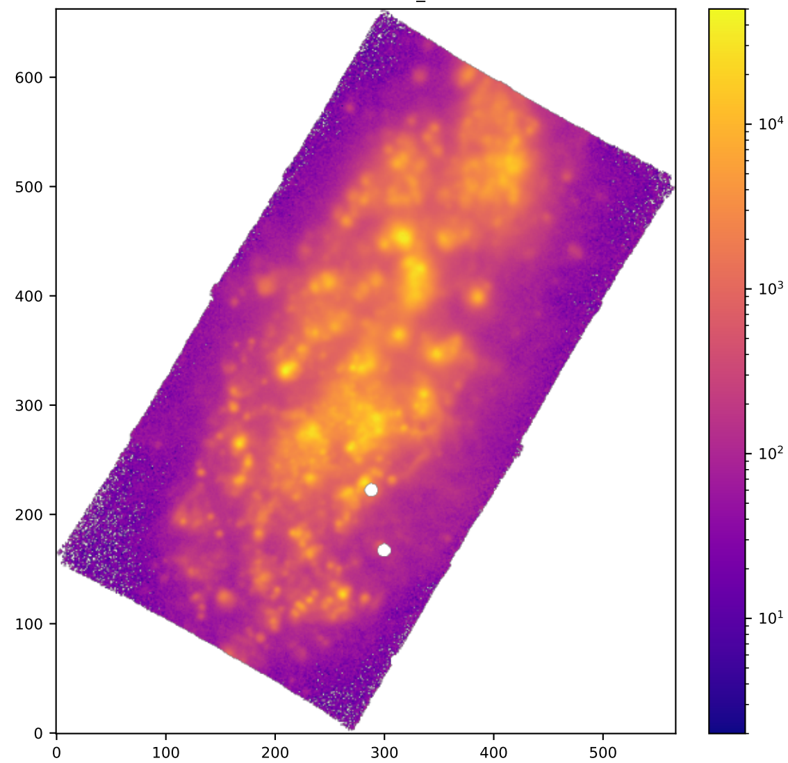
SPAXELS HA6562_SIGMA
