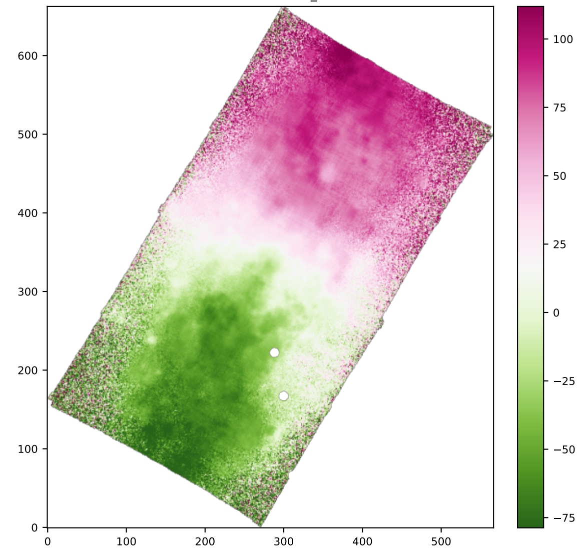
SPAXELS HA6562_VEL
