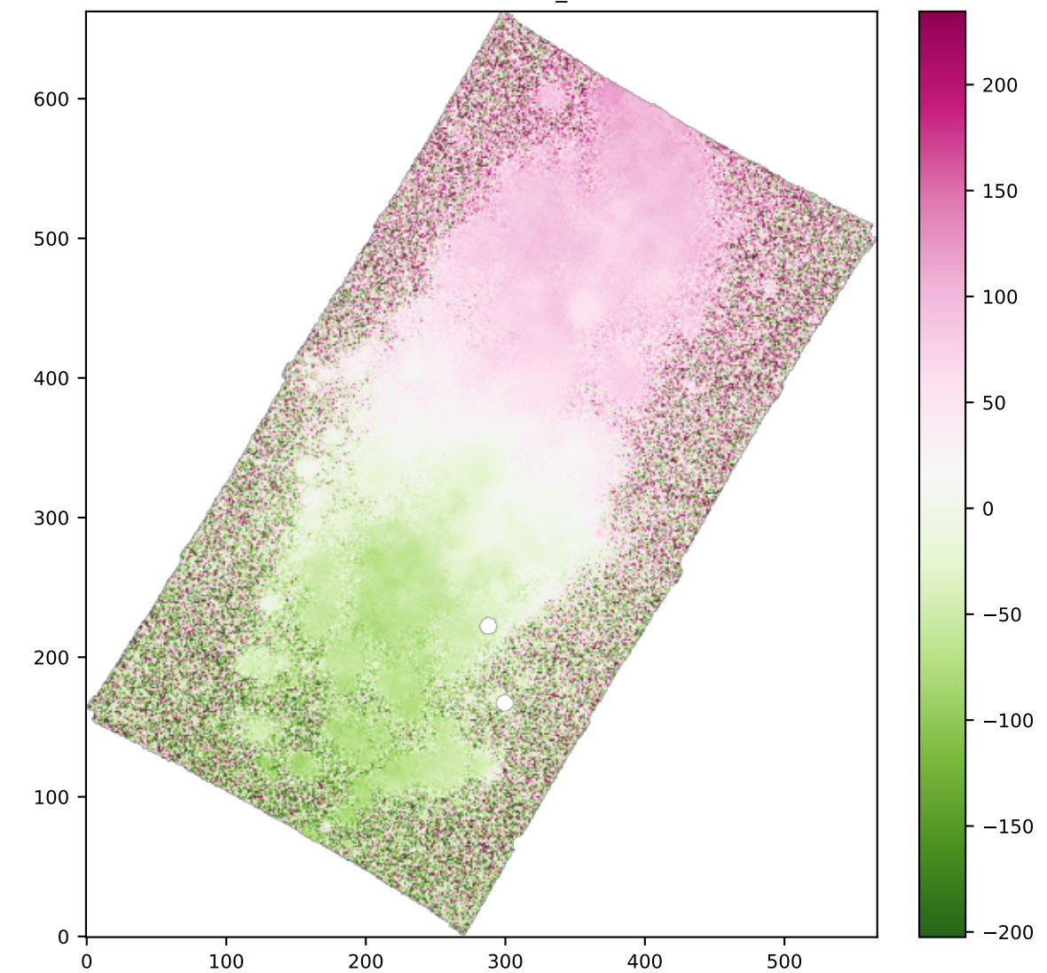
SPAXELS OIII5006_VEL
