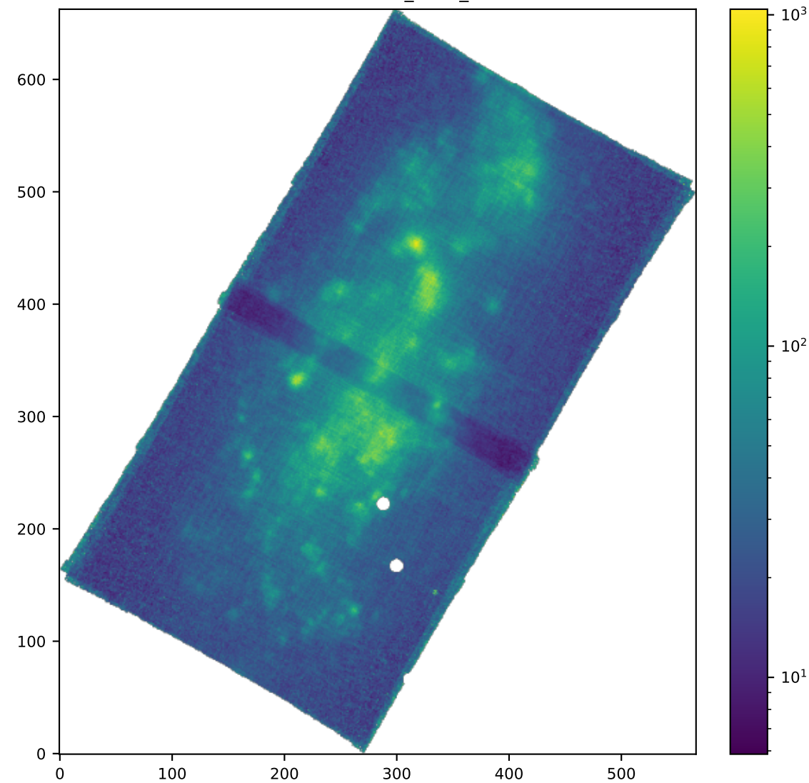
SPAXELS SII6716_SIGMA_ERR
