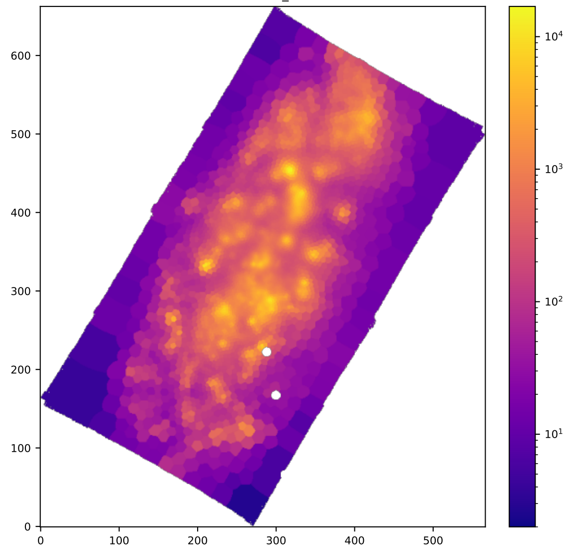
BIN HB4861_SIGMA
