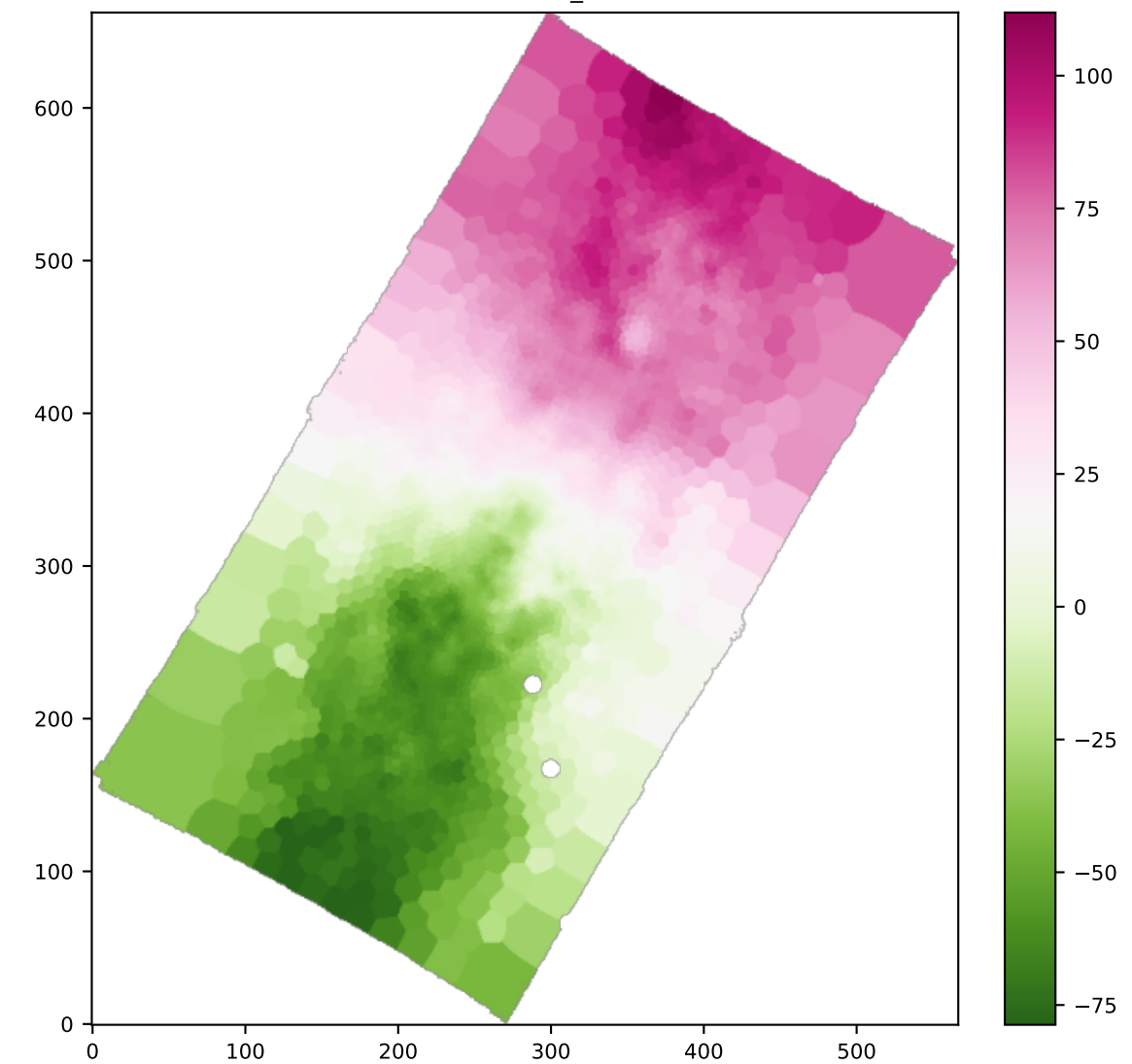
BIN HA6562_VEL
