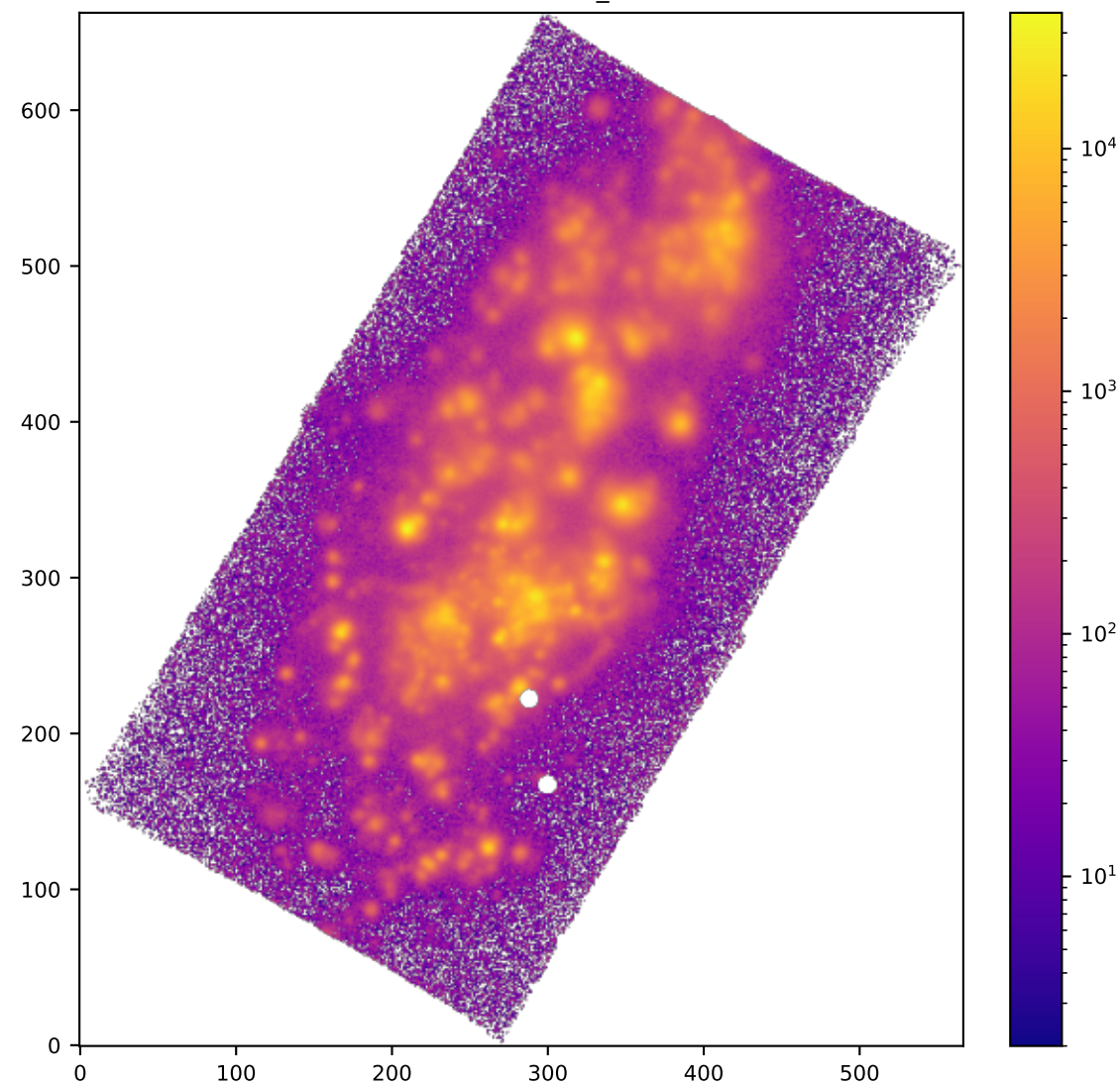
SPAXELS OIII5006_SIGMA
