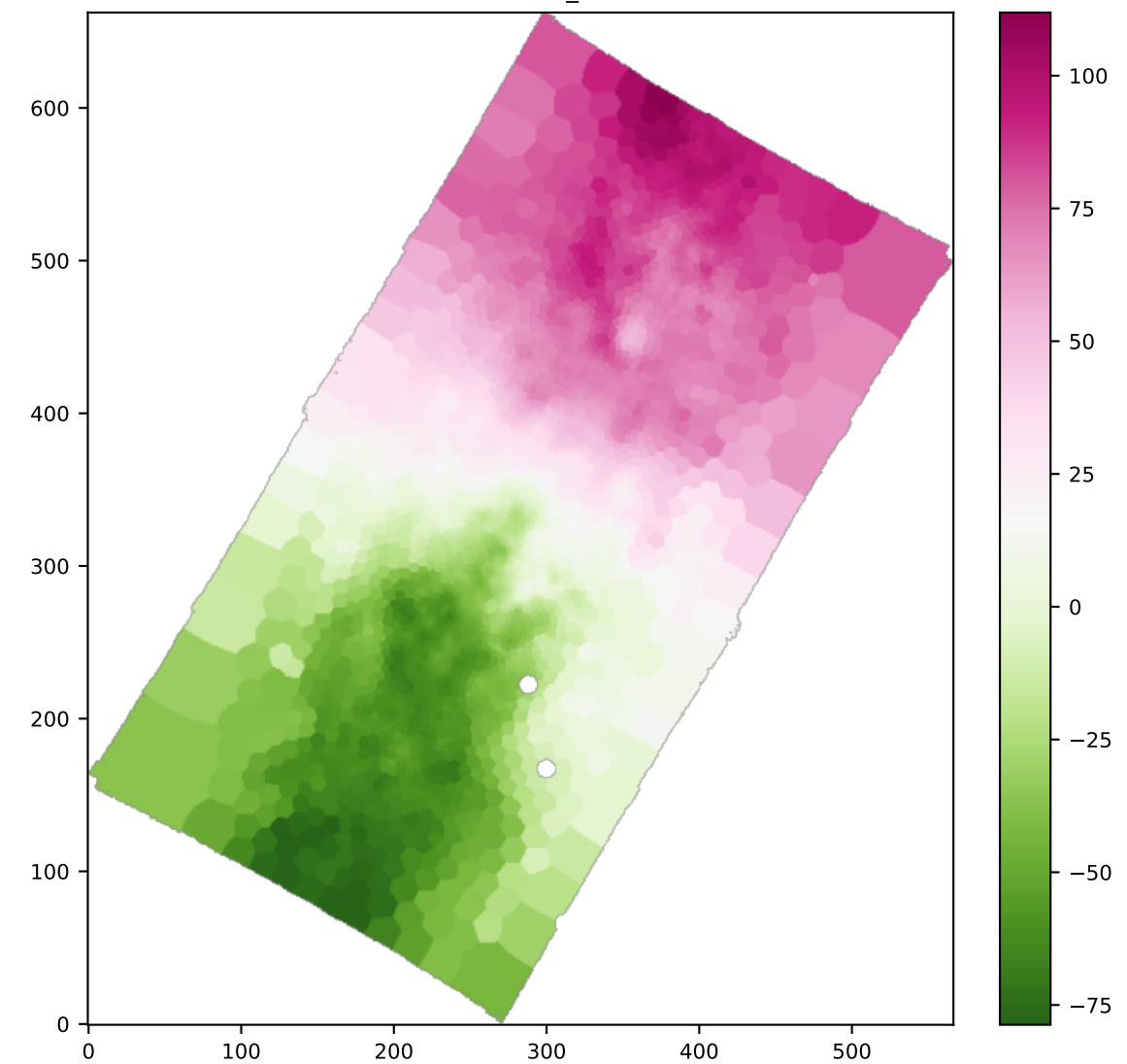
BIN HB4861_VEL
