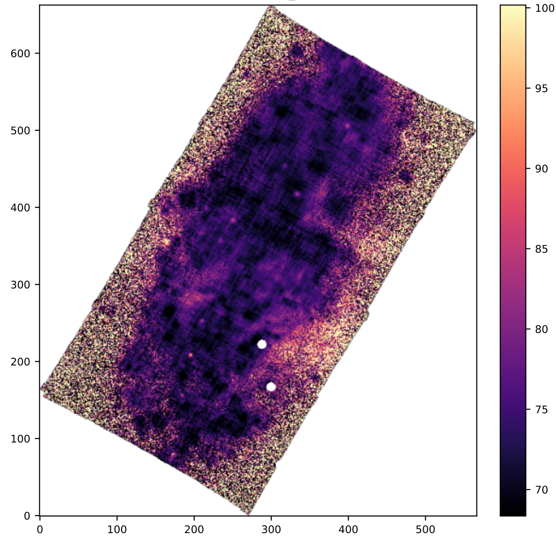
SPAXELS HB4861_SIGMA
