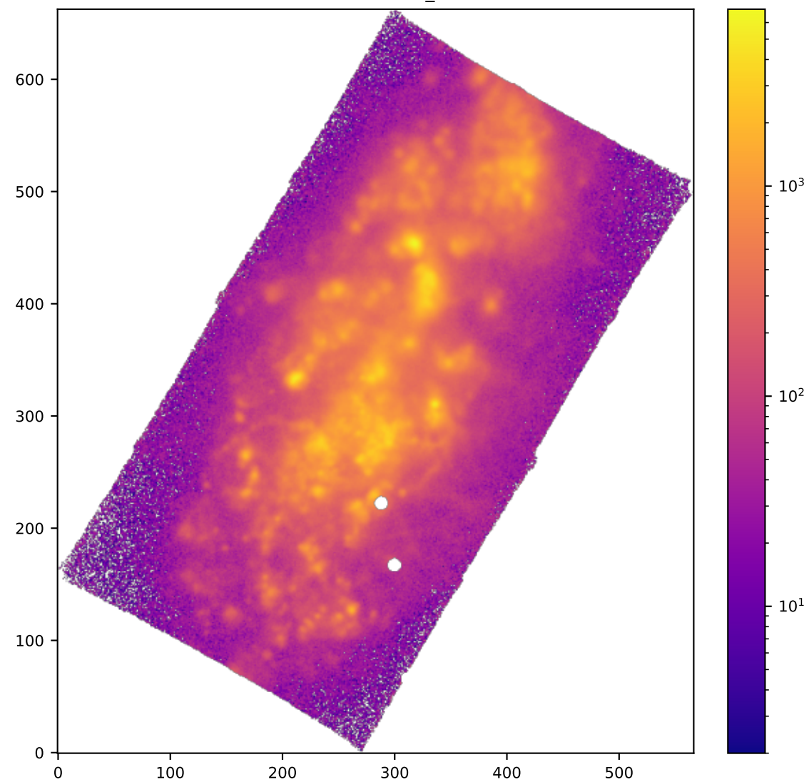
SPAXELS SII6716_SIGMA
