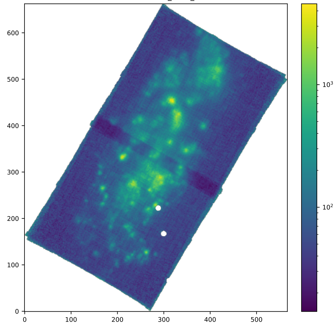
SPAXELS HB4861_SIGMA_ERR
