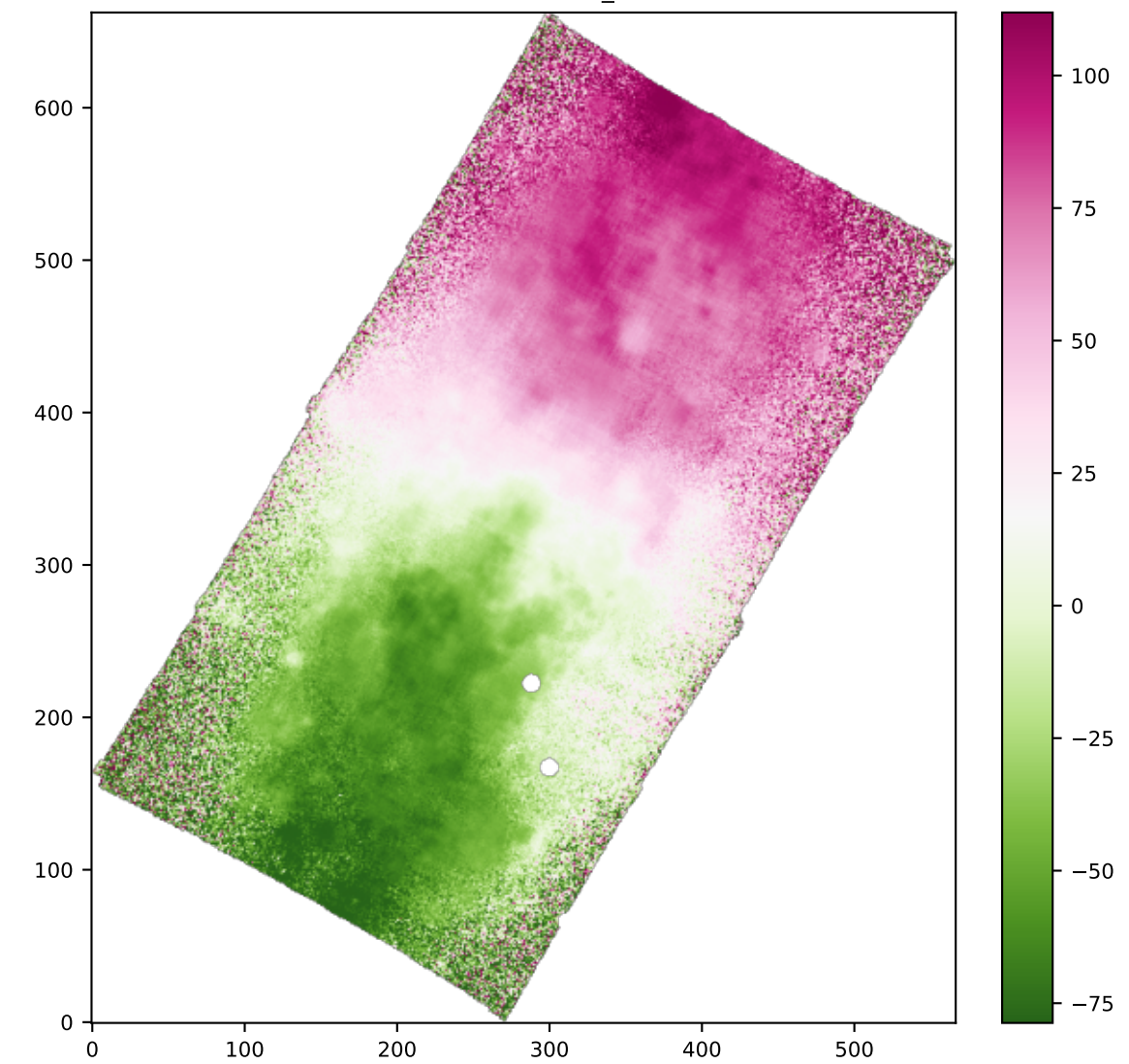
SPAXELS HB4861_VEL
