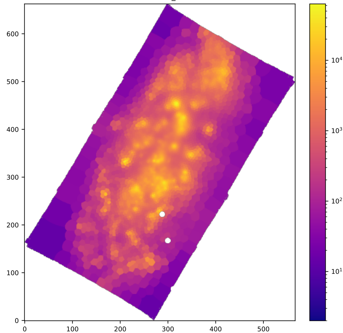
BIN HA6562_SIGMA
