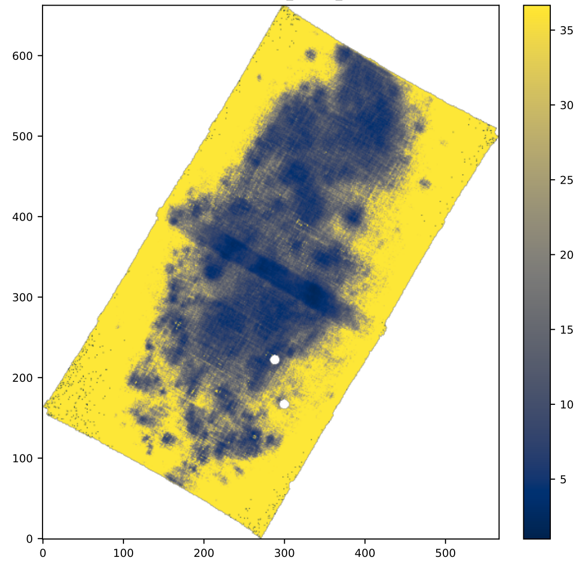
SPAXELS HA6562_SIGMA_ERR
