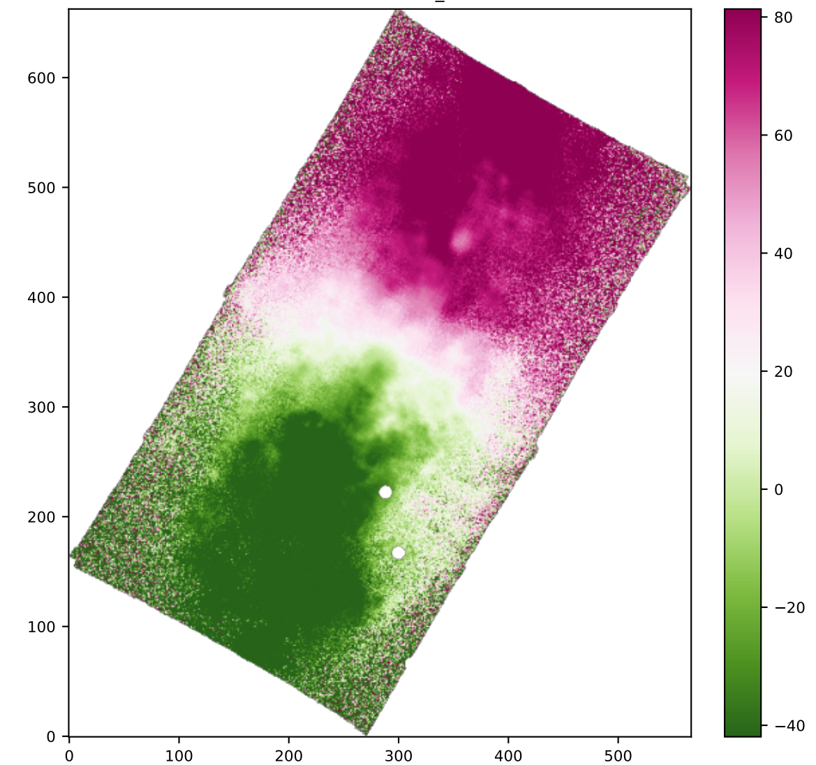
SPAXELS NII6583_VEL
