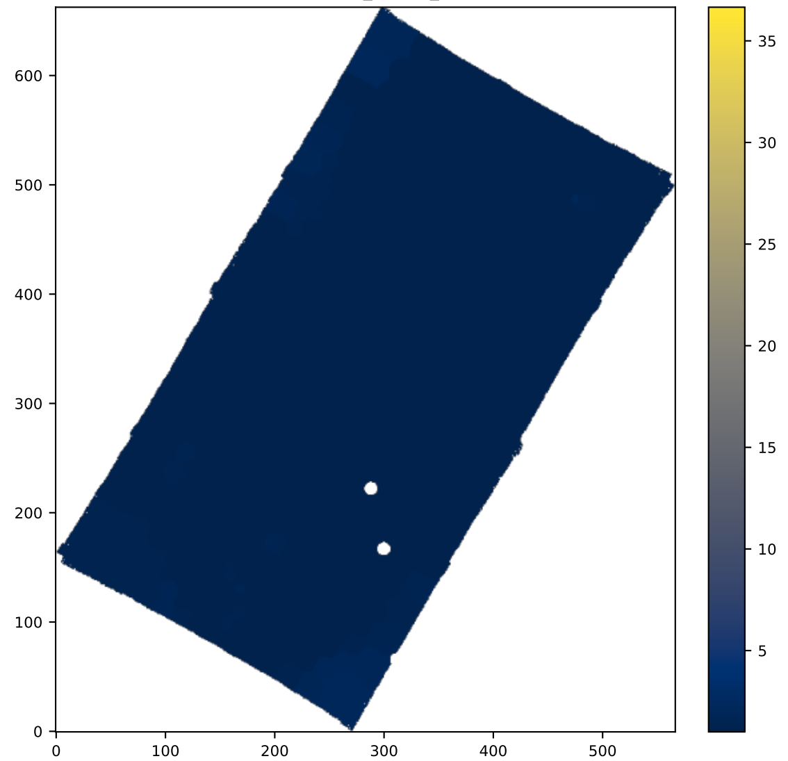
BIN HB4861_SIGMA_ERR
