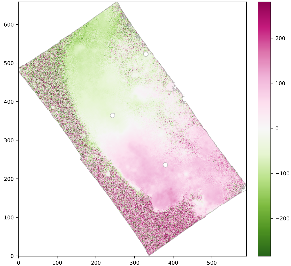
SPAXELS HA6562_VEL
