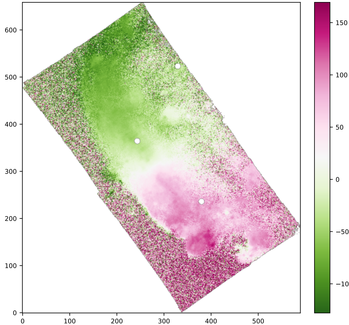
SPAXELS NII6583_VEL
