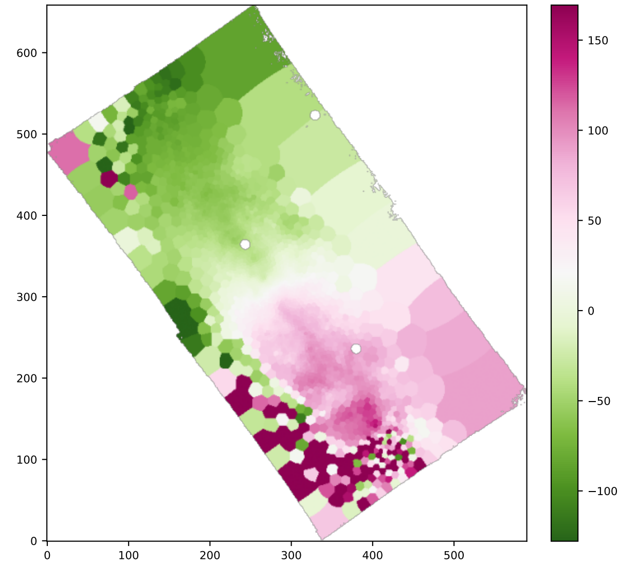
BIN OI6363_VEL
