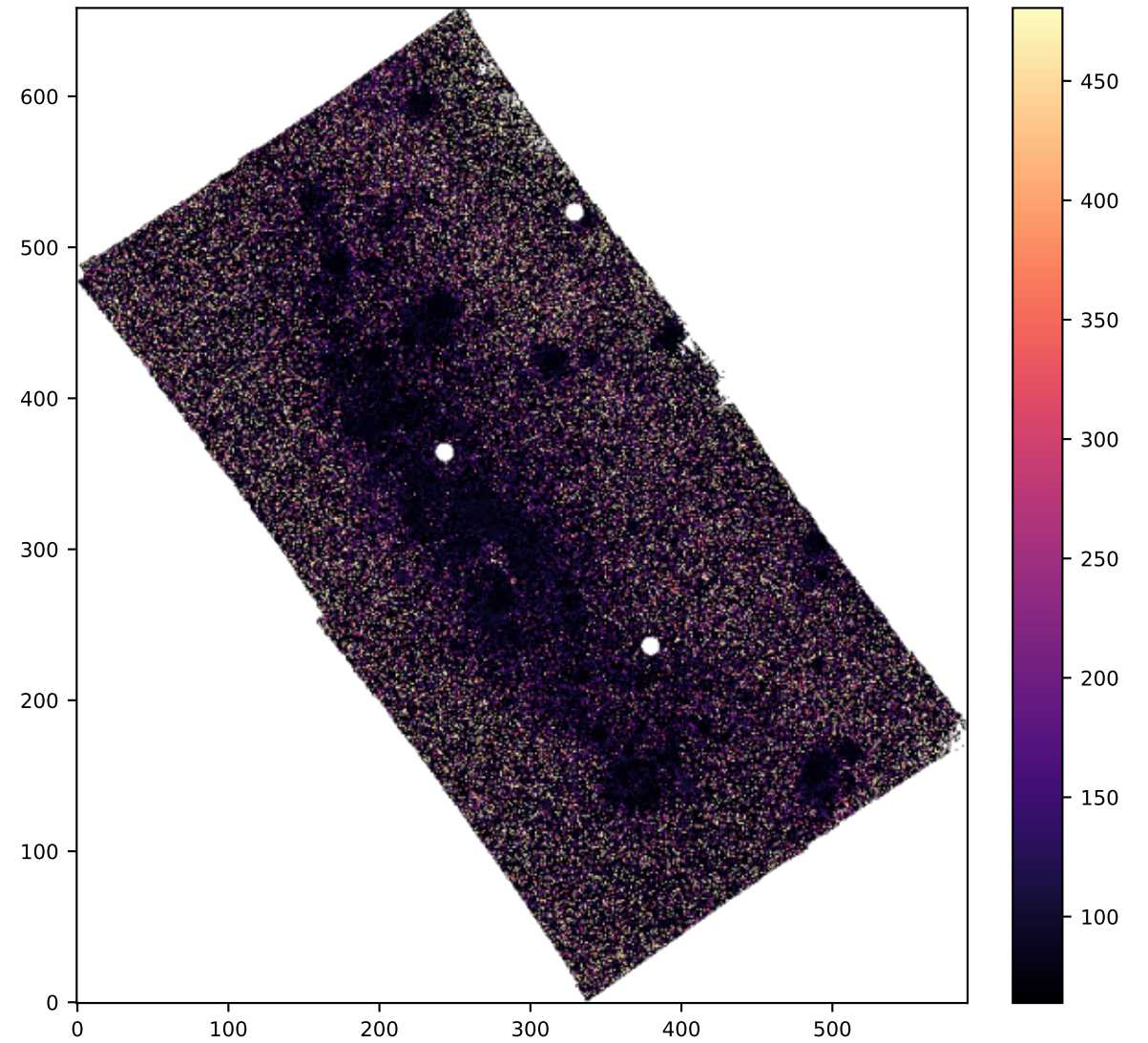
SPAXELS OIII5006_SIGMA
