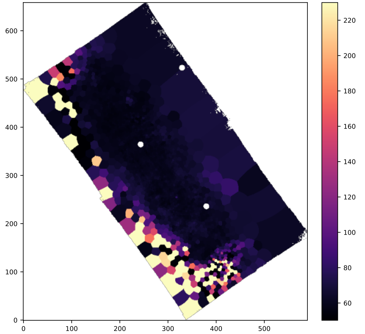
BIN OI6363_SIGMA
