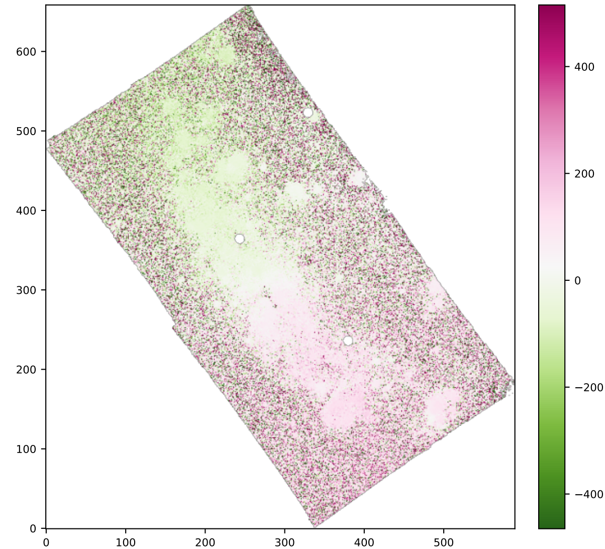
SPAXELS OIII5006_VEL
