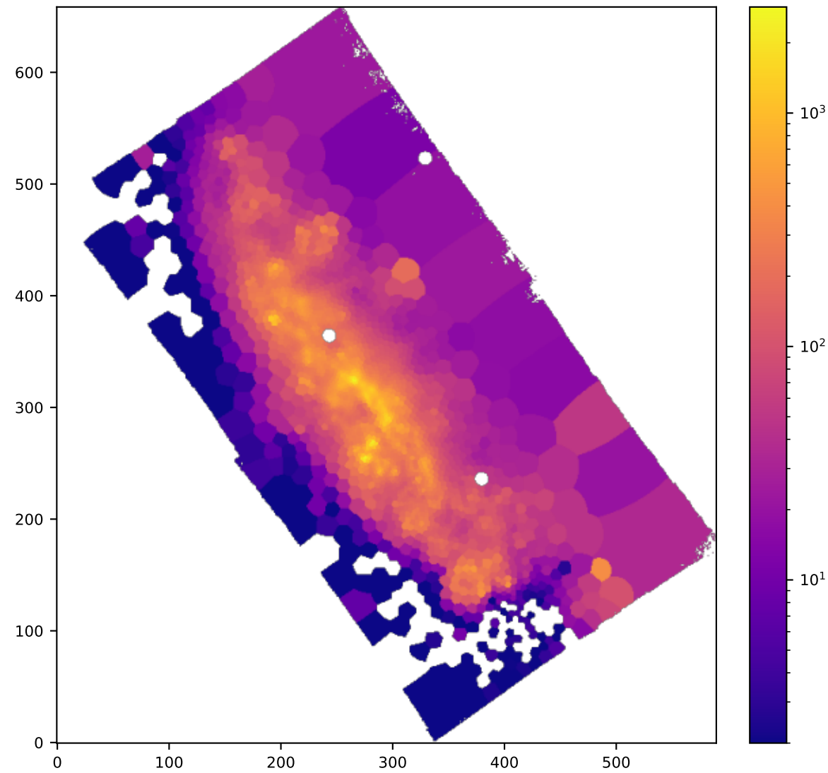
BIN SII6716_SIGMA
