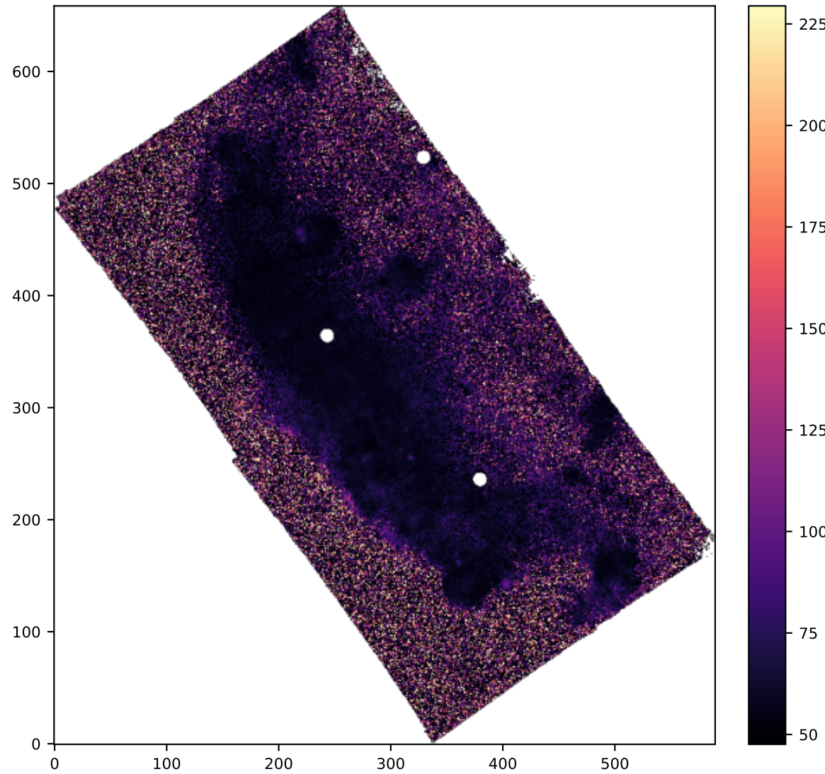
SPAXELS SII6716_SIGMA
