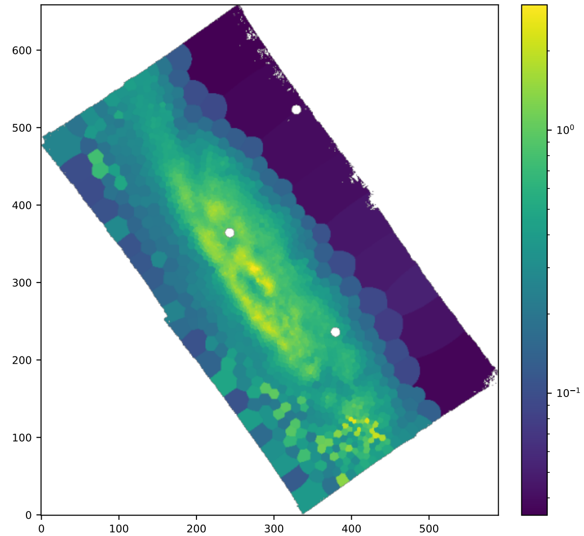
BIN OI6363_SIGMA_ERR
