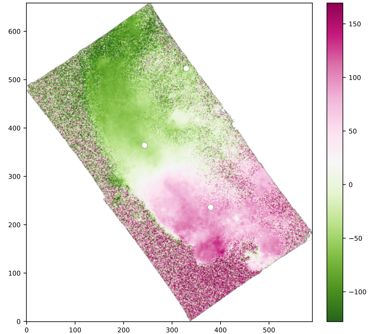
SPAXELS OI6363_VEL
