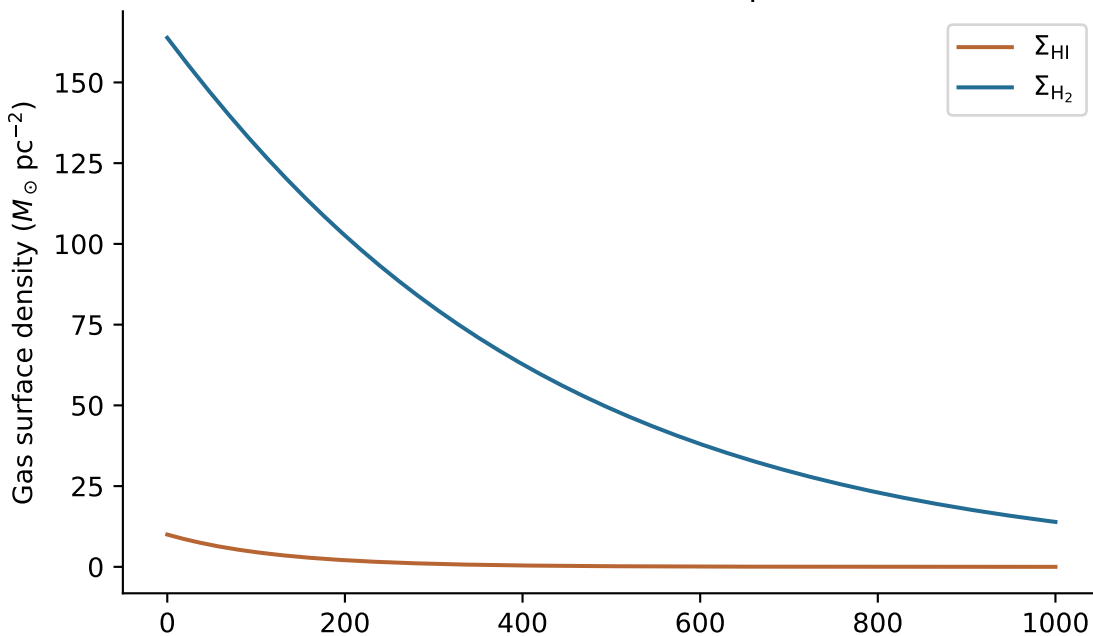
Negative = instantaneously rising SFR
