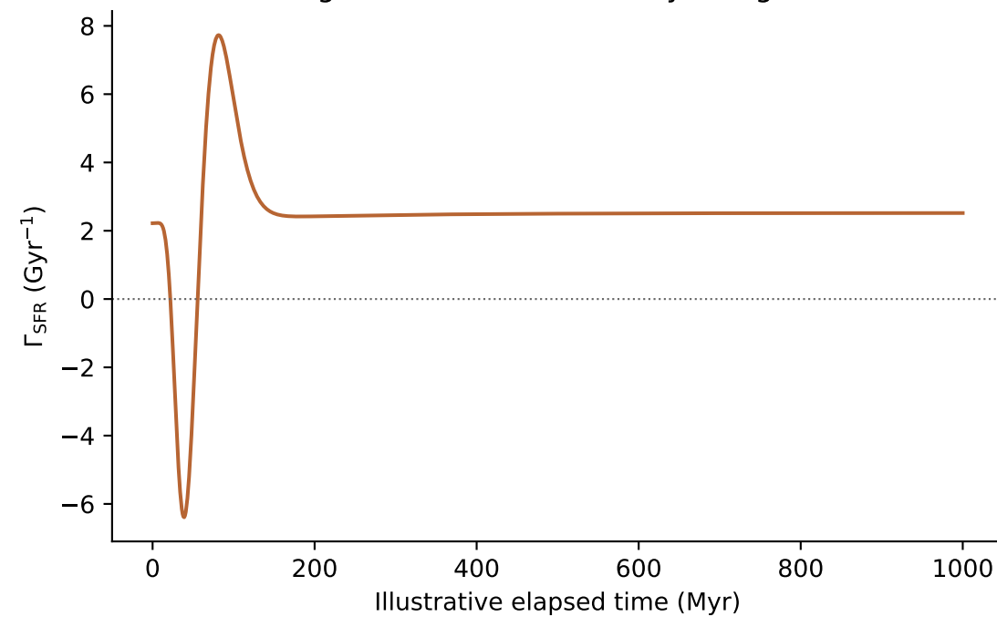
Negative = instantaneously rising SFR
