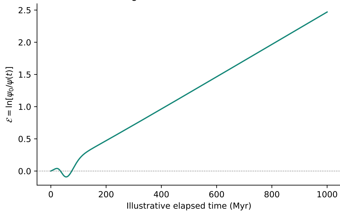
Negative = above initial SFR
