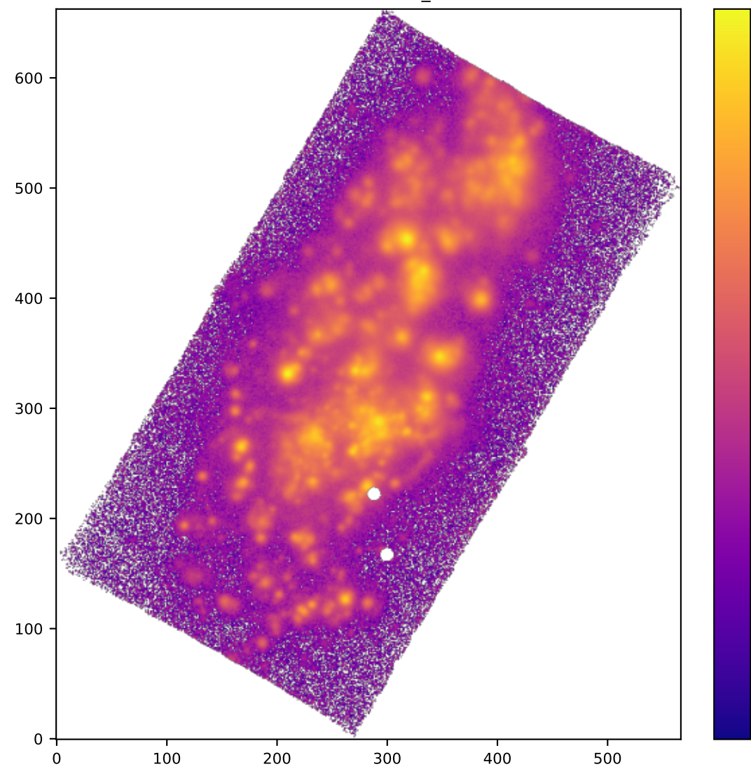
SPAXELS OIII5006_SIGMA
