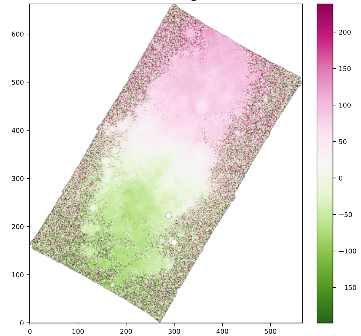
SPAXELS OIII5006_VEL
