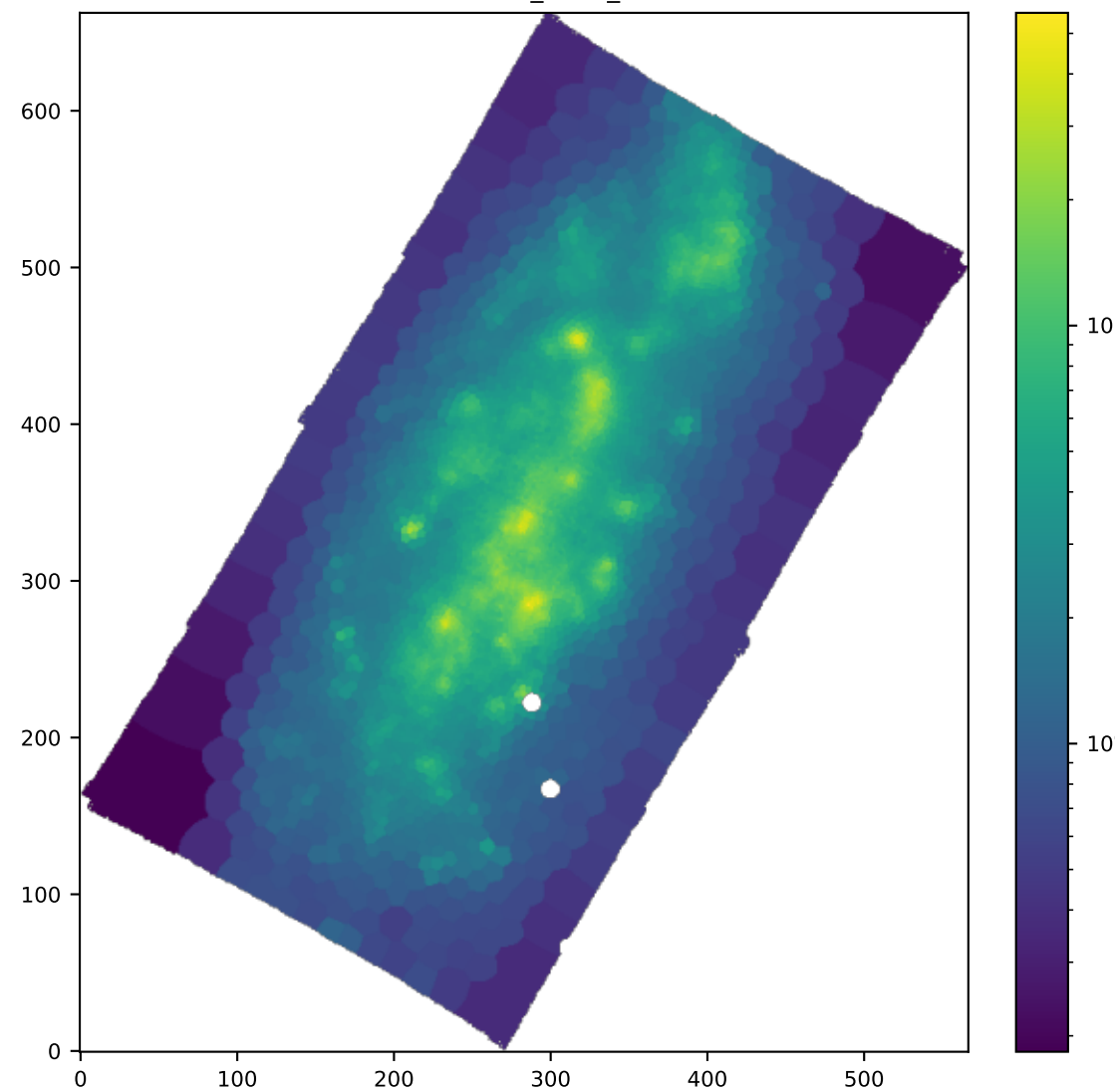
BIN HB4861_SIGMA_ERR
