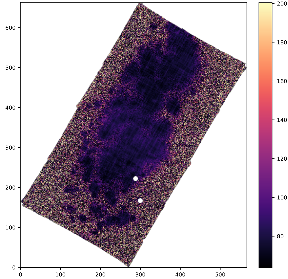
SPAXELS OIII5006_SIGMA
