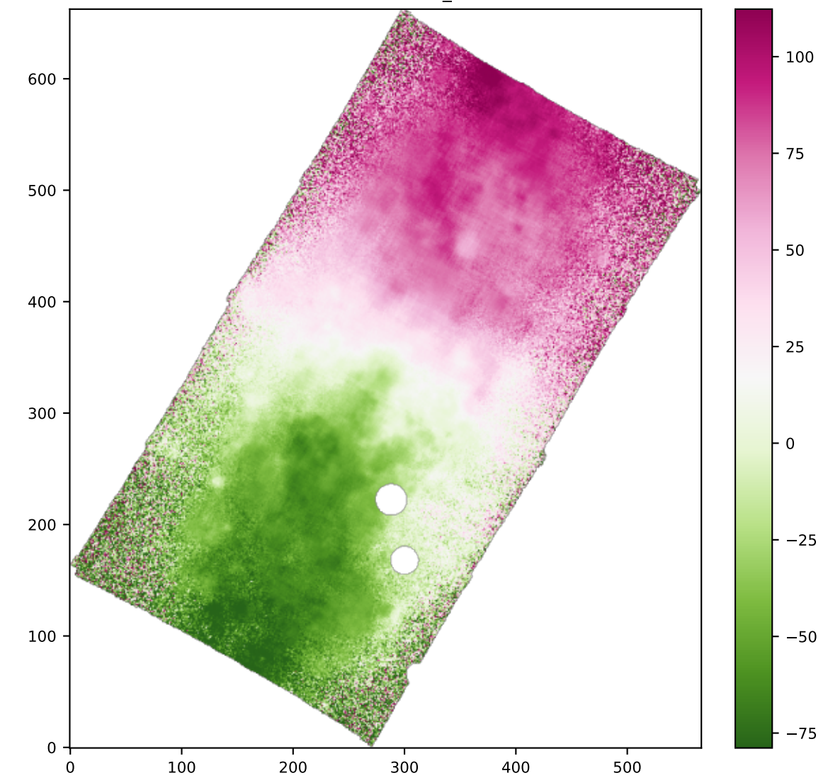
SPAXELS HA6562_VEL
