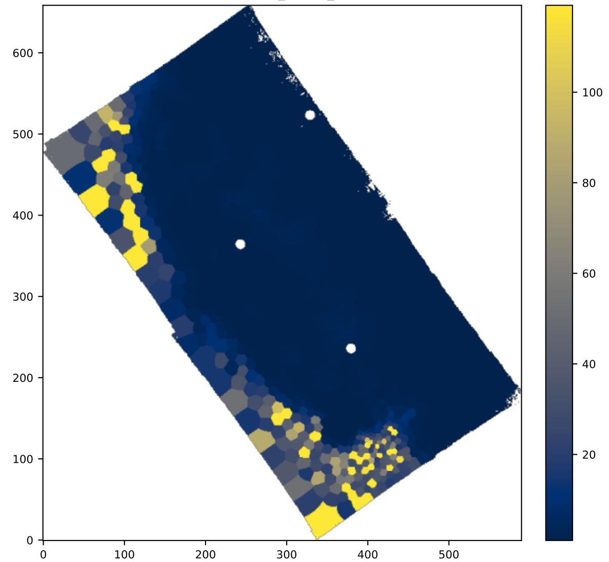
BIN OI6363_SIGMA_ERR
