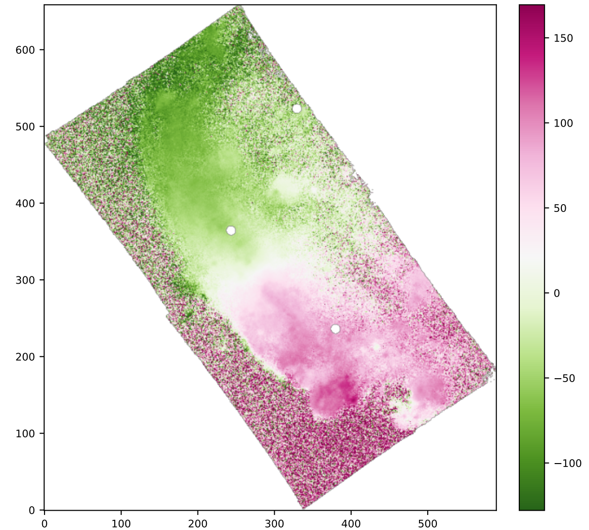
SPAXELS OI6300_VEL
