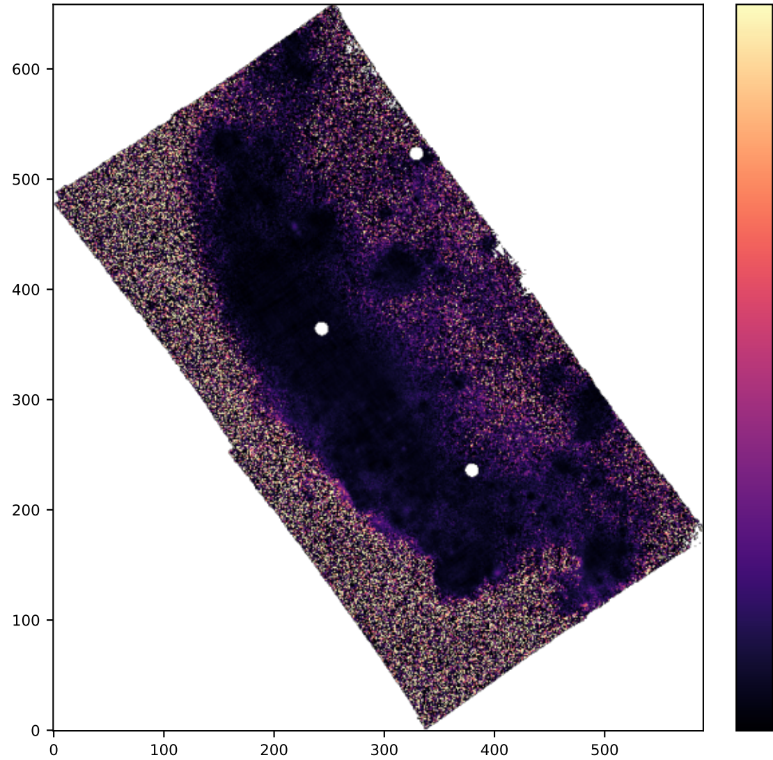
SPAXELS HB4861_SIGMA
