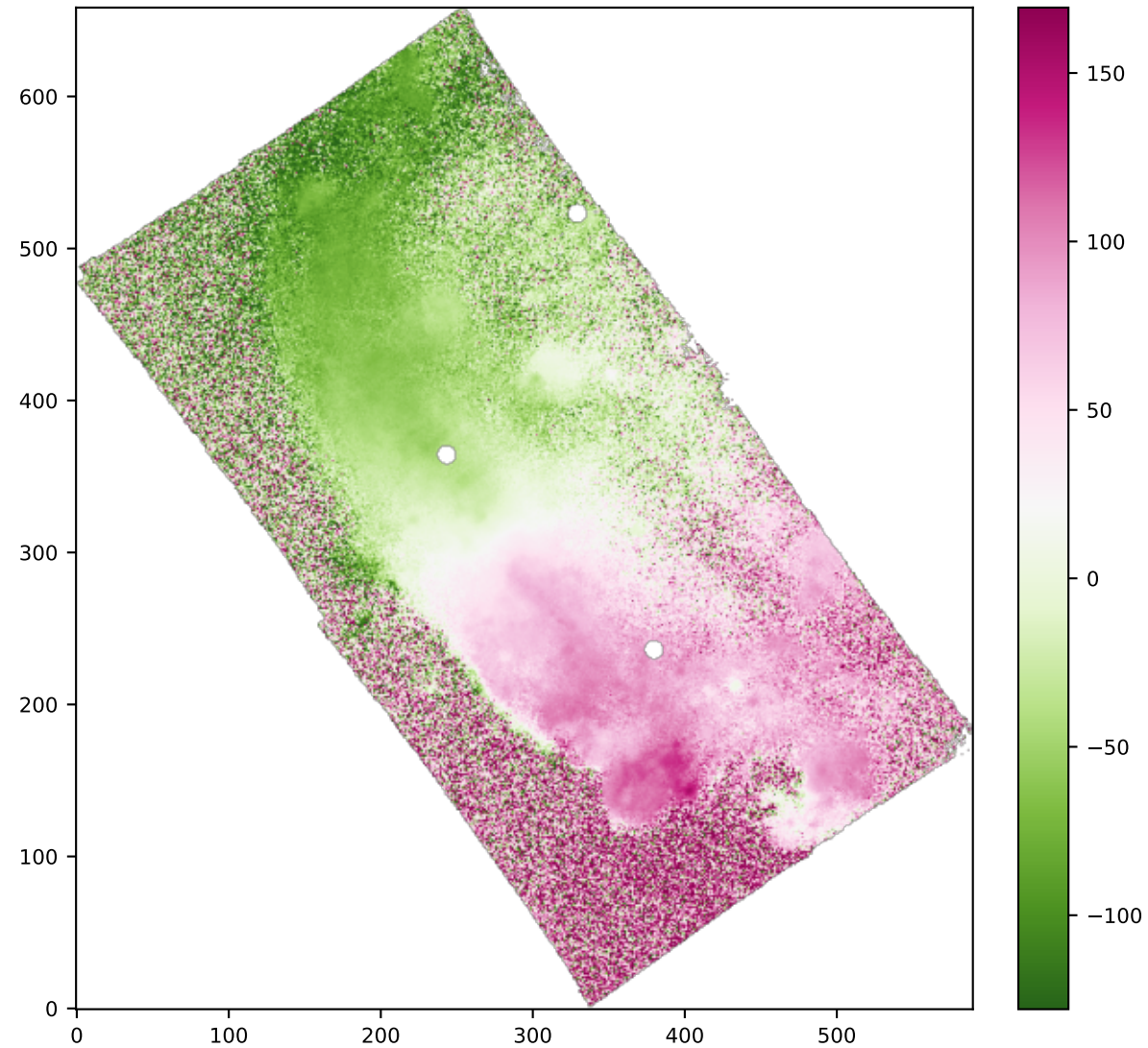
SPAXELS NII6583_VEL
