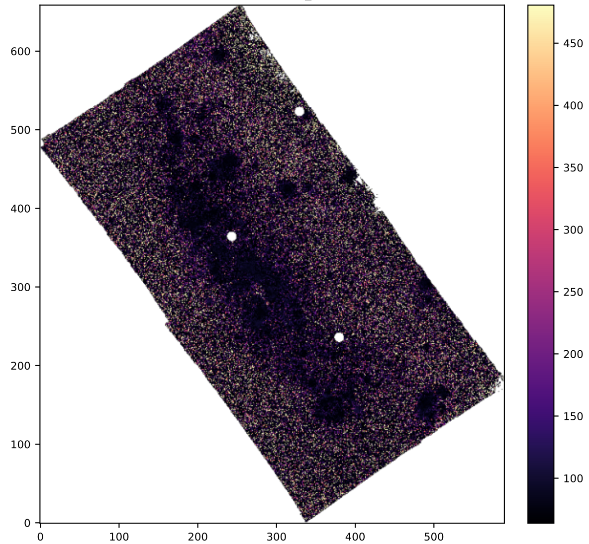
SPAXELS OIII5006_SIGMA
