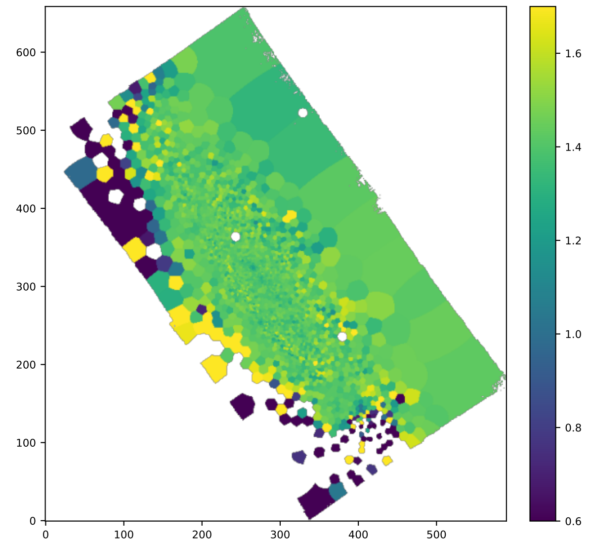
BIN SII6716/SII6730
