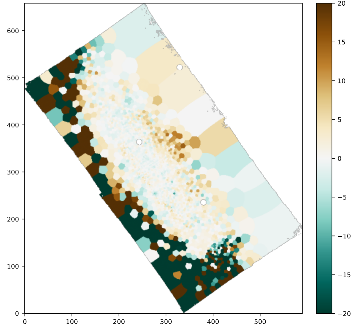
BIN SHa-SNII
