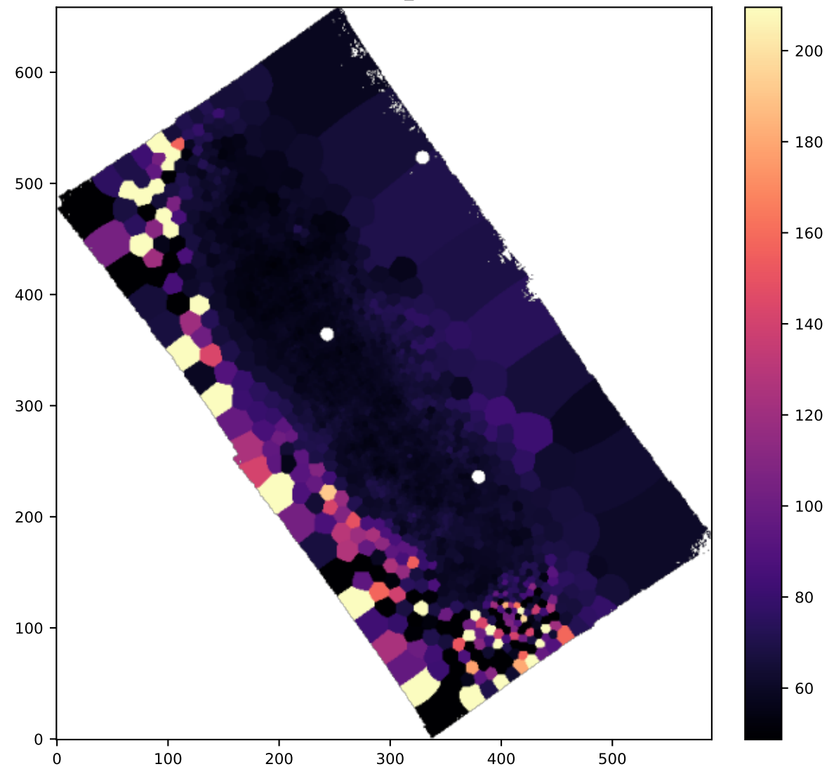
BIN HA6562_SIGMA
