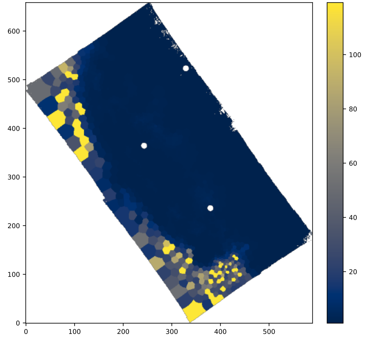
BIN SII6716_SIGMA_ERR
