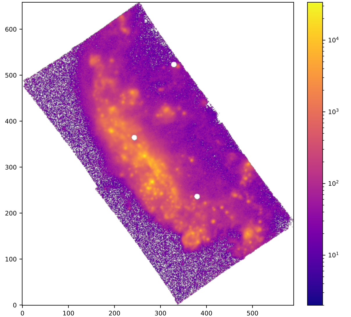
SPAXELS HA6562_SIGMA
