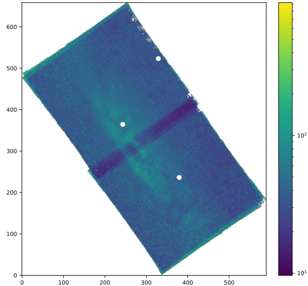
SPAXELS OI6300_SIGMA_ERR
