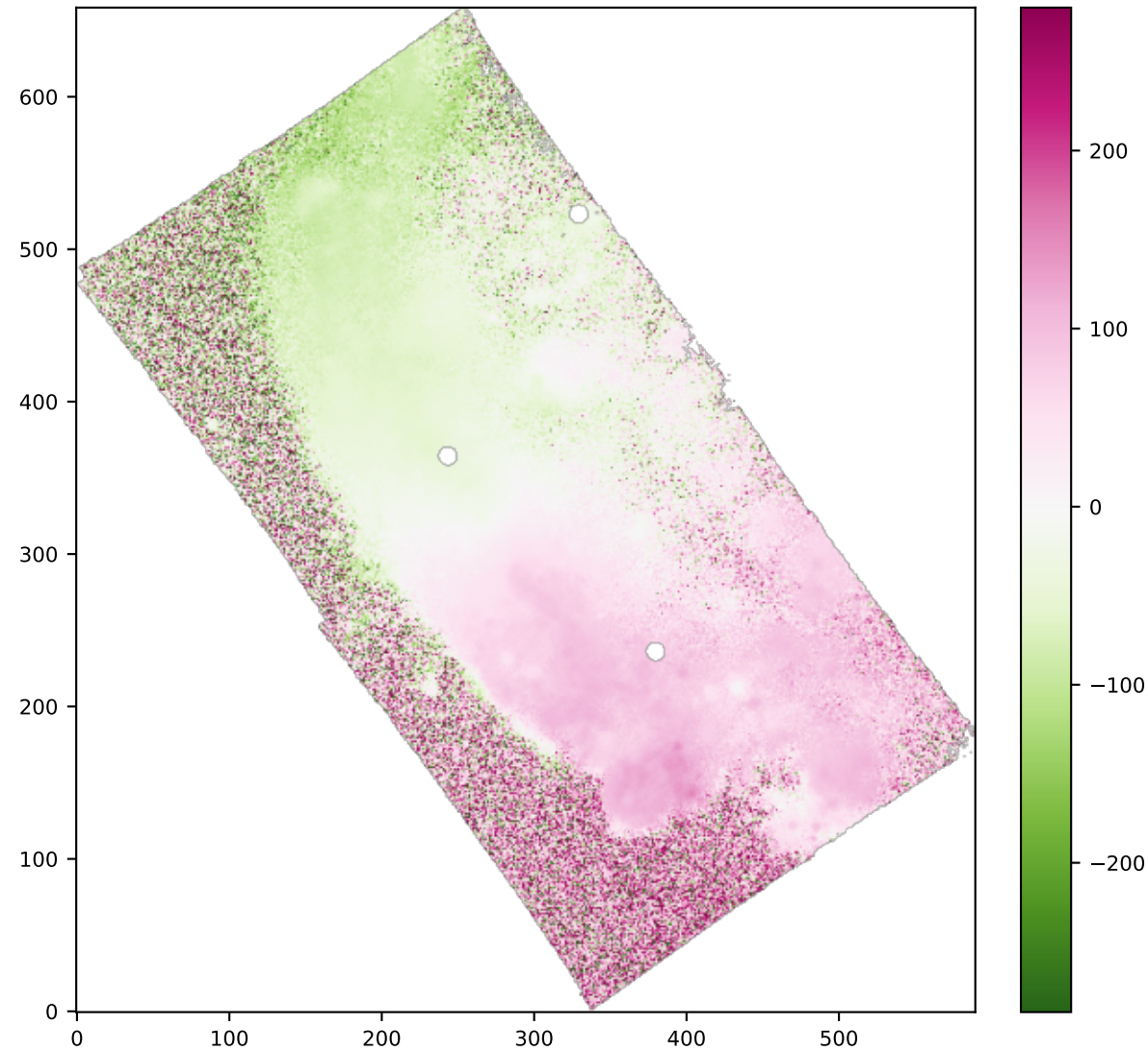
SPAXELS HB4861_VEL
