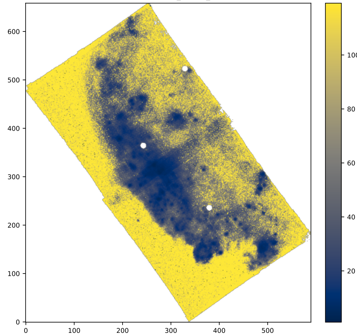
SPAXELS SII6716_SIGMA_ERR
