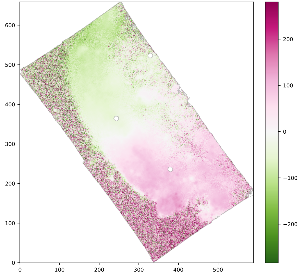
SPAXELS HA6562_VEL
