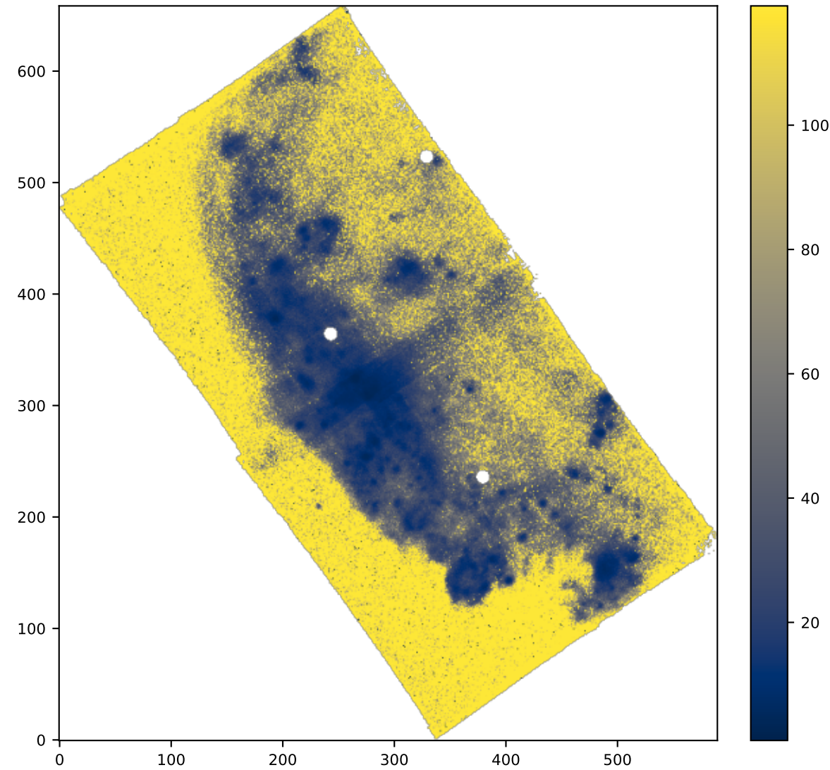
SPAXELS OI6363_SIGMA_ERR
