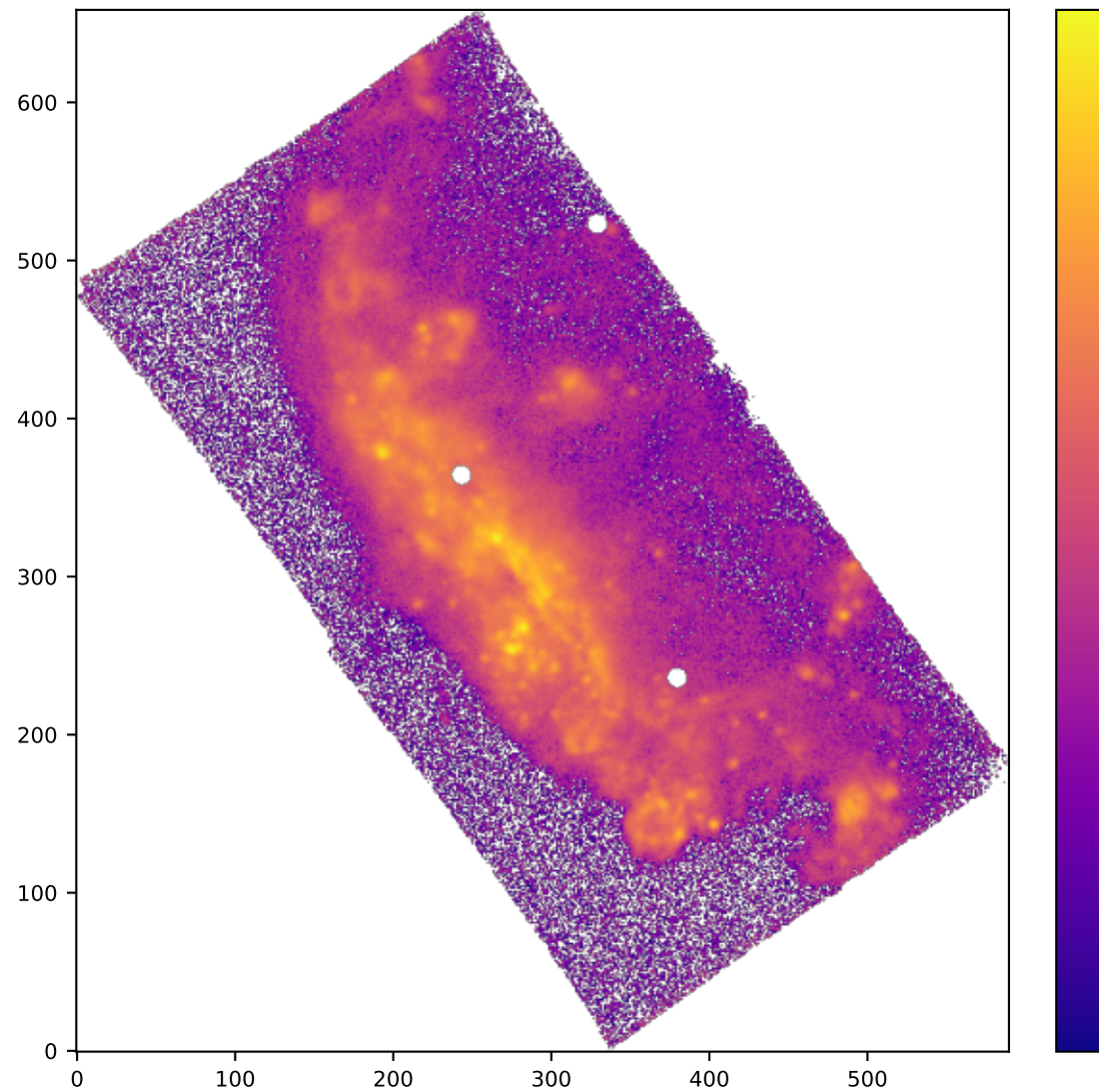
SPAXELS SII6716_SIGMA
