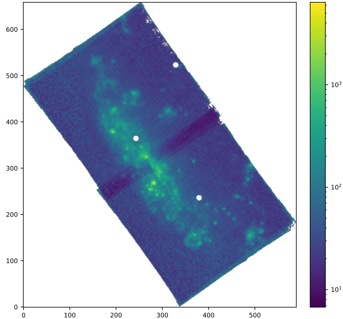
SPAXELS HA6562_SIGMA_ERR
