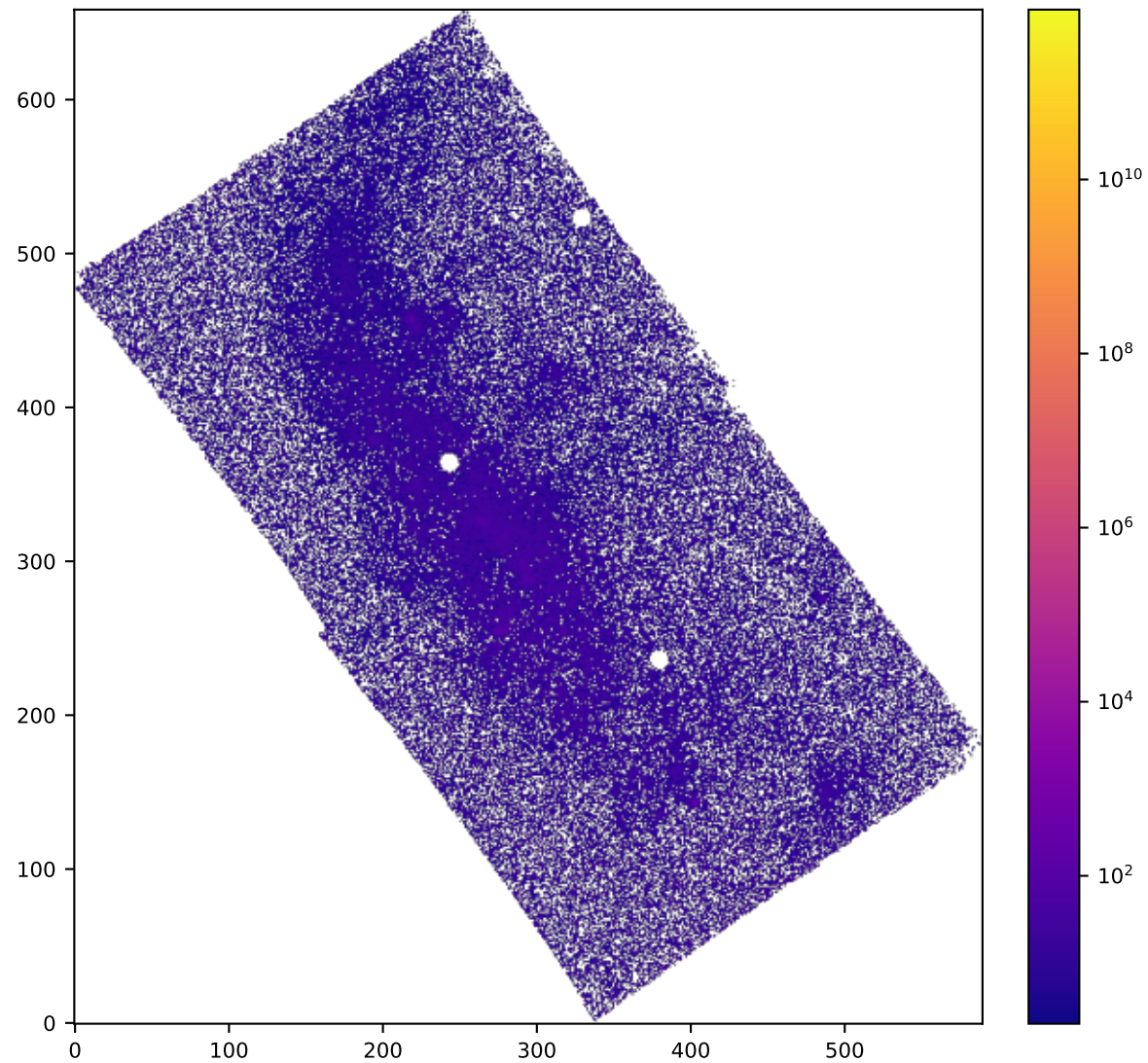
SPAXELS OI6363_SIGMA
