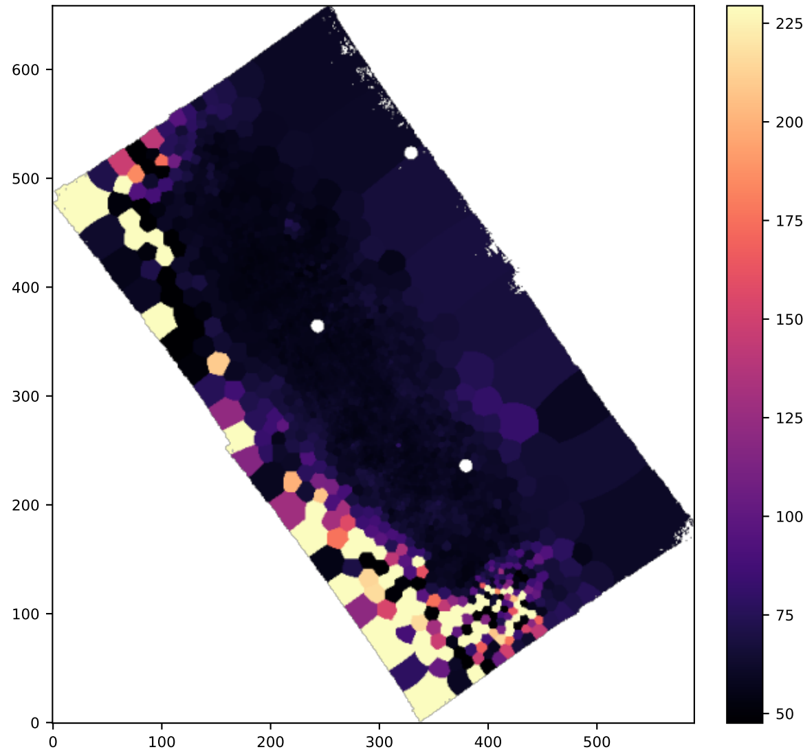
BIN SII6716_SIGMA
