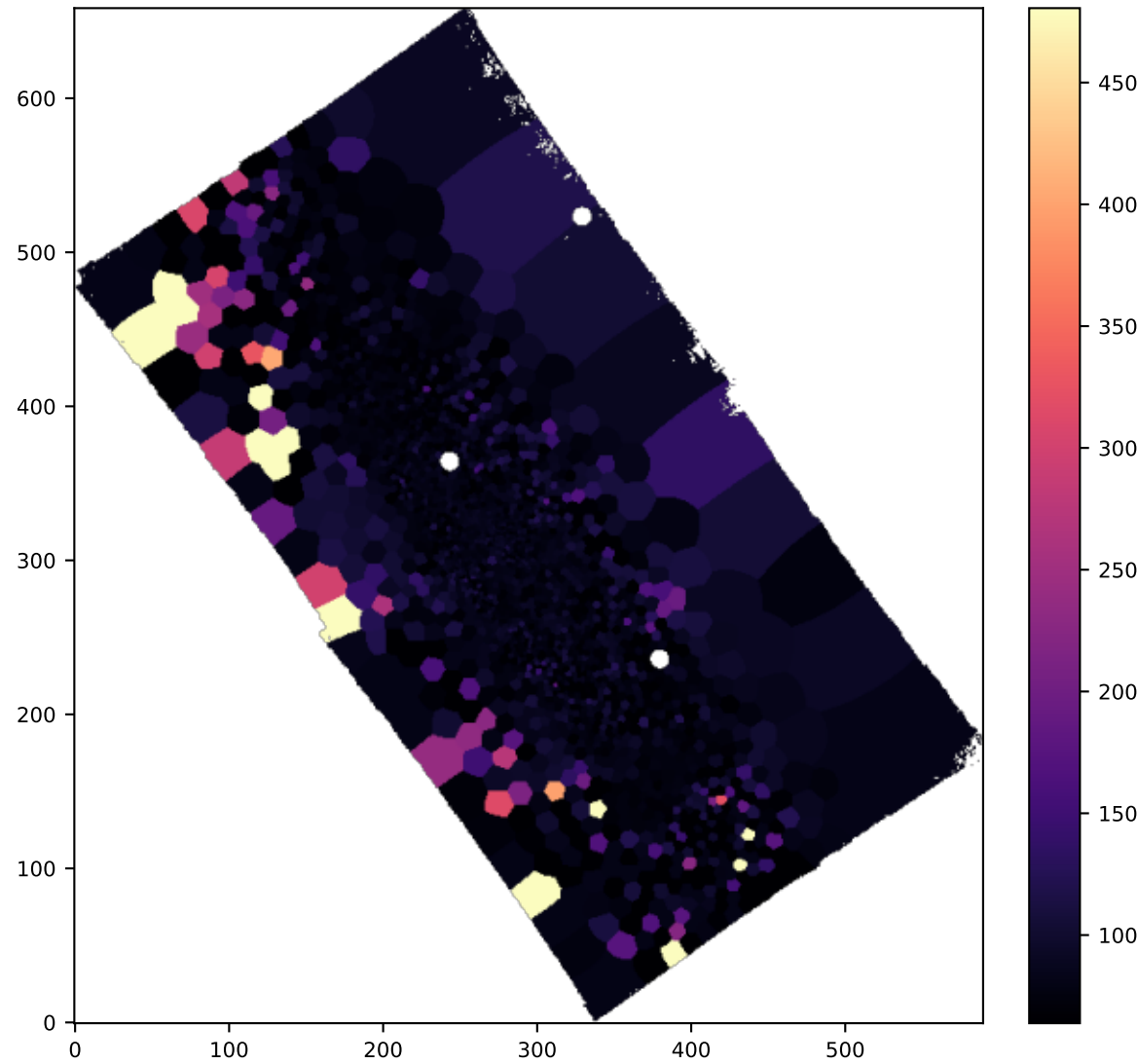
BIN OIII5006_SIGMA
