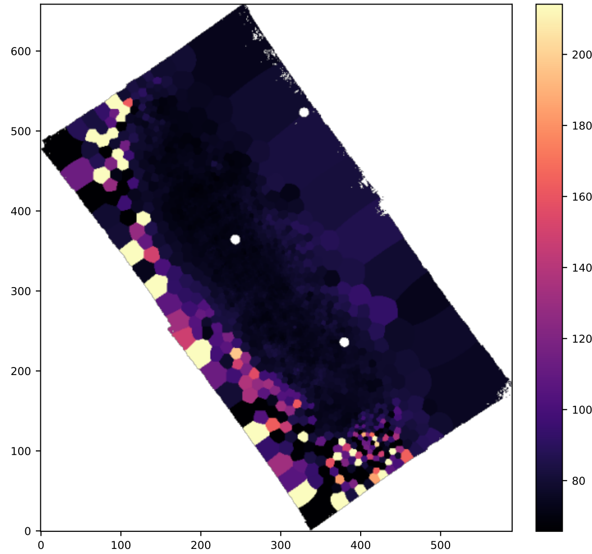
BIN HB4861_SIGMA
