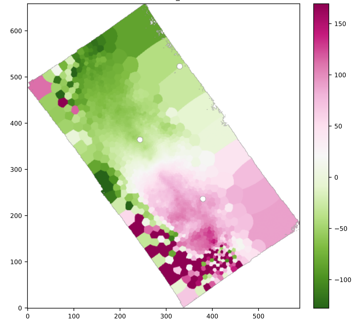
BIN OI6300_VEL
