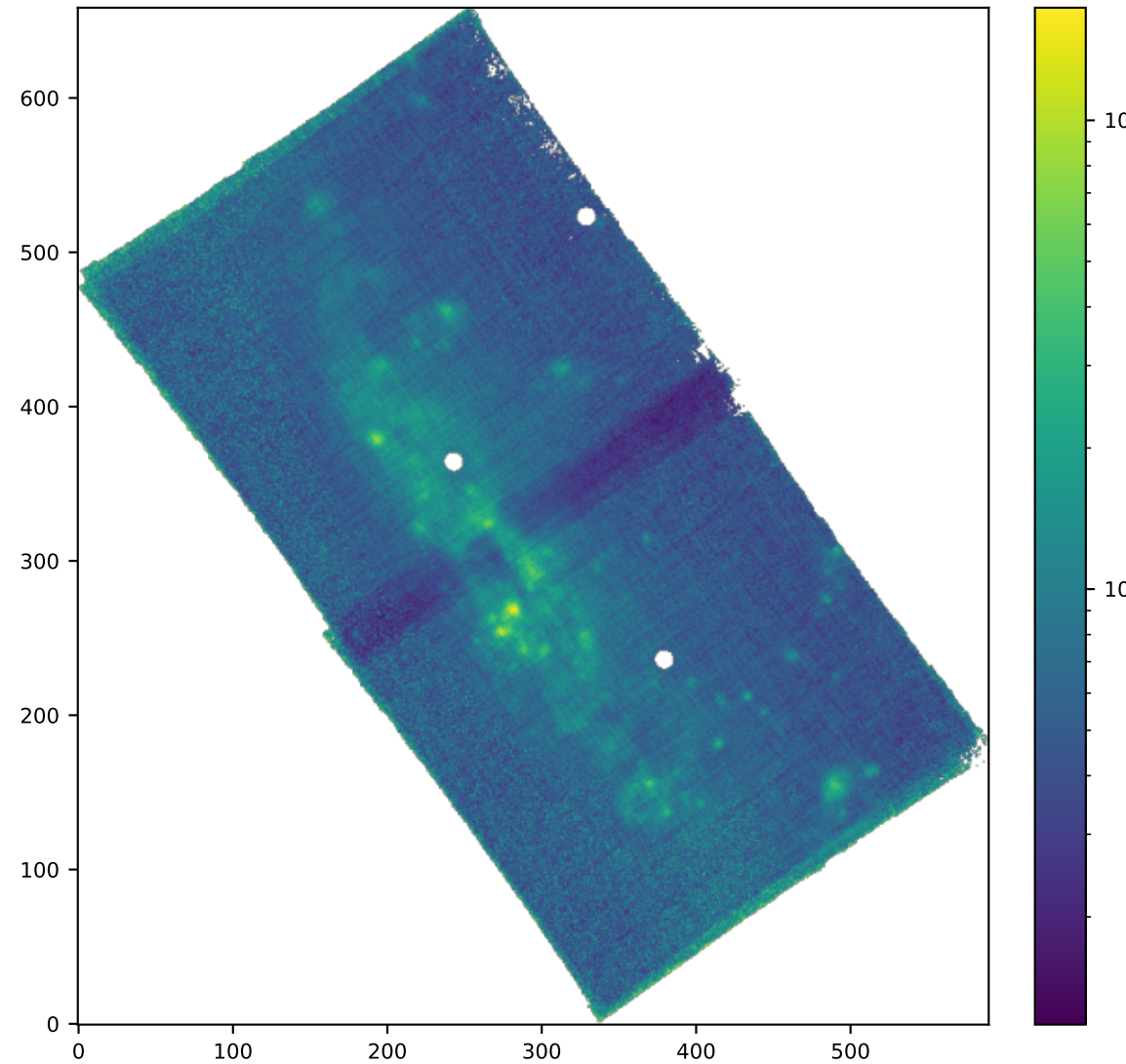
SPAXELS HB4861_SIGMA_ERR
