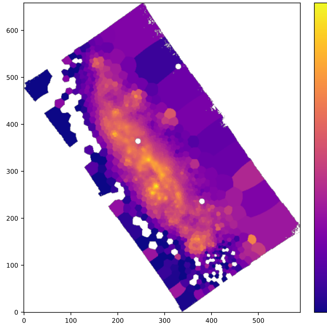
BIN HB4861_SIGMA
