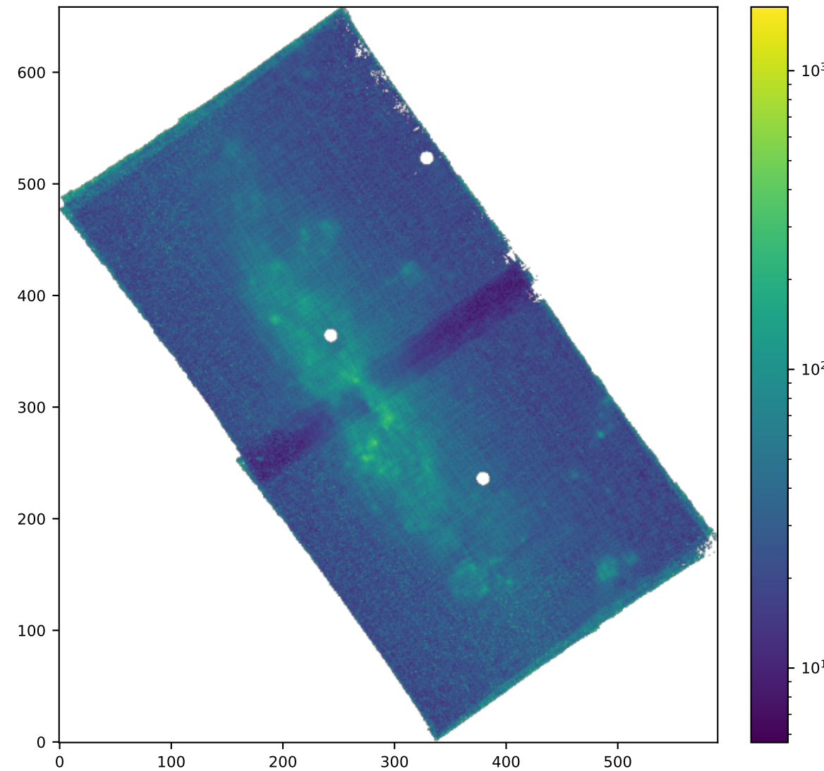
SPAXELS SII6716_SIGMA_ERR
