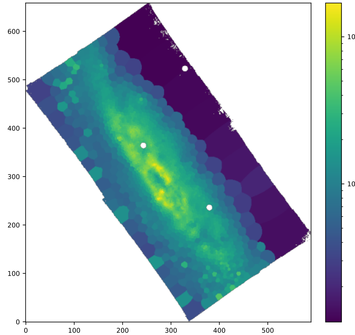
BIN HB4861_SIGMA_ERR
