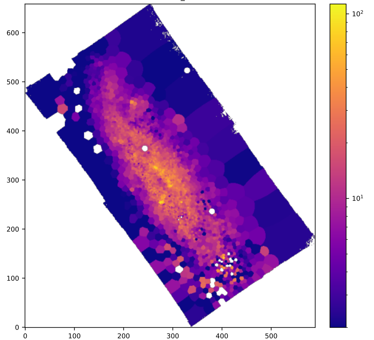
BIN OI6363_SIGMA
