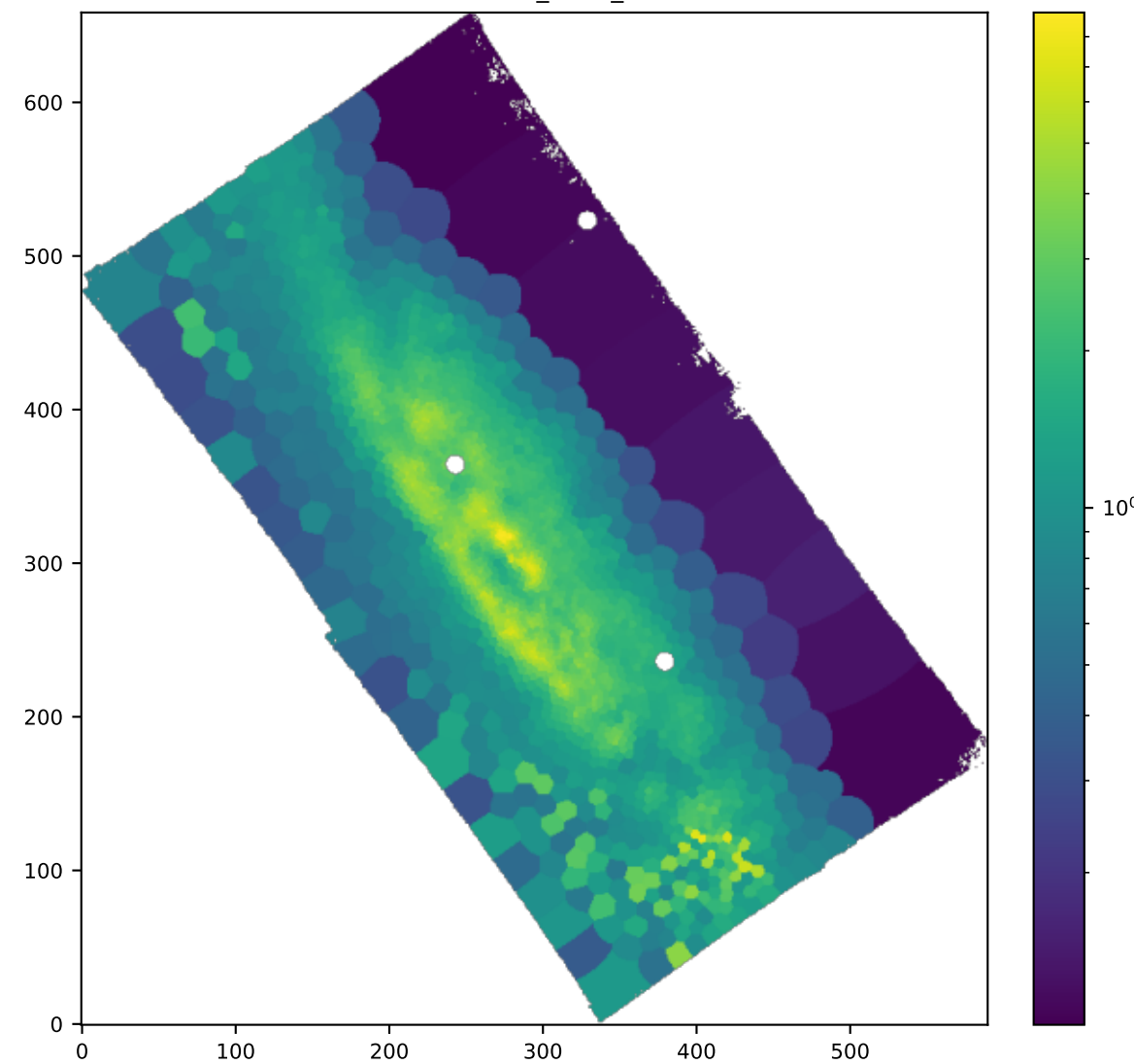
BIN OI6300_SIGMA_ERR
