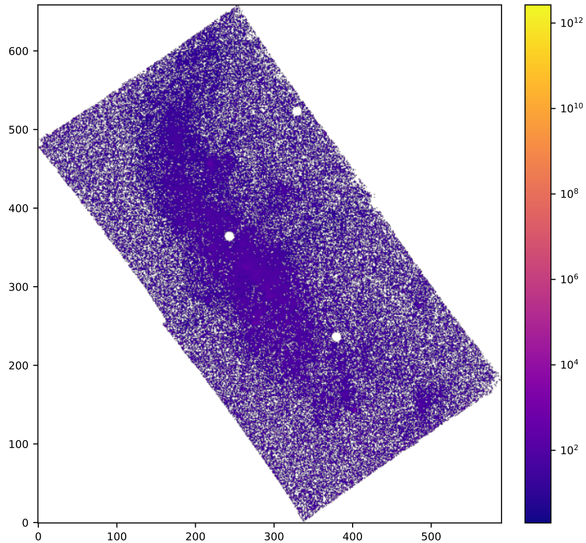
SPAXELS OI6300_SIGMA
