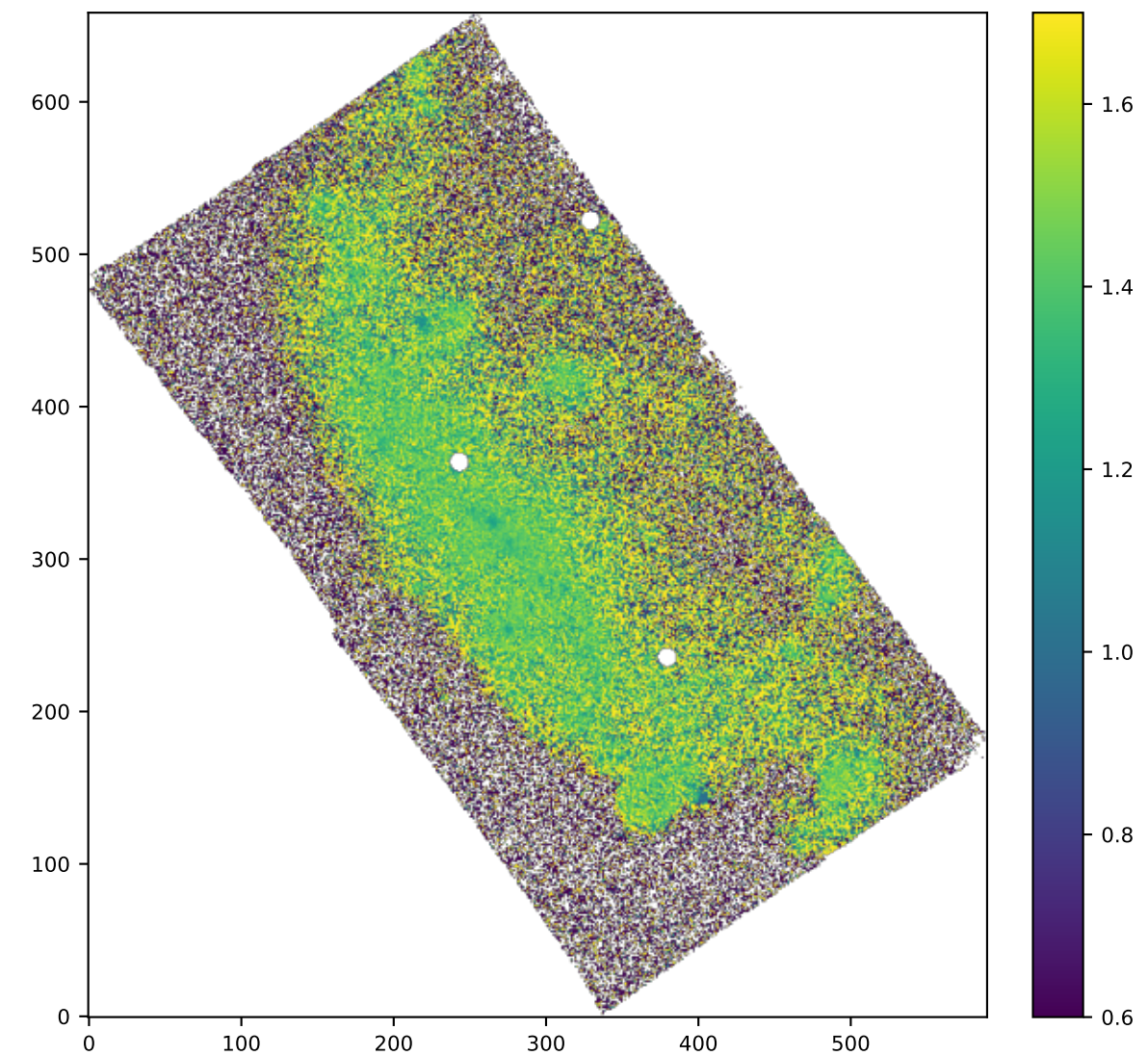
SPAXELS SII6716/SII6730
