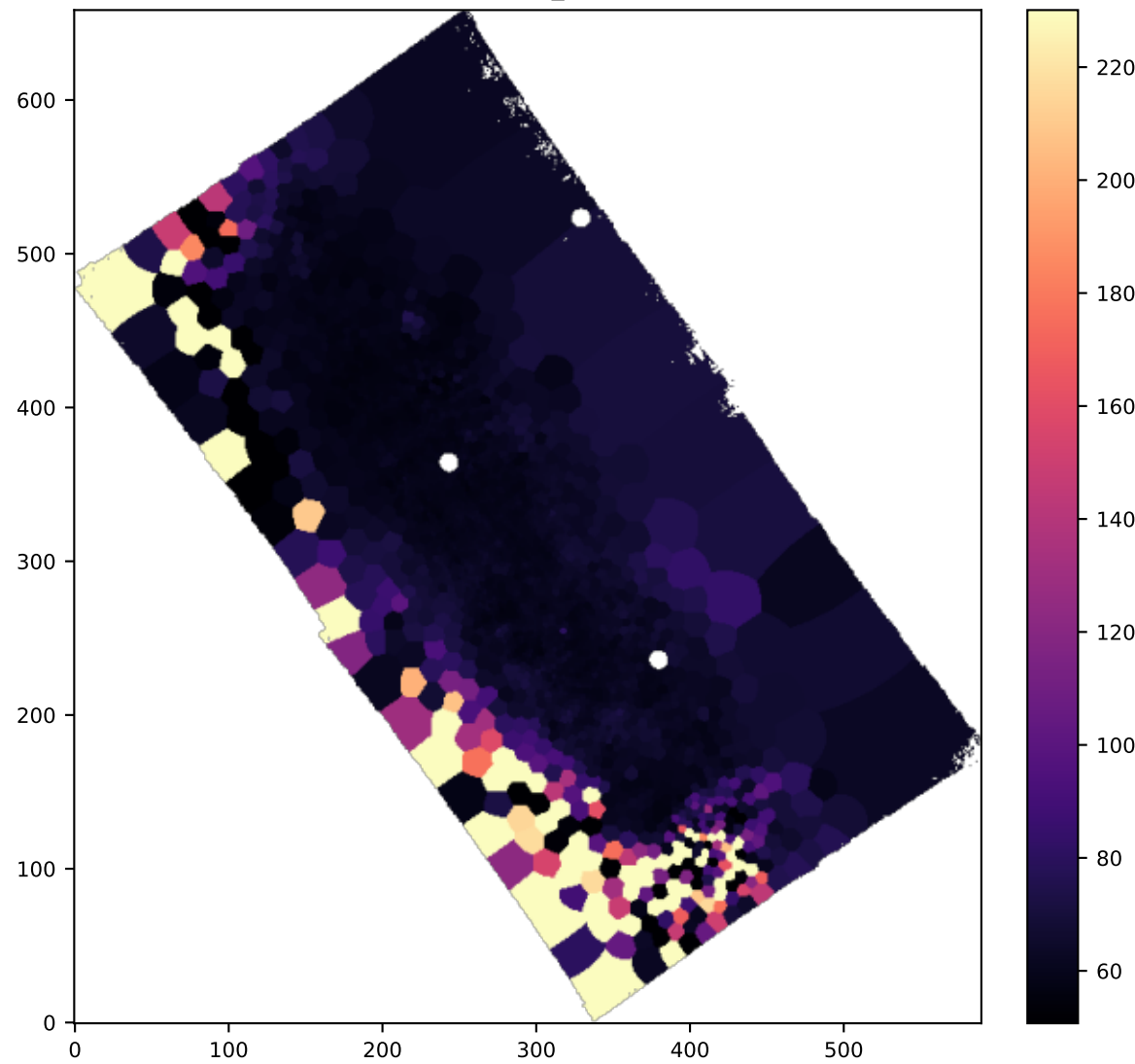
BIN OI6300_SIGMA
