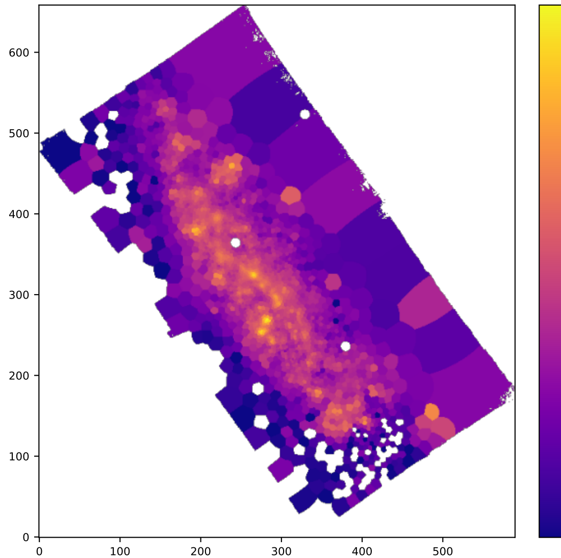
BIN OIII5006_SIGMA
