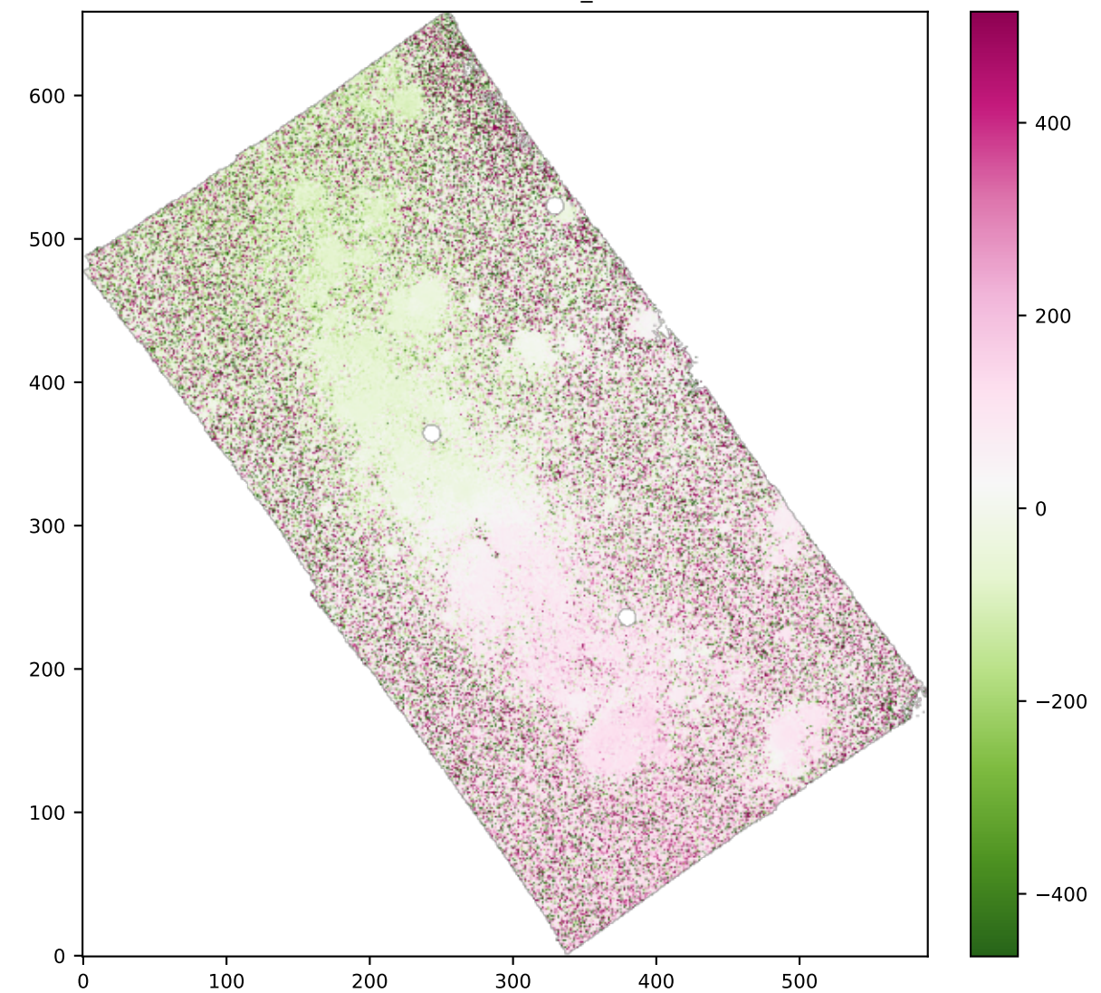
SPAXELS OIII5006_VEL
