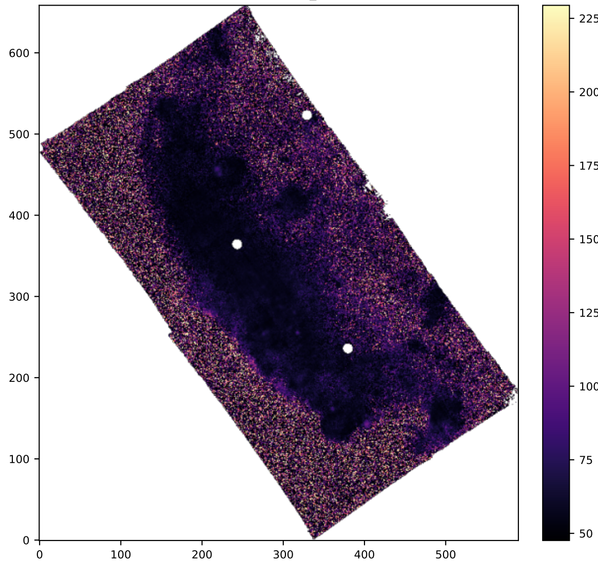
SPAXELS SII6716_SIGMA
