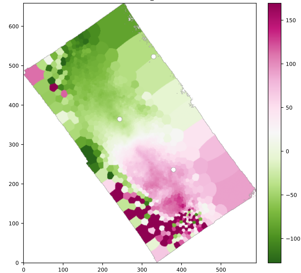
BIN OI6363_VEL
