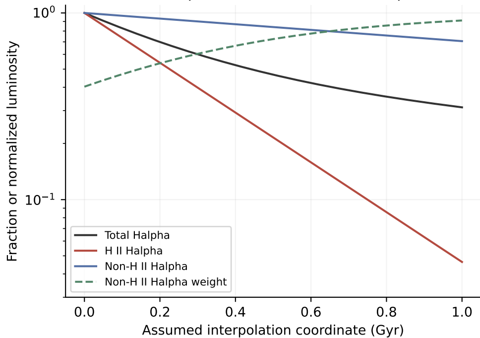
NSF H \alpha + NII-calibrated example
