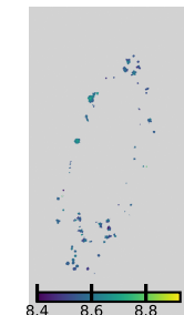
[O/H] (O3N2-M13, HII)
