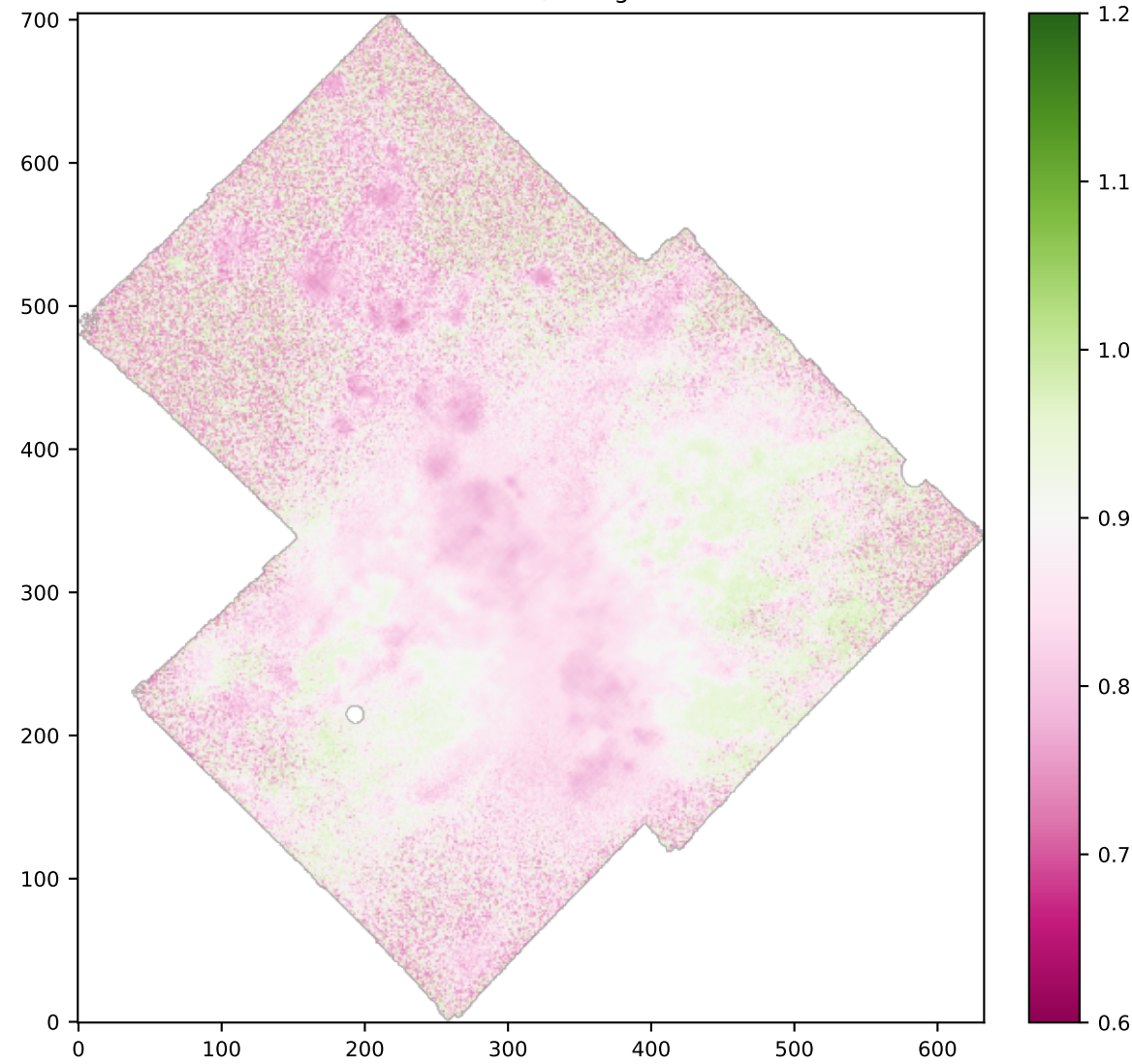
SPAXELS Ha/Hb sigma
