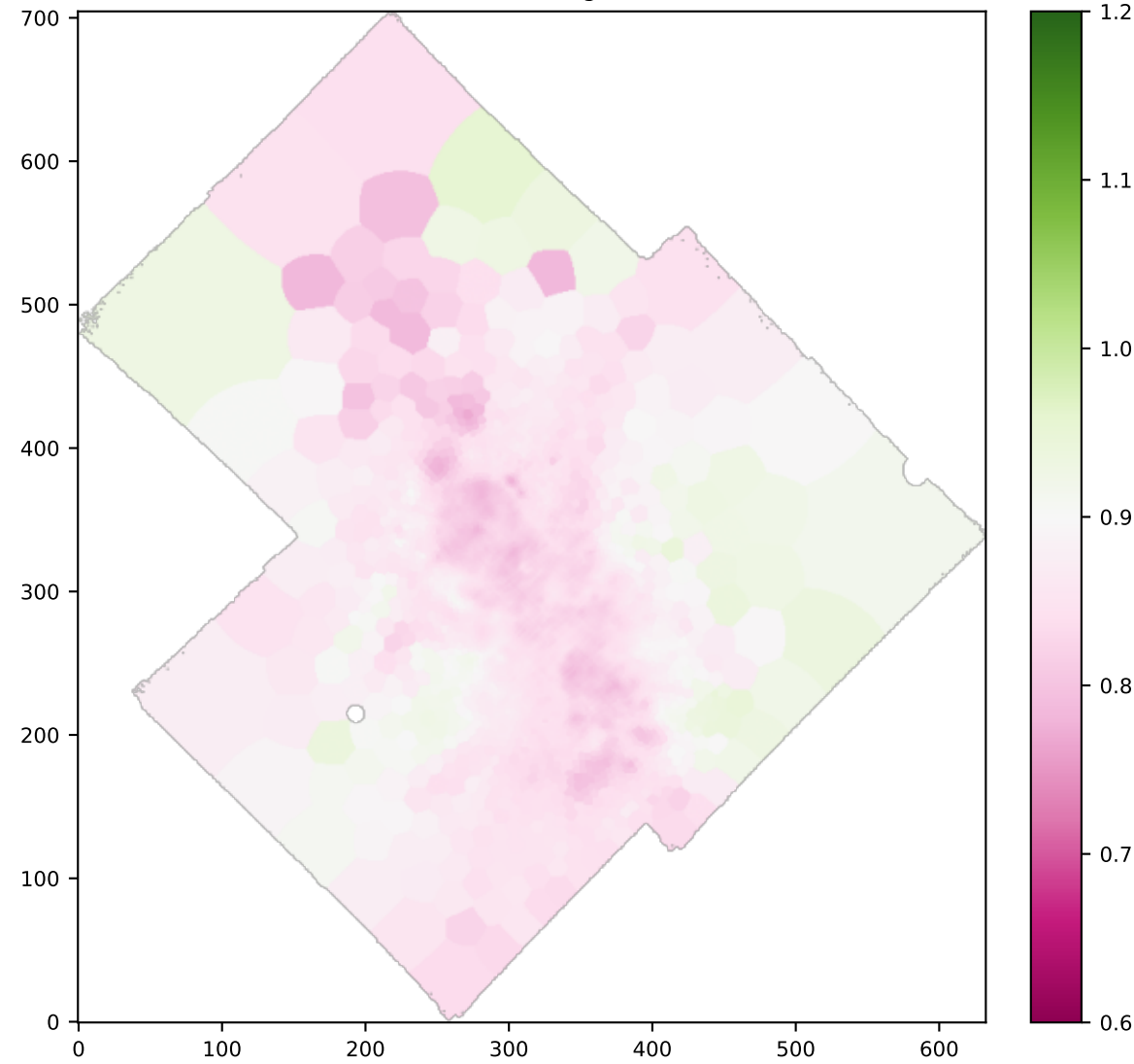
BIN Ha/Hb sigma
