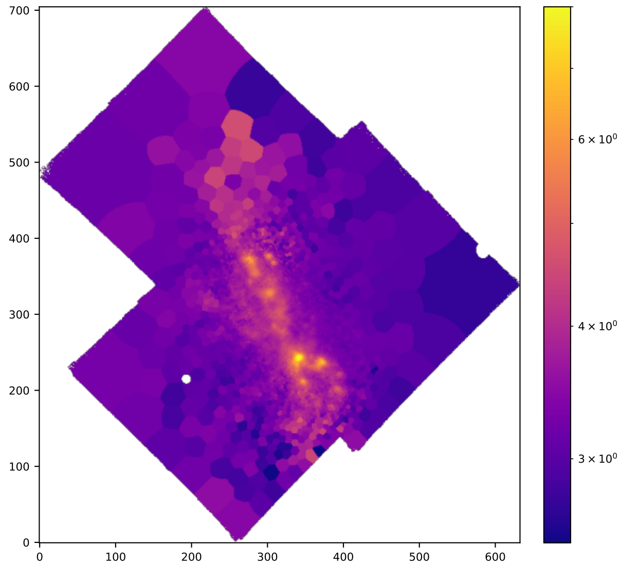
BIN Ha-Hb vel
