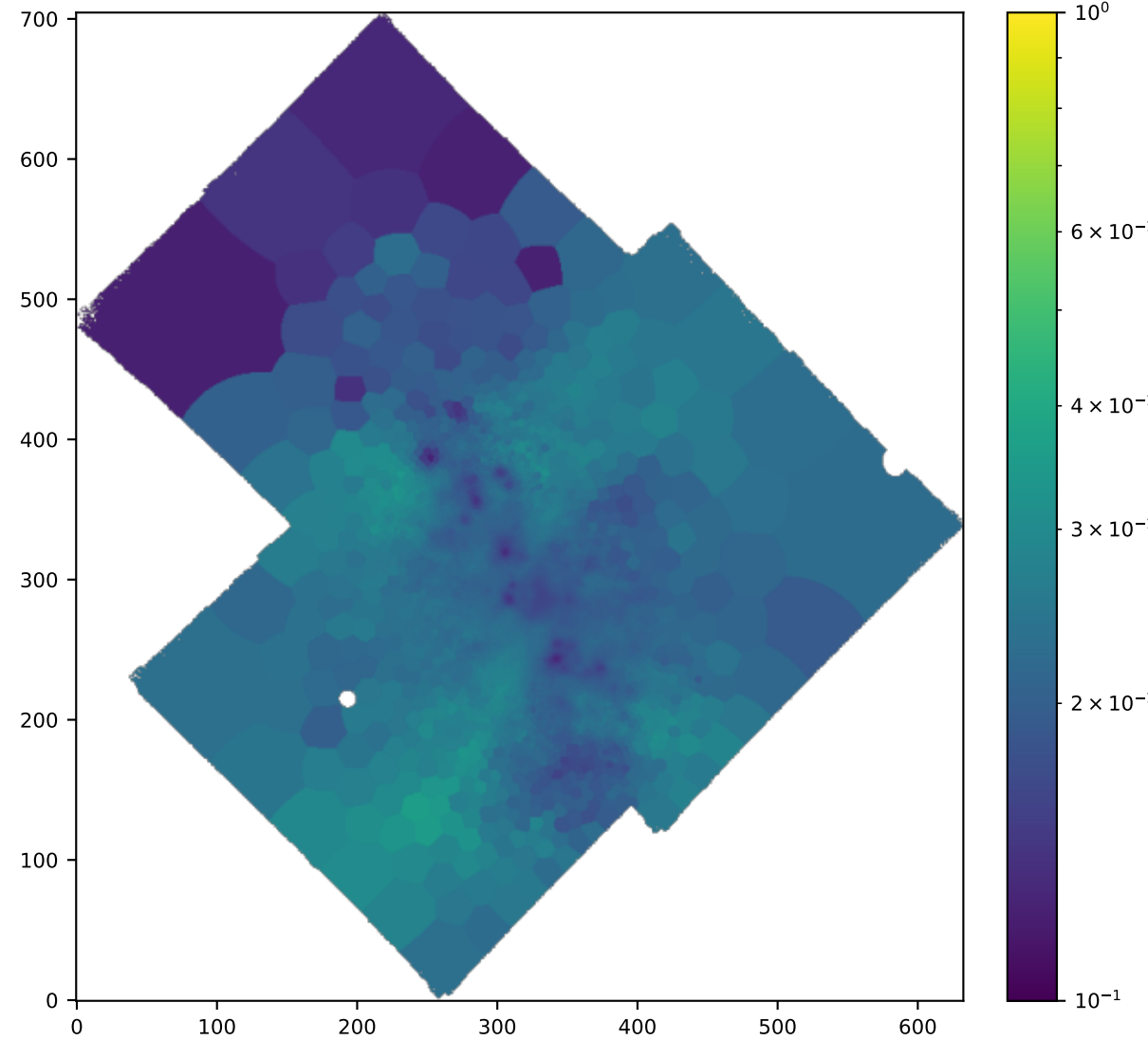
BIN Ha/Hb sigma
