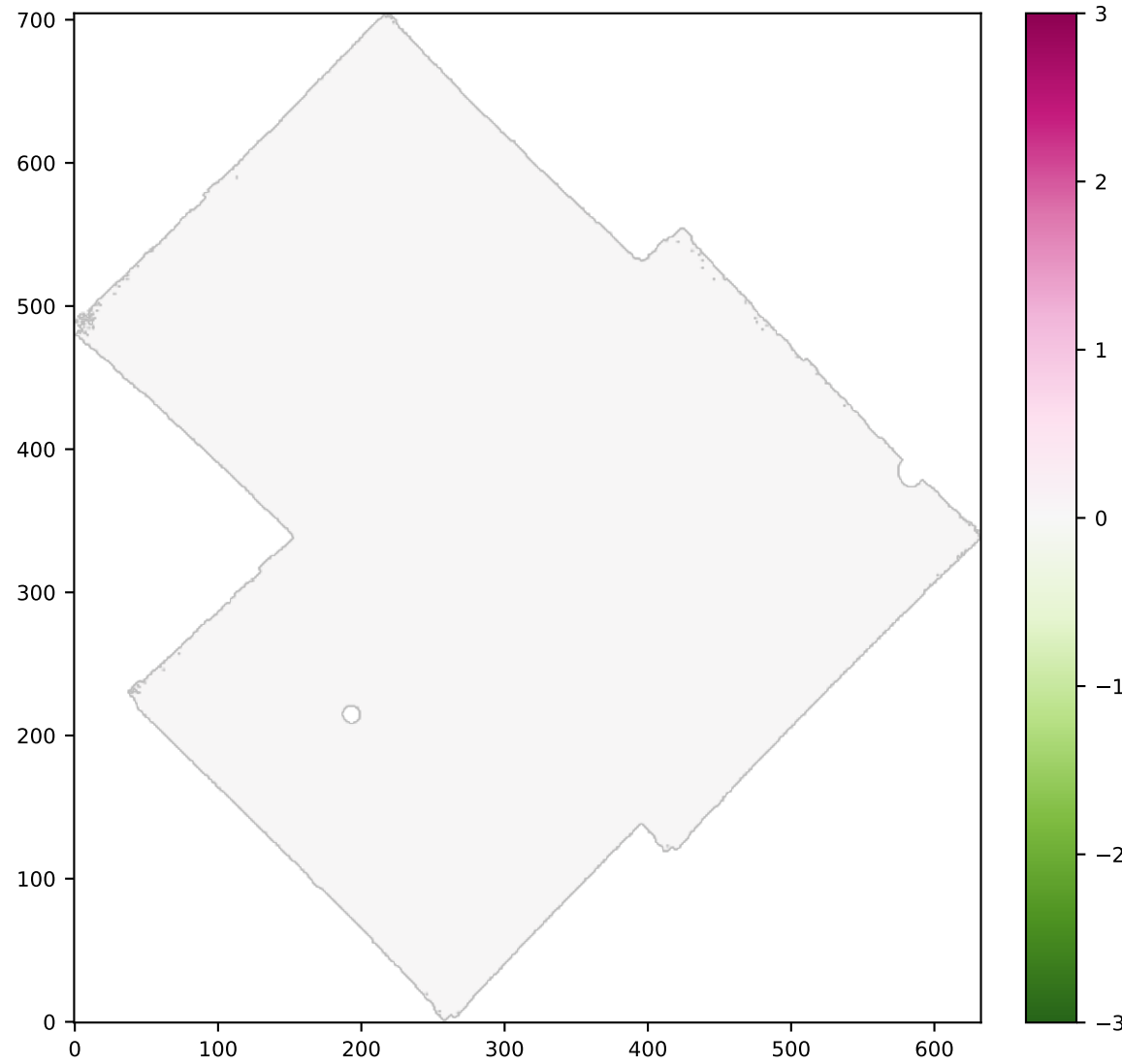
SPAXELS Ha-Hb vel
