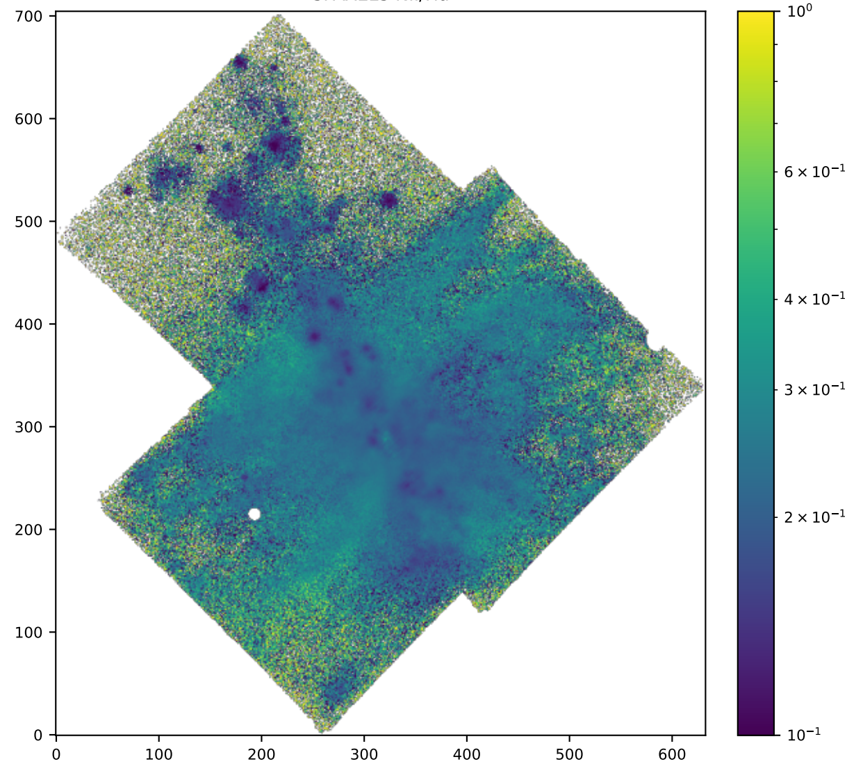
SPAXELS Ha/Hb sigma
