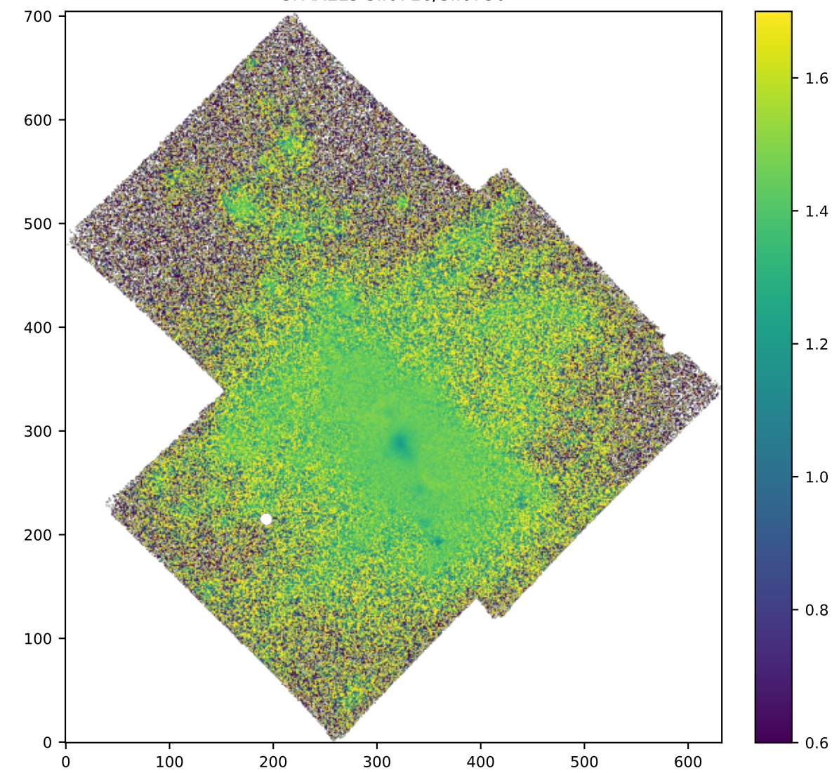
SPAXELS SII6716/SII6730
