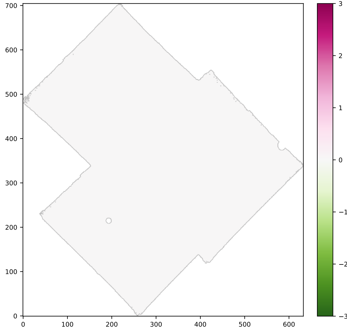
BIN Ha-Hb vel
