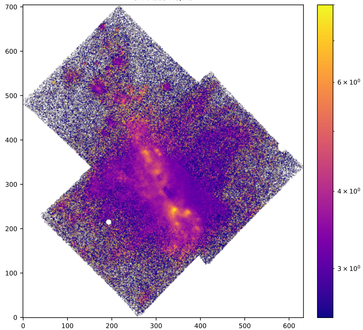
SPAXELS Ha-Hb vel
