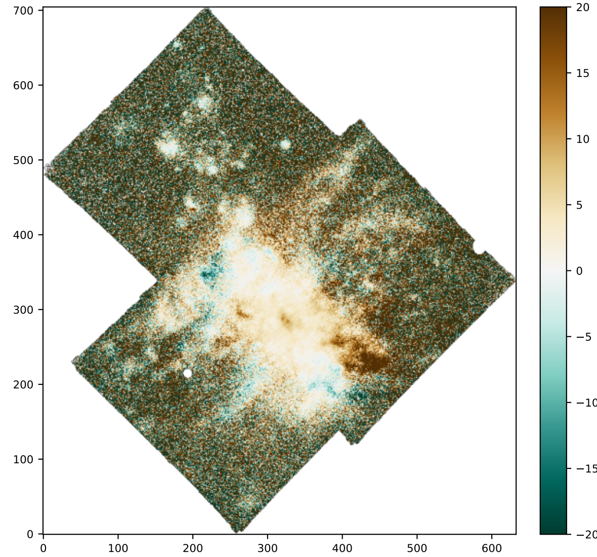
SPAXELS SHa-SNII
