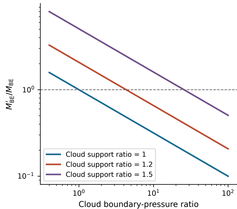
Pressure-confined cloud threshold
