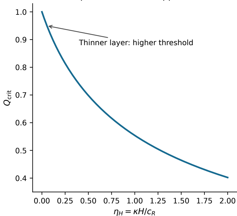
Frozen-profile thickness approximation
