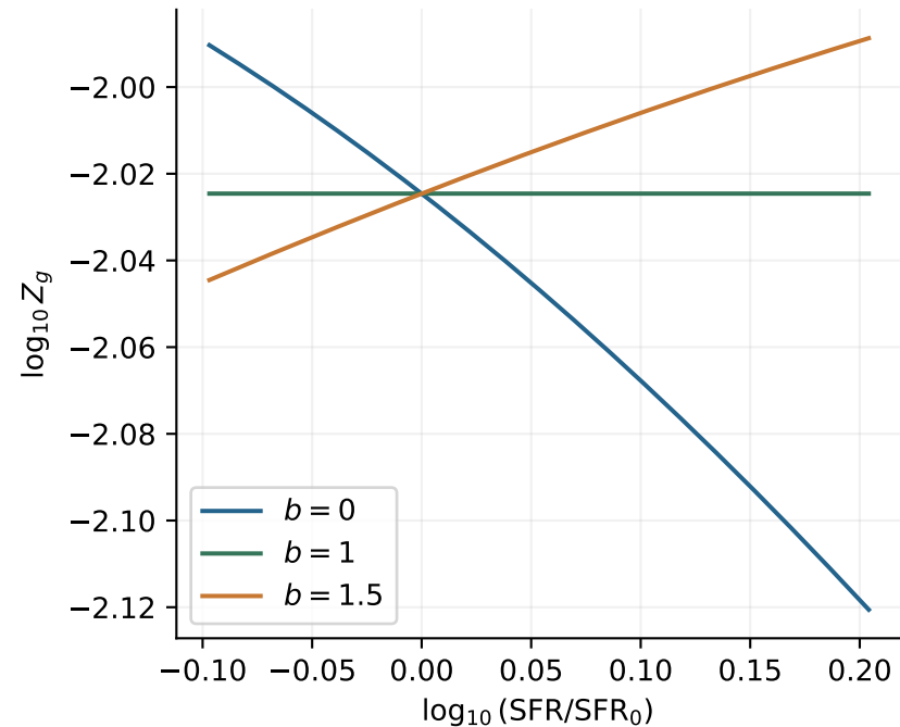
Exact fixed-mass families: M_{\star} = 10^{10.7} M_{\odot} , \eta = 0.44
