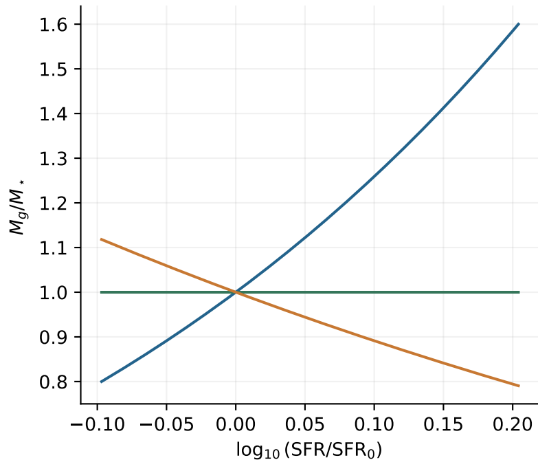
Exact fixed-mass families: M_{\star} = 10^{10.7} M_{\odot} , \eta = 0.44
