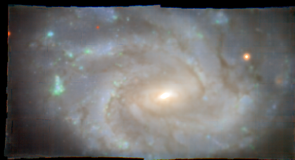
NGC4189
