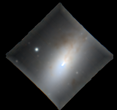
NGC4694
