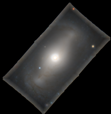
NGC4394
