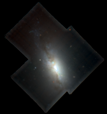
NGC4383
