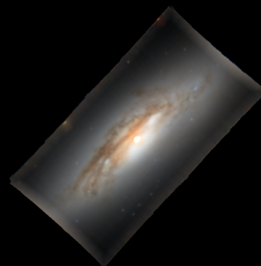
NGC4419
