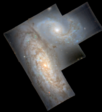
NGC4567 / NGC4568
