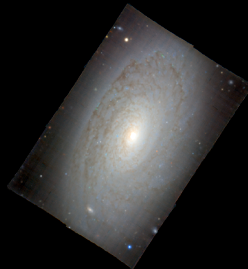
NGC4380
