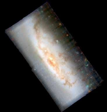
NGC4522
