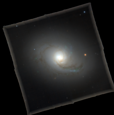
NGC4457
