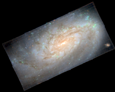
NGC4654
