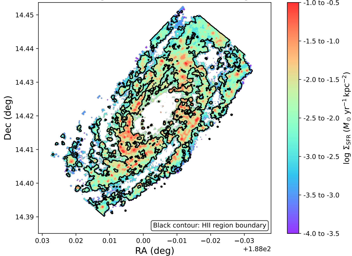
NGC4501: \log \Sigma_{\text{SFR}} (Discrete Bins - SF regions)
