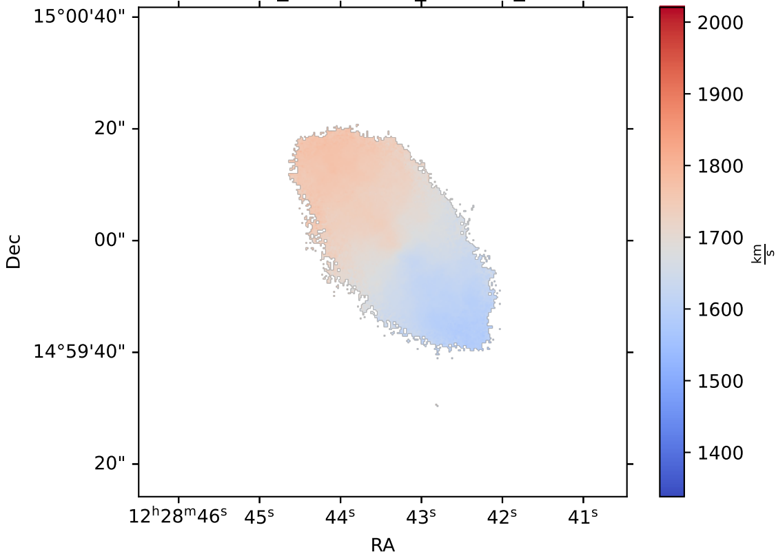
IC3392_multithresh_HA6562_VEL
