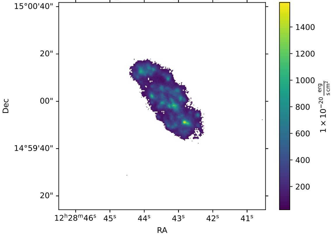
IC3392_multithresh_HB4861_FLUX
