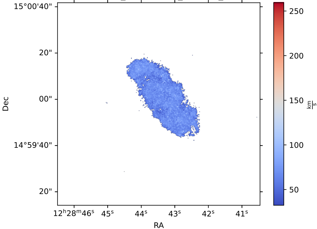
IC3392_multithresh_Hb4861_S
