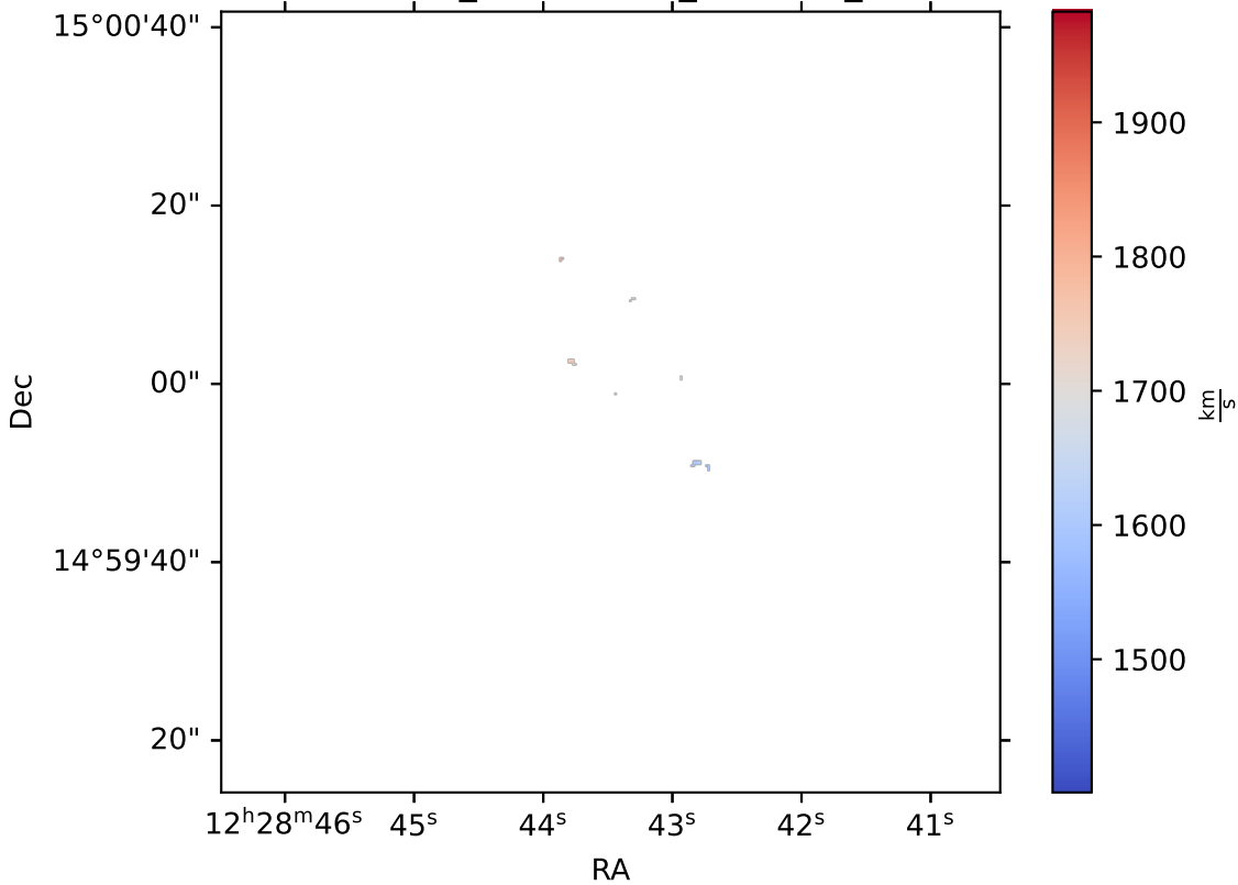
IC3392_multithresh_HeI5875_V
