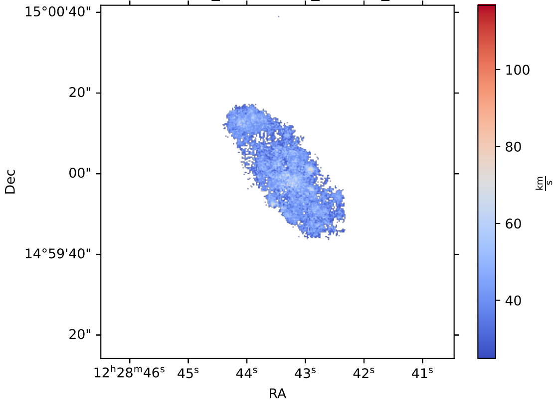
IC3392_multithresh_NII6548_S
