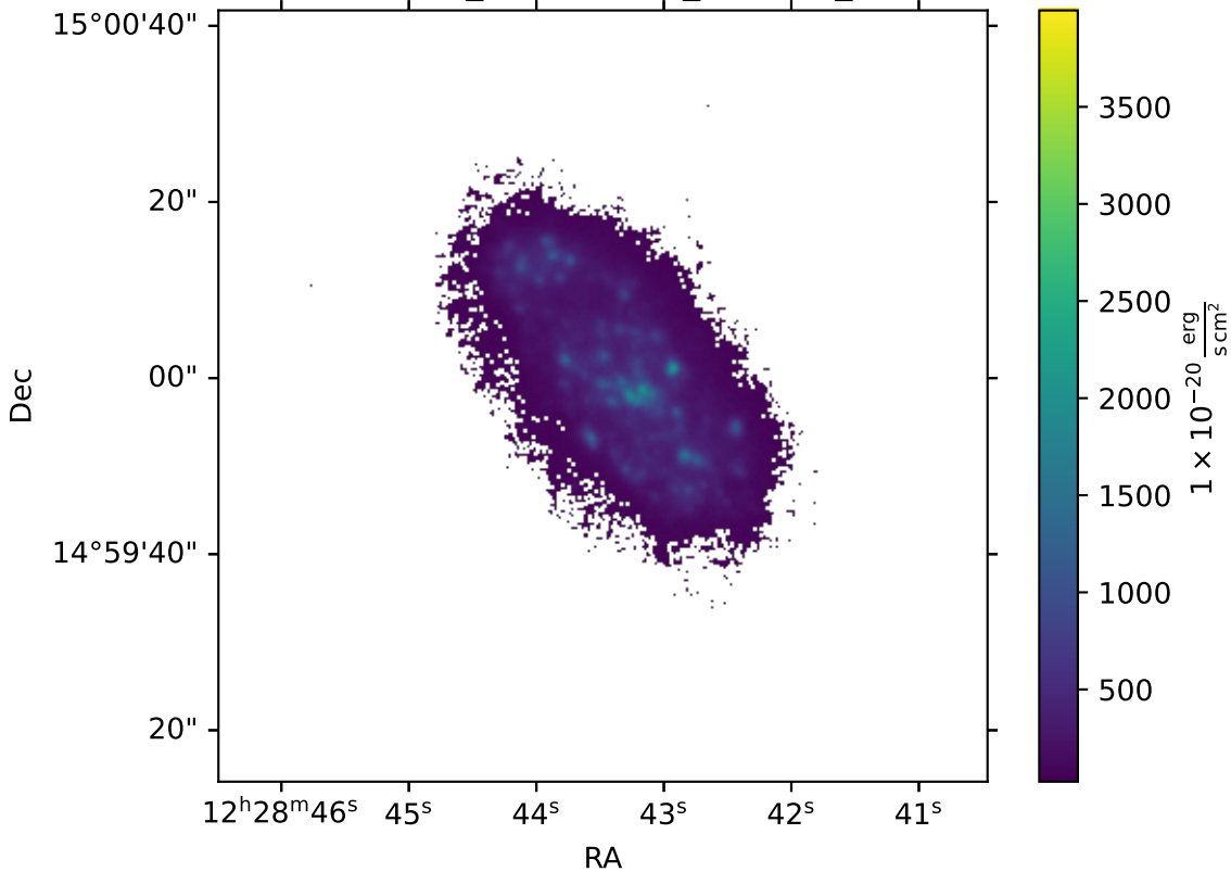
IC3392_multithresh_NII6583_I
