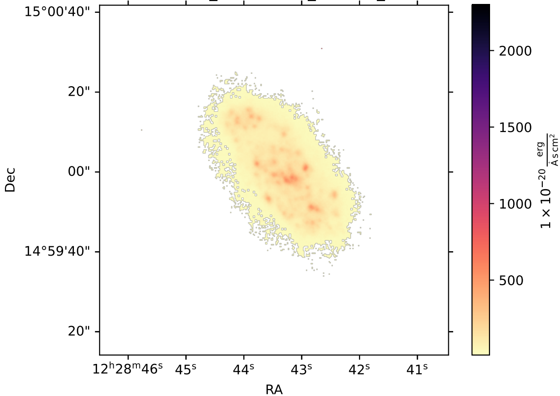
IC3392_multithresh_NII6583_P
