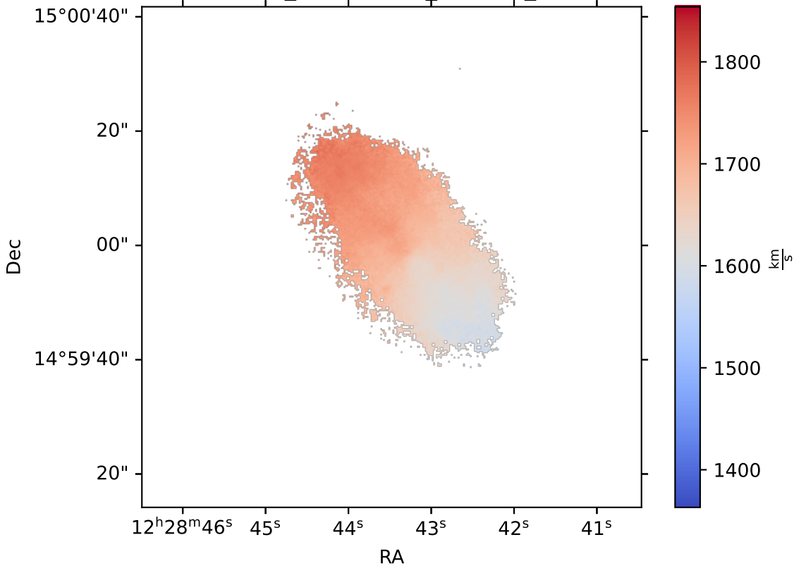
IC3392_multithresh_NII6583_VEL
