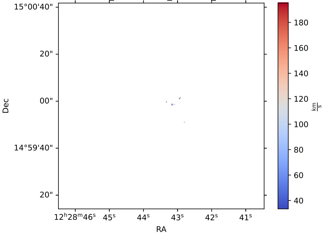
IC3392_multithresh_OIII4958_SIGMA
