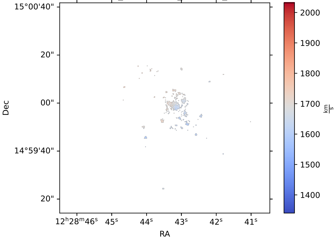
IC3392_multithresh_OIII5006_VEL
