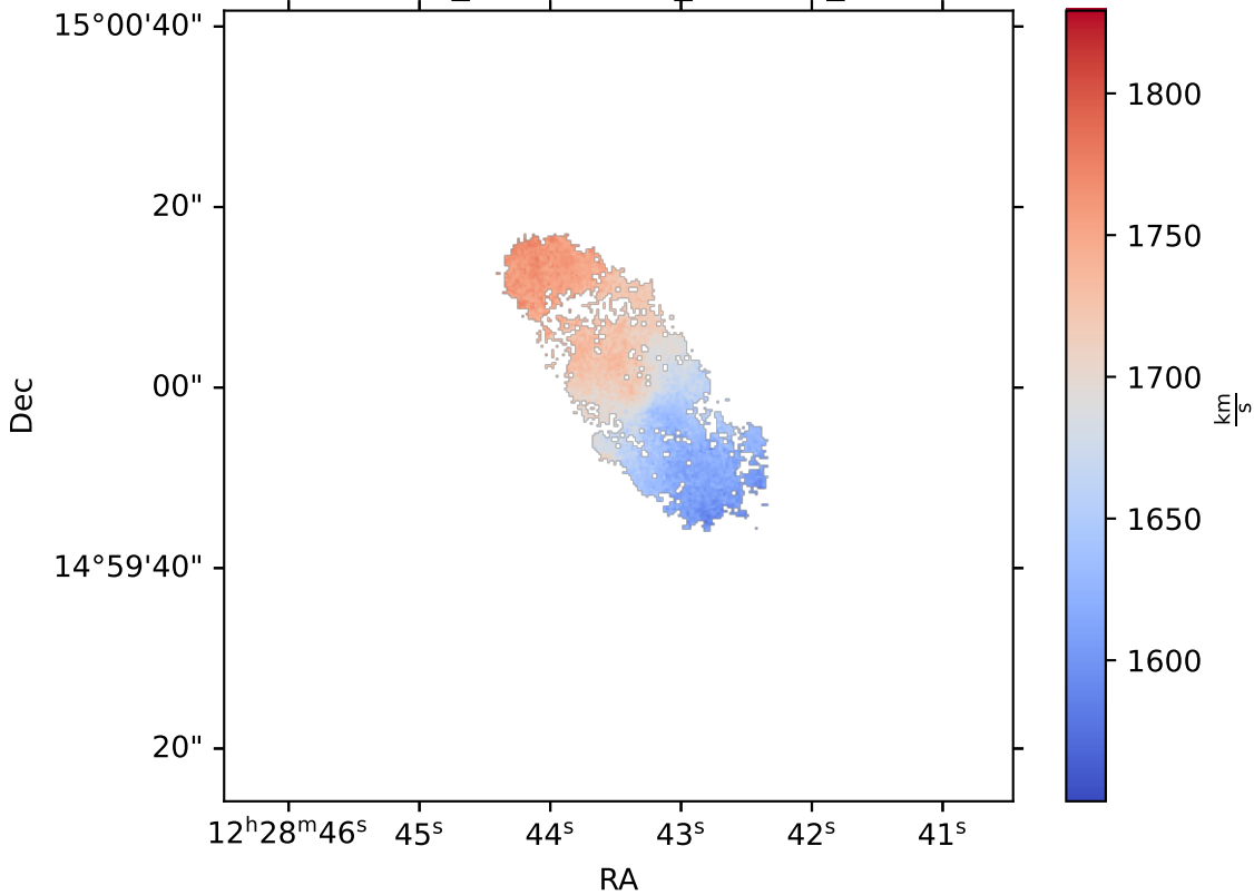
IC3392_multithresh_SII6730_VEL
