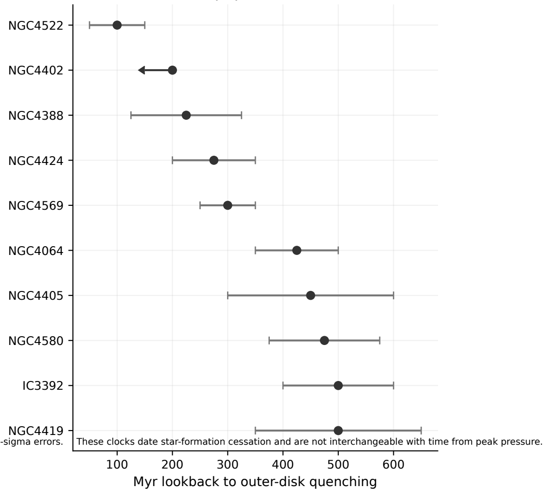
Stellar-population clocks
