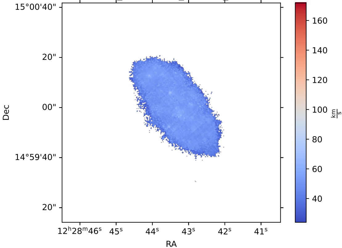
IC3392_multithresh_HA6562_SIGMA
