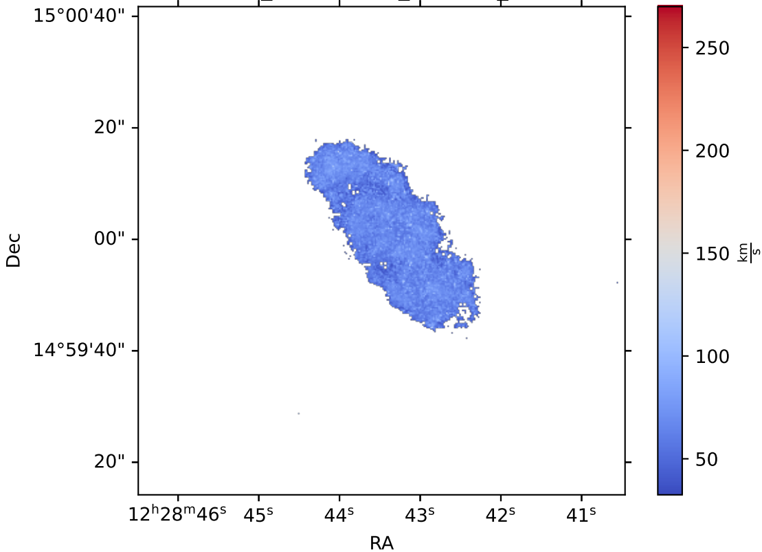
IC3392_multithresh_HB4861_SIGMA
