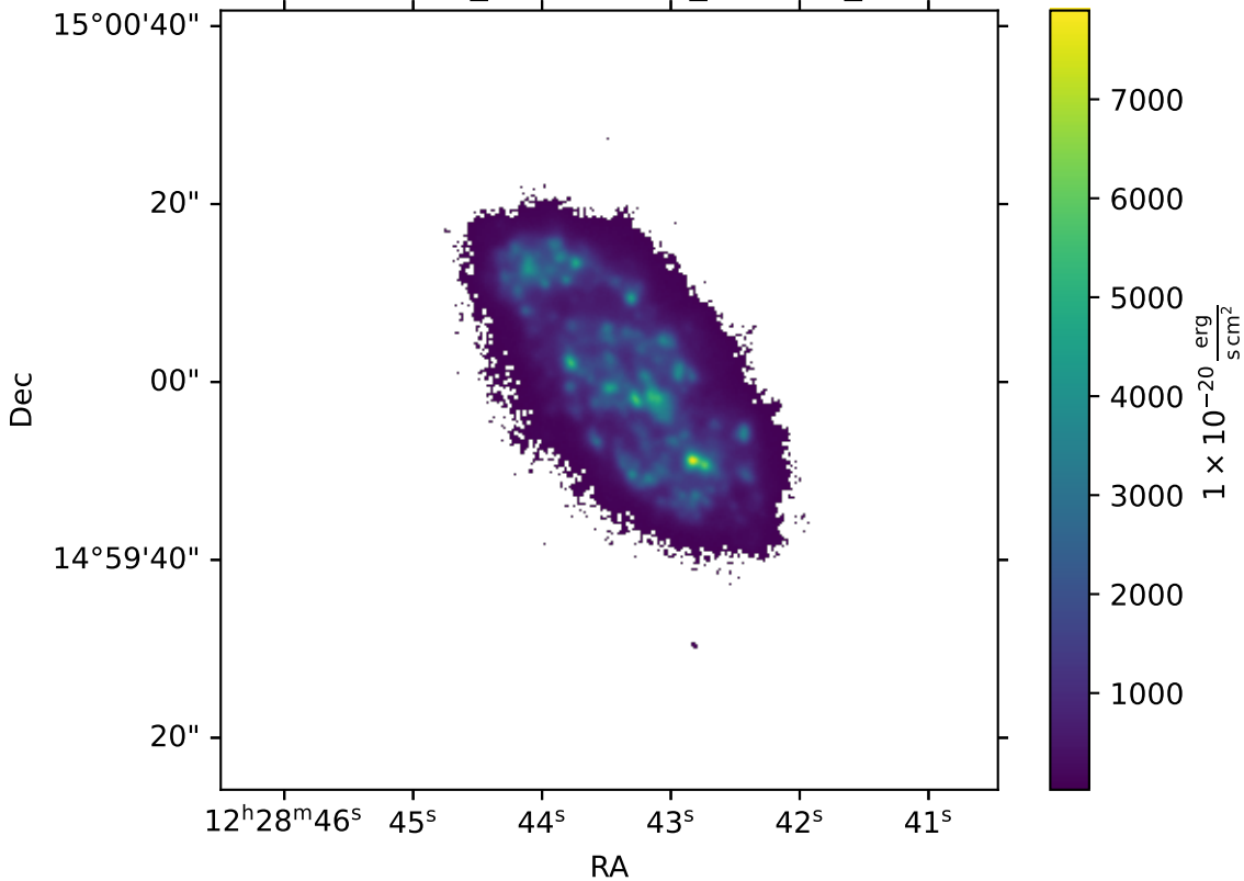
IC3392_multithresh_Ha6562_I
