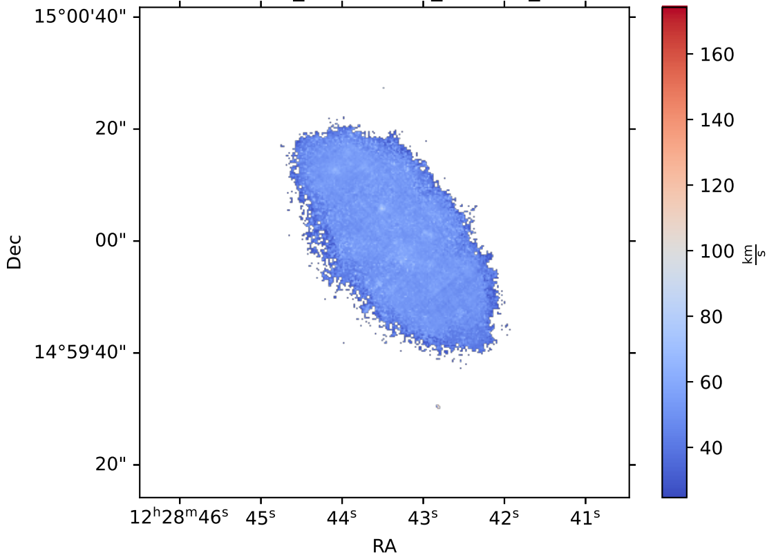
IC3392_multithresh_Ha6562_S
