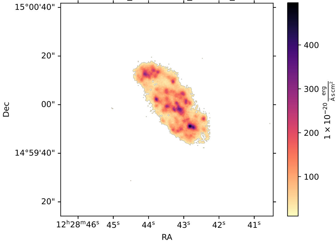
IC3392_multithresh_Hb4861_P
