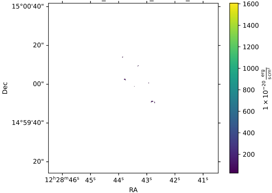
IC3392_multithresh_HeI5875_I
