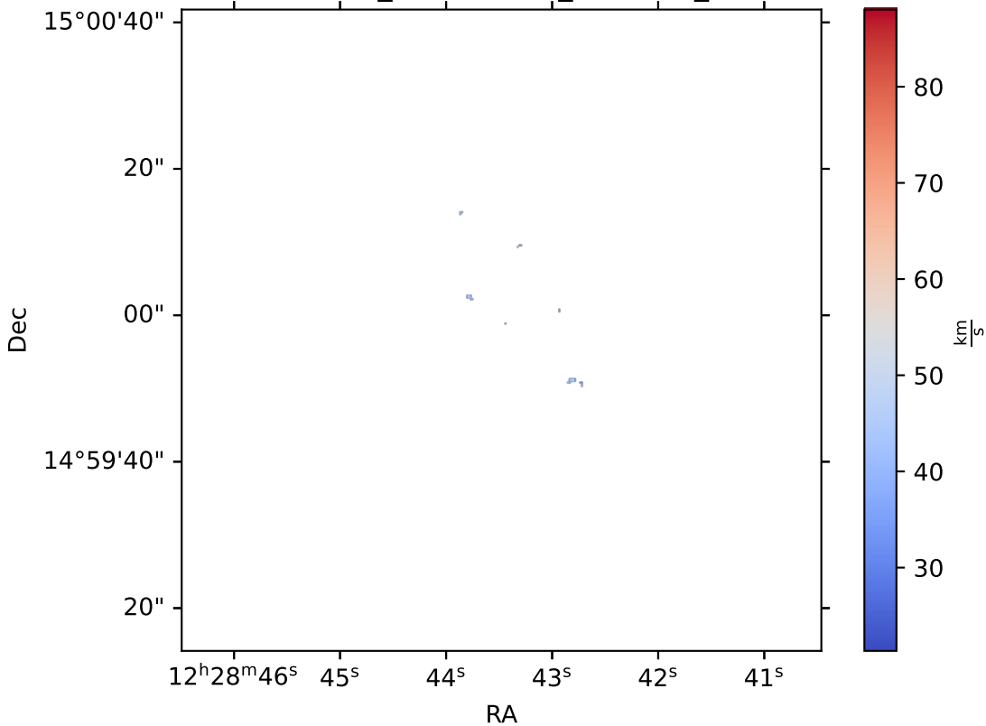
IC3392_multithresh_Hel5875_S
