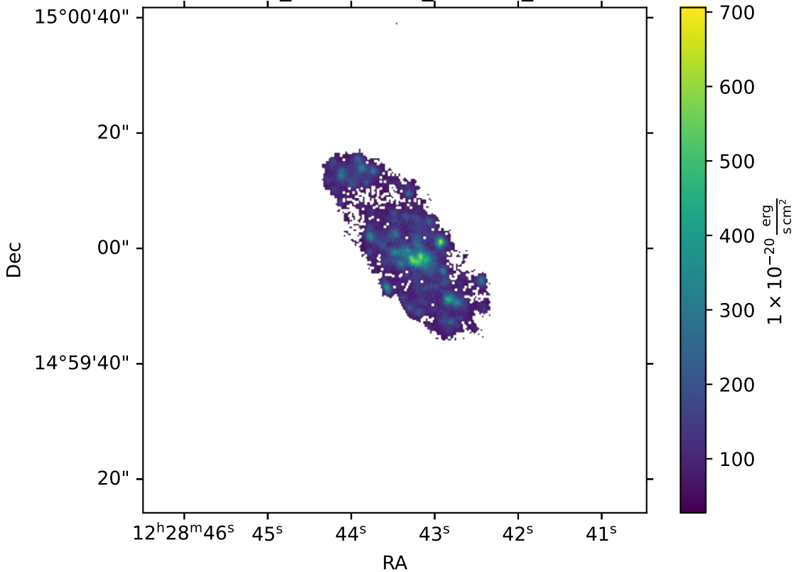
IC3392_multithresh_NII6548_FLUX
