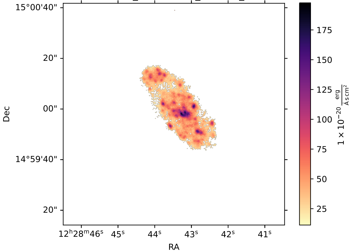
IC3392_multithresh_NII6548_P
