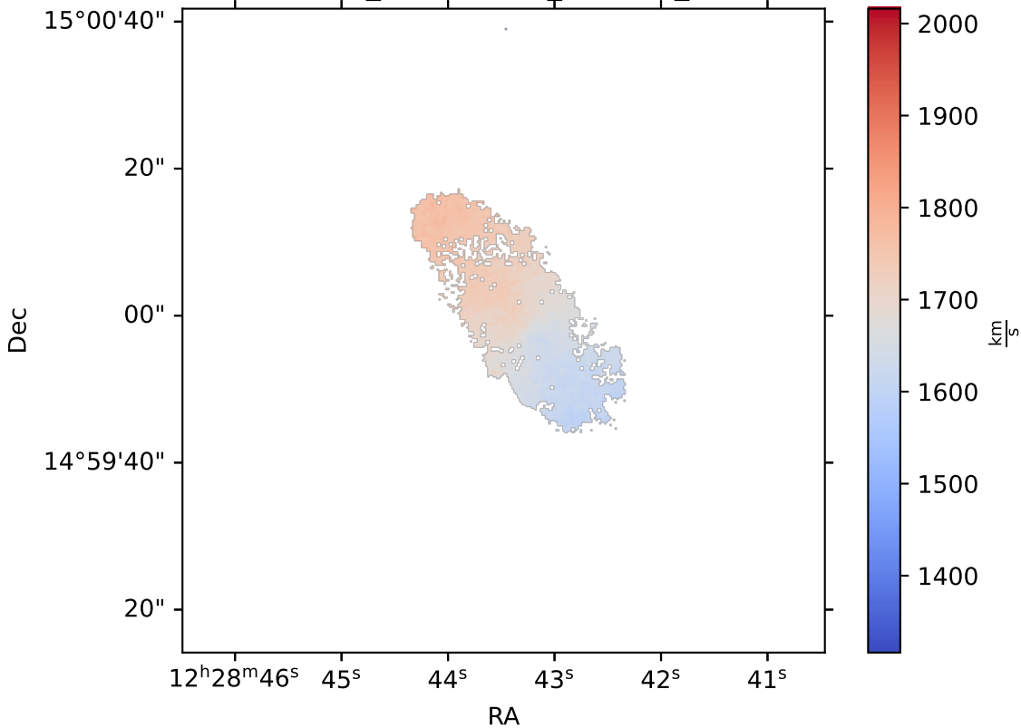
IC3392_multithresh_NII6548_VEL
