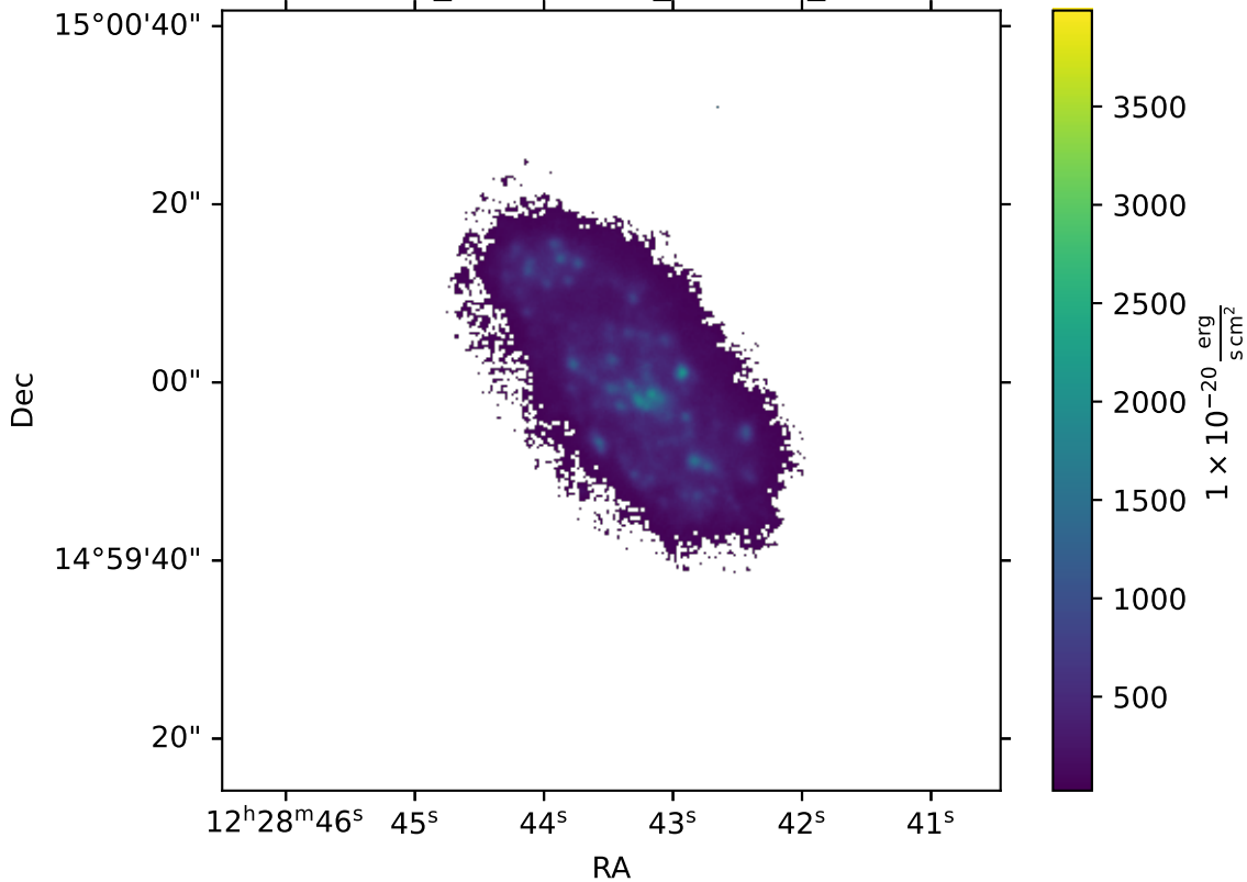
IC3392_multithresh_NII6583_FLUX
