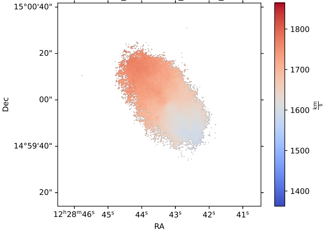
IC3392_multithresh_NII6583_V
